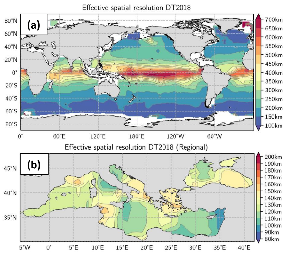
Figure 2: Effective spatial resolution in km of the DUACS-DT2018 maps for a) the Global Ocean product, b) the Mediterranean Sea and the Black Sea products. Unit in km
