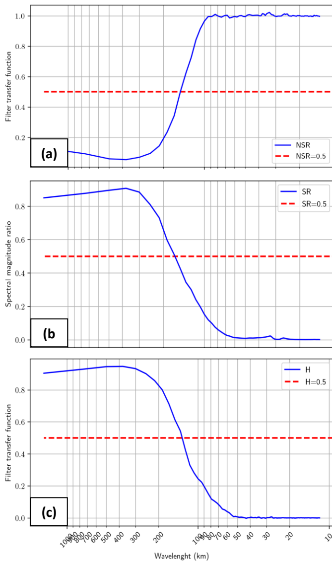
Figure A5: Illustration of the various spectral function used to estimate the resolution a 330°E, 45°N: a) with NSR method, b) with SR method, and c) with the transfer function
