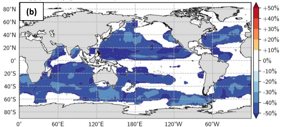
Figure B3: Ratio effective resolution computed with a) SNR=2 versus SNR=4 criterion and b) SNR=2 versus SNR=10 criterion. Blue means finer resolution with SNR=2
