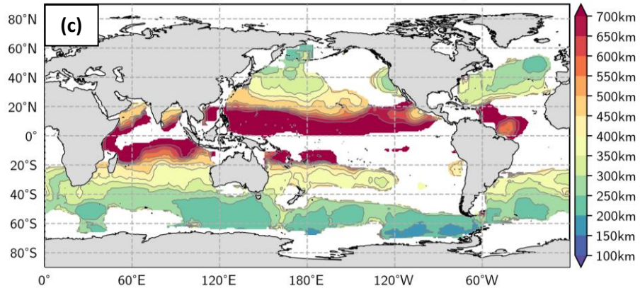
Figure B1: Effective resolution computed for three different SNR criteria: a) SNR=2, b) SNR=4 and c) SNR=10
