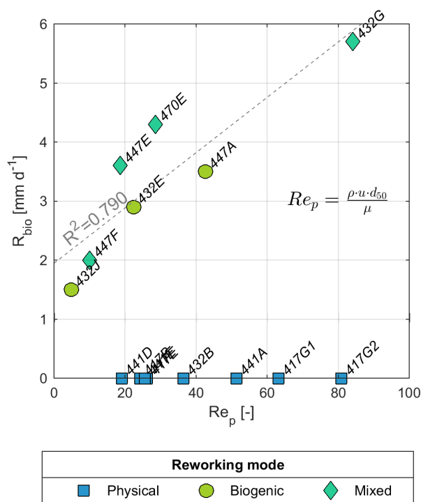
Fig. 1. Correlation of the overturning rates with the particle Reynolds number.
