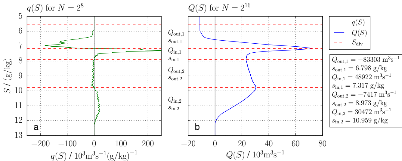
Figure 9. Cross section through Gotland Basin: profiles of q for N = 2^8 = 256 , a), and Q for N = 2^{16} = 65536 , b), for the Gotland transect in 2002/2003. Five dividing salinities separate two inflows and two outflows. The corresponding TEF bulk values are listed on the right.
