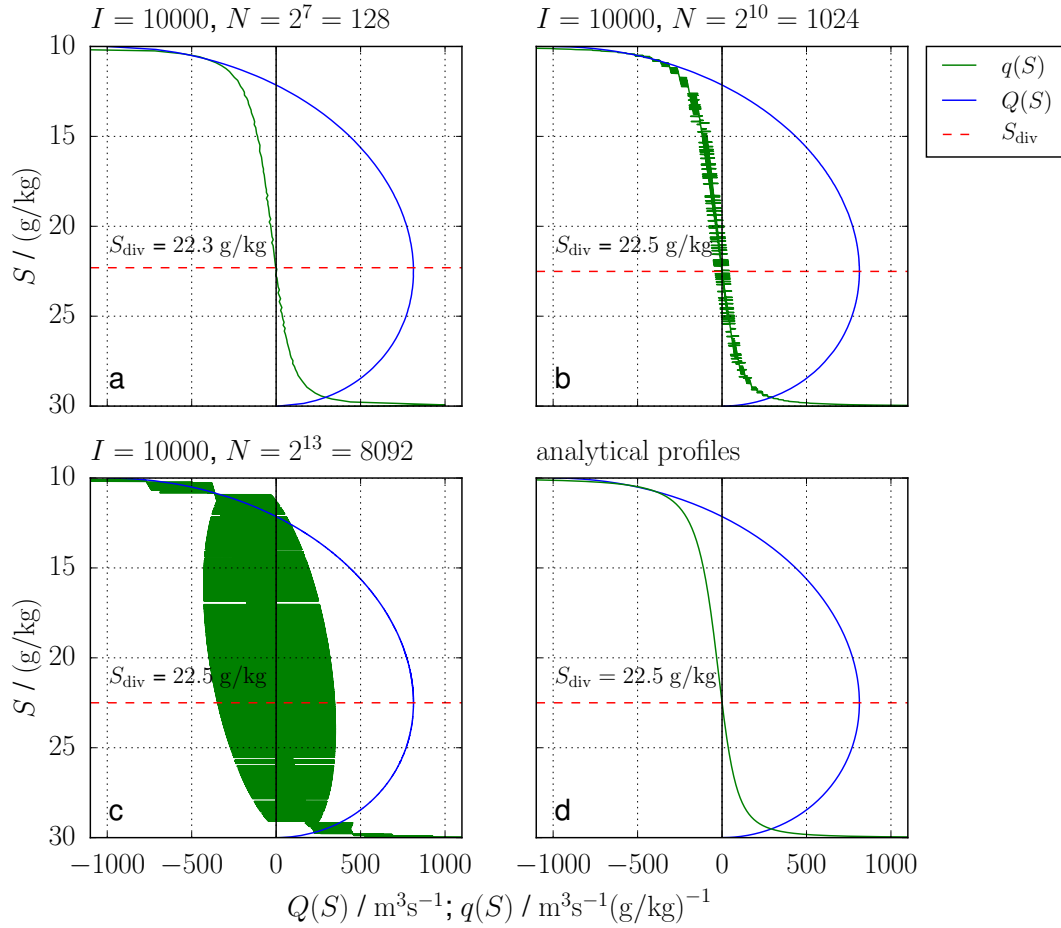
Figure 2. Oscillating exchange flow (see Section 2): from (14) and (15) numerically, a)-c), and analytically, d), found Q(S) (blue), q(S) (green), dividing salinity, S_{\text{div}} (dashed, red), for I = 10^4 time steps for one tidal cycle and varying number of salinity classes N . With increasing N q becomes more noisy, whereas Q seems unchanged.
