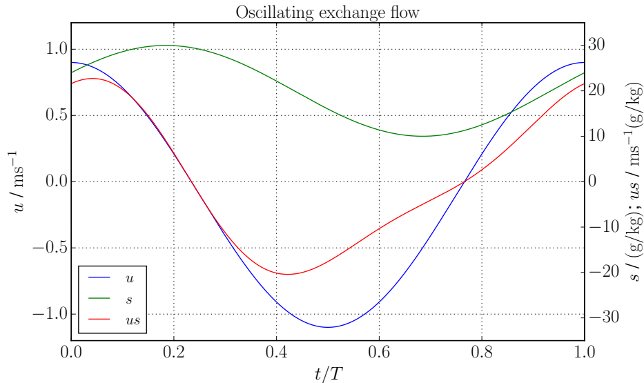
Figure 1. Oscillating exchange flow (see Section 2): time series of velocity (blue), salinity (green) and salinity flux (red) for the oscillating exchange flow scenario (8).
