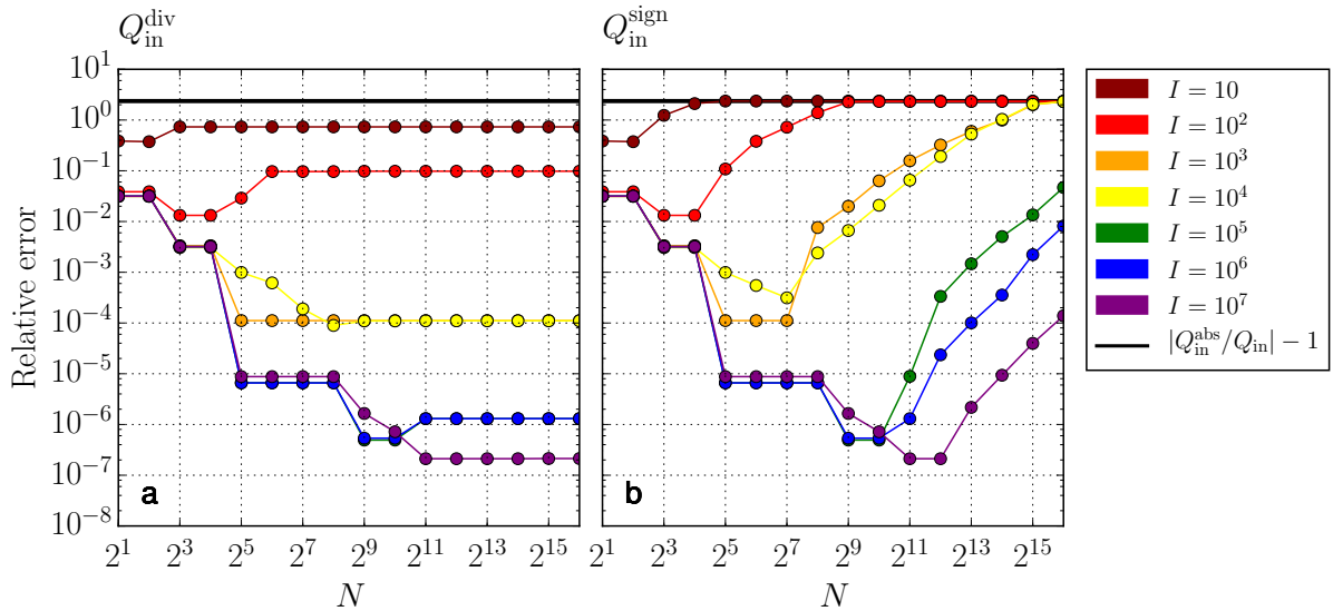
Figure 3. Oscillating exchange flow (see Section 2): relative error of Q_{in} computed with a) the dividing salinity method and b) the sign method in dependency of the number of time steps I (color) and salinity classes N . The sign method, (5) and the dividing salinity method, (7) coincide for a small number of salinity classes, but the error of the sign method converges in the limit of large N towards the error of the absolute bulk values (black line, (6)). In contrast, the error of the dividing salinity method converges towards a constant value. The errors of both methods decrease with increasing number of time steps I .
