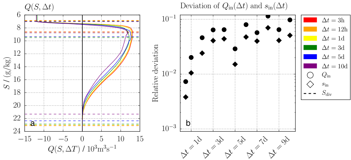
Figure 8. Exchange flow over Darss Sill: comparison of Q(S) ( N = 2^{16} = 65536 ) for different \Delta t in a) and the relative deviations of Q_{\text{in}} and s_{\text{in}} in dependency \Delta t to the bulk values for \Delta t = 3\text{h} . The bulk values were computed from Q(\Delta t) using the extended dividing salinity method (11),(16). The dashed lines in a) show the dividing salinities used to compute the bulk values in b). With different temporal resolutions the shape of Q(S) changes considerably and the resulting bulk values deviate significantly from the ones for 3-hourly data.
