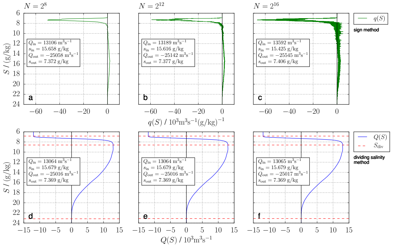
Figure 7. Exchange flow over Darss Sill: profiles of q (upper panels) and Q (lower panels) for the Darss Sill transect in 2002/2003 in dependency of the number of salinity classes N , a) and d) N = 2^8 = 256 , b) and e) N = 2^{12} = 4096 , c) and f) N = 2^{16} = 65536 . The respective TEF bulk values are calculated with the sign method (5) in the upper panels and the extended dividing salinity method (11), (16) in the lower panels.
