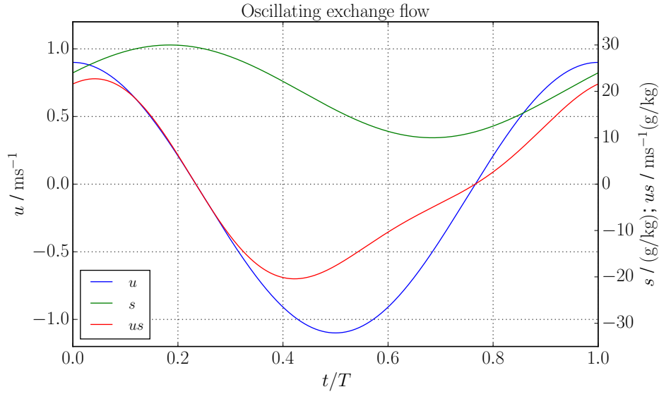
Figure 1. Velocity-Oscillating exchange flow (see Section 2): time series of velocity (blue), salinity (green) and salinity flux (red) time-series for the oscillating exchange flow scenario (8).
