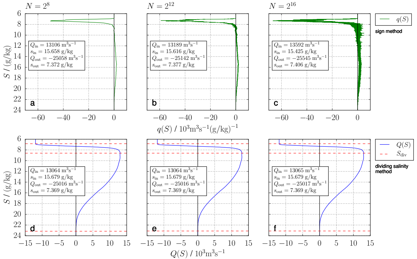
Figure 7. Profiles Exchange flow over Darss Sill: profiles of q (upper panels) and Q (lower panels) for the Darss Sill transect in 2002/2003 in dependency of the number of salinity classes N , a) and d) N = 2^8 = 256 , b) and e) N = 2^{12} = 4096 , c) and f) N = 2^{16} = 65536 . The respective TEF bulk values are calculated with the sign method (5) in the upper panels and the extended dividing salinity method (12), (16) in the lower panels.
