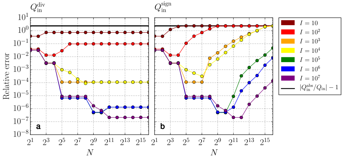
Figure 3. Comparison of the Oscillating exchange flow (see Section 2): relative error of numerically-calculated bulk values to the analytical values, Q_{in} computed with a) Q_{in}^{div} the dividing salinity method and b) Q_{in}^{sign} the sign method in dependency of the number of time steps I (color) and salinity classes N . The sign method (dots), (5) (MacCready, 2011) and the dividing salinity method (stars), (7) (MacCready et al., 2018) coincide for a small number of salinity classes, but the error of the sign method converges in the limit of large N towards the error of the absolute bulk values (black line), defined in (26). In contrast, the error of the dividing salinity method converges towards a constant value. The errors of both methods decrease with increasing number of time steps I .
