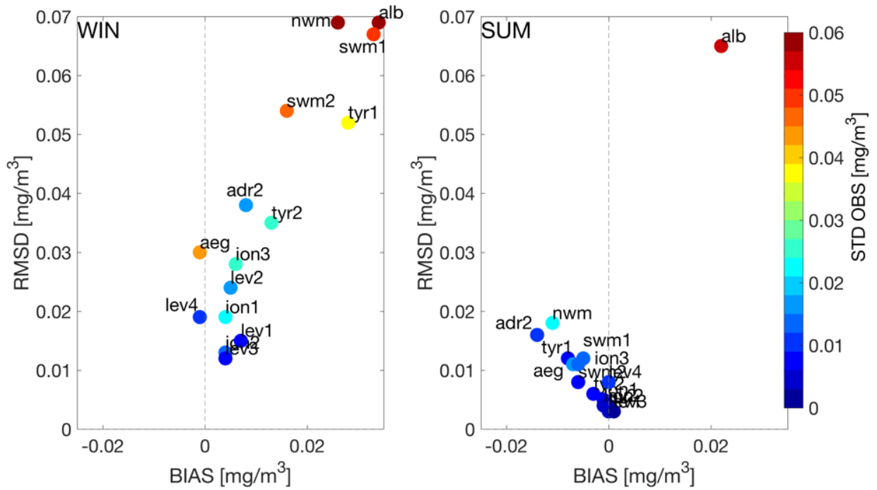
5 Figure 8: Target diagrams of the model and satellite chlorophyll comparison and standard deviation of observations (in colour shading) for two periods: January to April (WIN, left) and June to September (SUM, right). For sake of readability, an offset in the values in WIN of [RMSD, BIAS] for ALB and of [RMSD] for NWM (respectively equal to [0.17, 0.09] mg/m 3 , and [0.1] mg/m 3 ) has been applied to include the dots within the plot.
