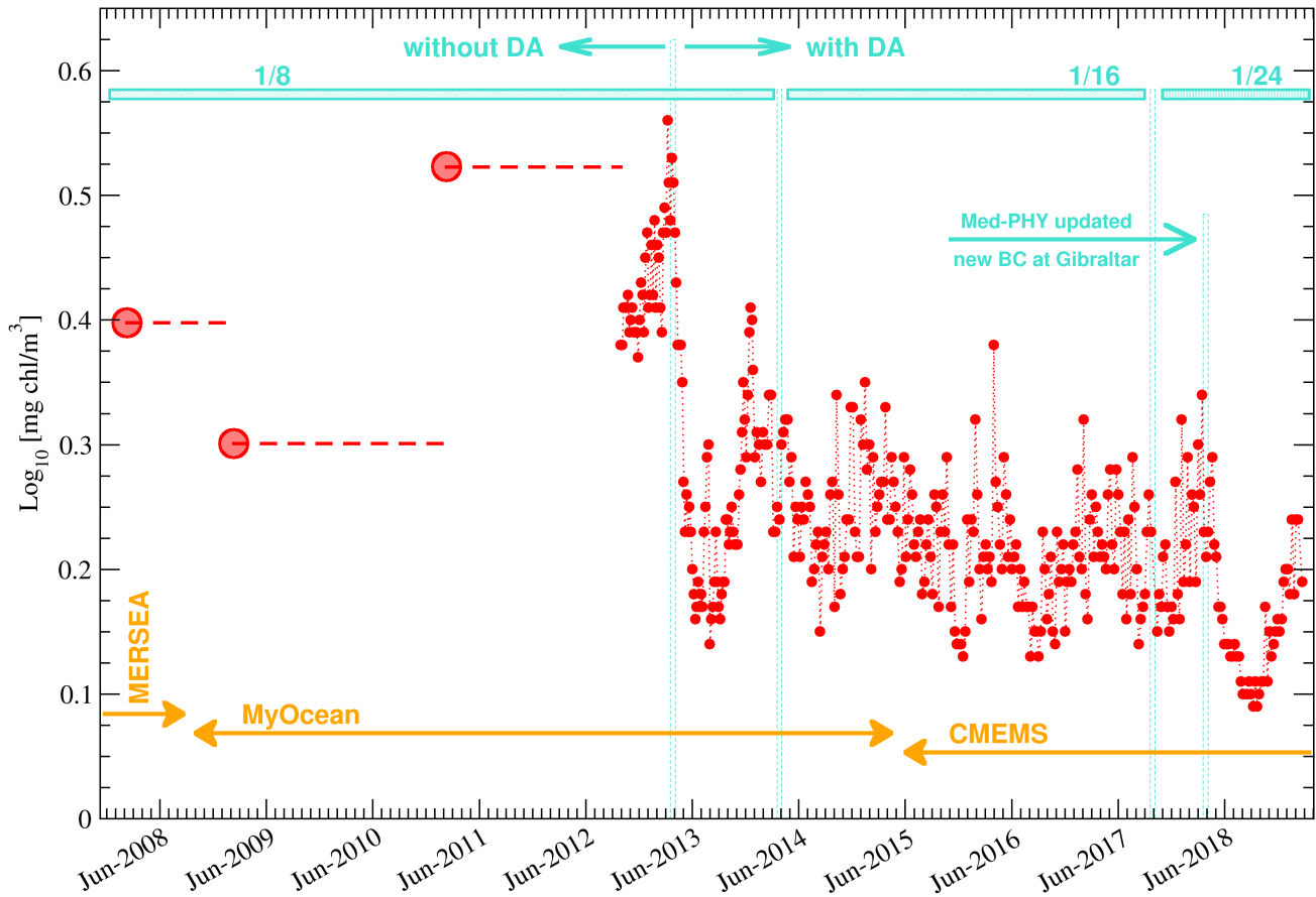
5 Figure 14: RMSD of the surface chlorophyll concentration with satellite data. The use of logarithmic units has been the standard for RMSD since the implementation phase. Regular, weekly product quality assessment (red dots and dotted line) started at the end of 2012. Before, quality assessment was performed only occasionally for specific periods (e.g. Teruzzi et al., 2011; Tonani et al., 2012; large red dots) and thick red lines). In the plot, we identify the different projects (yellow), the start of data assimilation (April 2013), and the increase of horizontal resolution (cyan).
