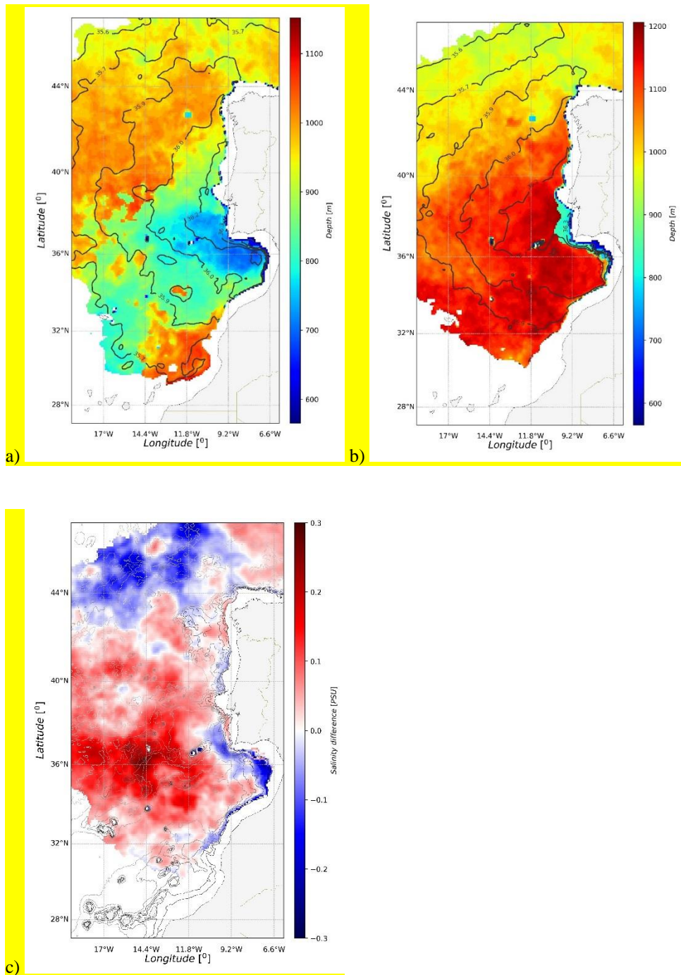
5 Figure 9: (a and b) Maximum salinity depth (shaded colours) between 500 and 1500 m and salinity (isolines) at the maximum salinity depth. Maps obtained from the composites of minimum (a) and maximum (b) salinity defined by 10 th and 90 th percentiles of salinity anomalies in Horseshoes Basin respectively. (c) Difference of salinity between panels a and b, contour lines represent bathymetry.
