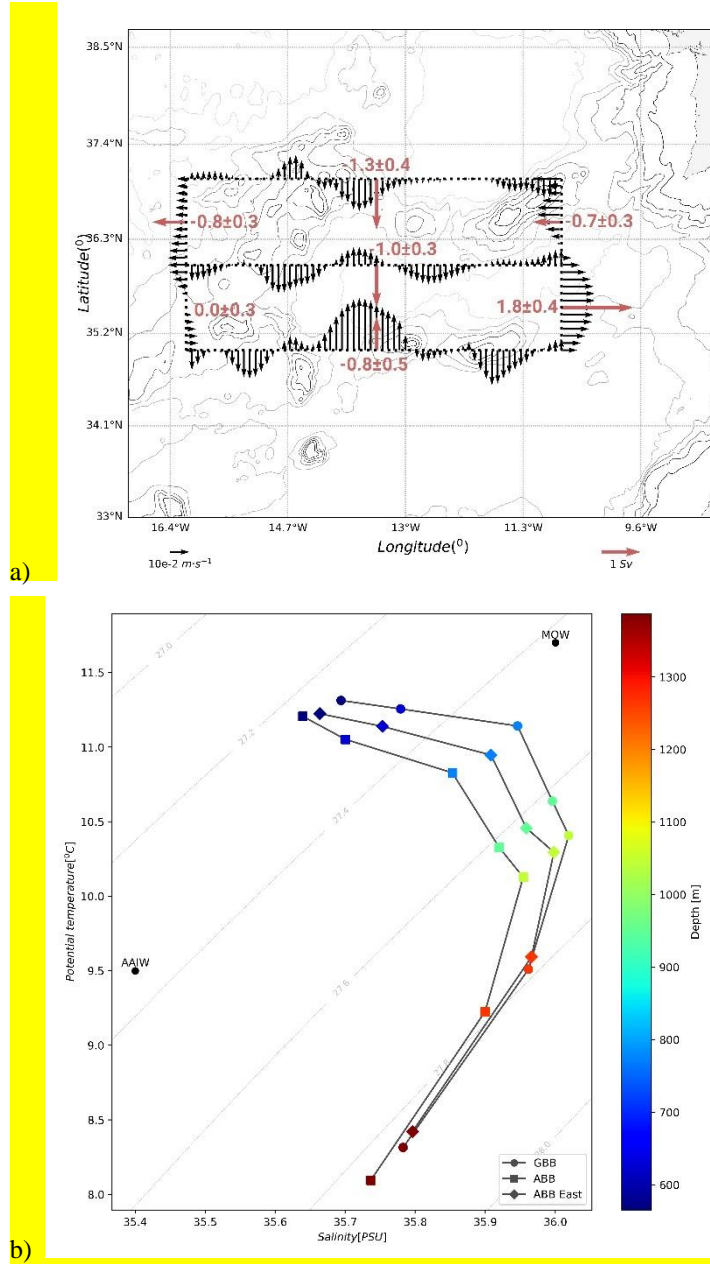
5 Figure 4: (a) Transverse velocity (black arrows) and net volume transport (red arrows) in sections delimiting GBB and ABB. (b) Mean \theta/S diagram averaged in GBB (circles), ABB (squares) and along the section marking the Eastern-ABB boundary (diamonds). Dotted isolines correspond to potential density anomaly in \text{Kg/m}^3 . Black dots represent the position of the source water types AAIW and MQW.
