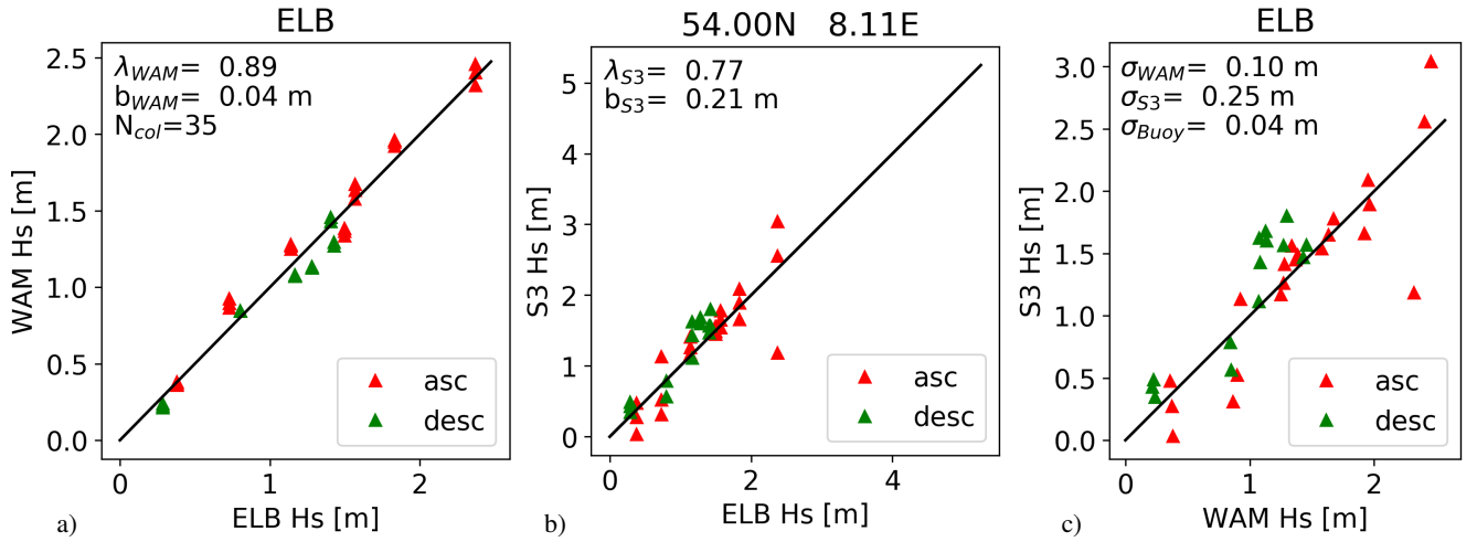
Figure 5. (a,b) Comparison of wave heights measured by the Elbe buoy with numerical model results (a), and SENTINEL-3a altimeter measurements (b). The model and satellite data sets were corrected according to the calibration factors \lambda_{WAM} , \lambda_{S3} and bias parameters b_{WAM} , b_{S3} estimated in the triple collocation procedure (see eq. 21). (c): Direct comparison between model and satellite data. Numbers are given for the estimated calibration factors, bias, and stochastic error standard deviations \epsilon_{WAM} , \epsilon_{S3} , \epsilon_{Buoy} . The red triangles refer to ascending satellite passes and the green ones to descending passes.
