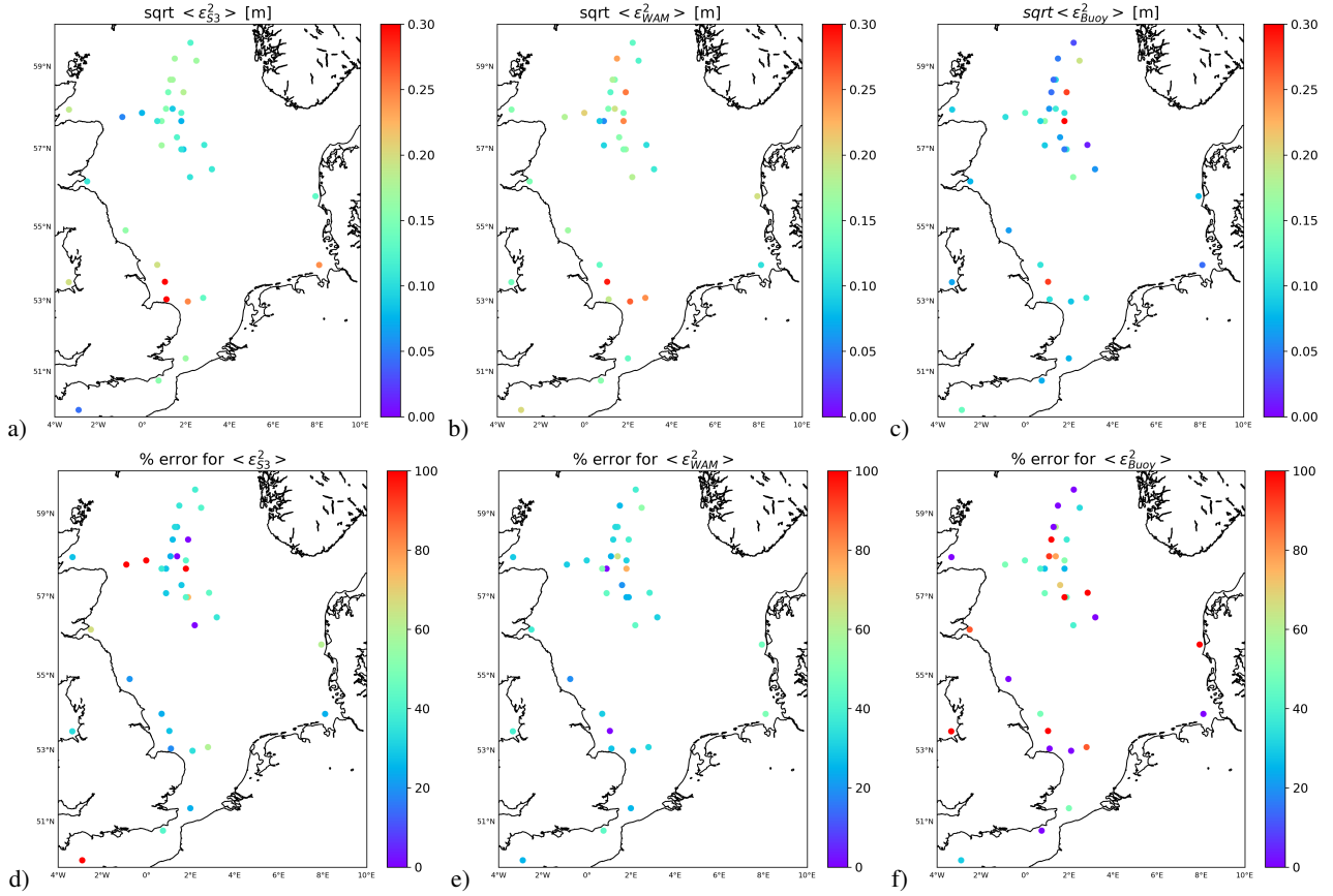
Figure 7. (a,b,c): Colour coded stochastic error standard deviations of wave heights provided by the SENTINEL-3a altimeter (a), the WAM model (b), and the insitu stations (c) estimated by triple collocation . (d,e,f): Relative uncertainties of the stochastic error estimates, derived by using the approach in Section 2.1.
