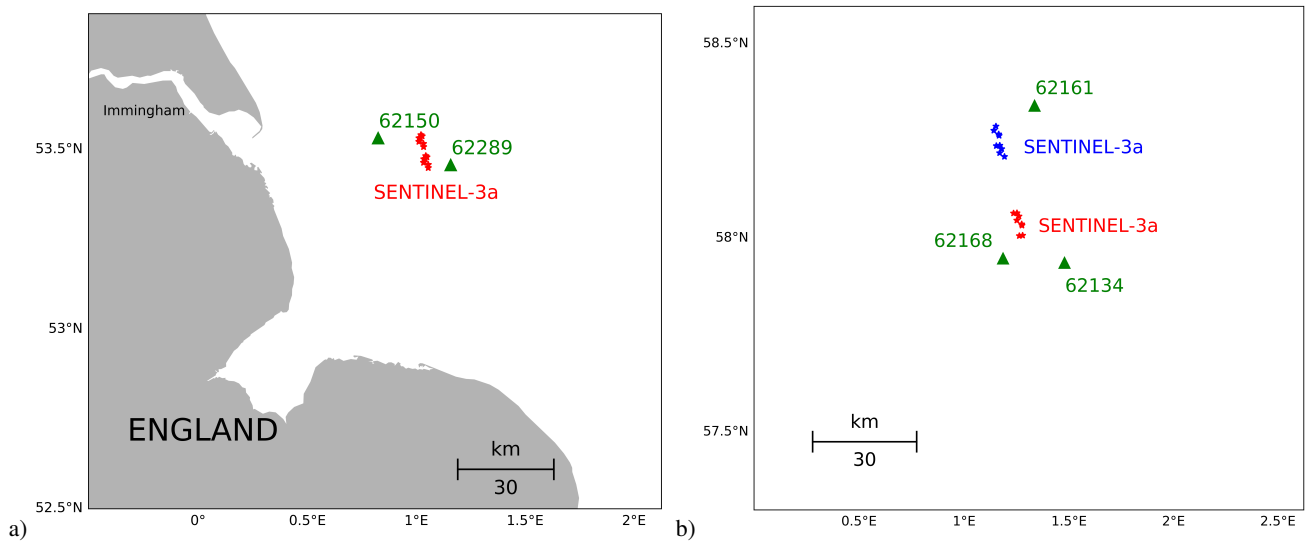
Figure 8. (a): Example of observation configuration with a descending SENTINEL-3a altimeter track passing between two insitu wave observation instruments ("62150" and "62289"), (b): Observation geometry with SENTINEL-3a track passing through a group of three insitu wave measurement devices. The blue and red altimeter measurements are used to estimate error correlations for both the altimeter and the numerical model.
