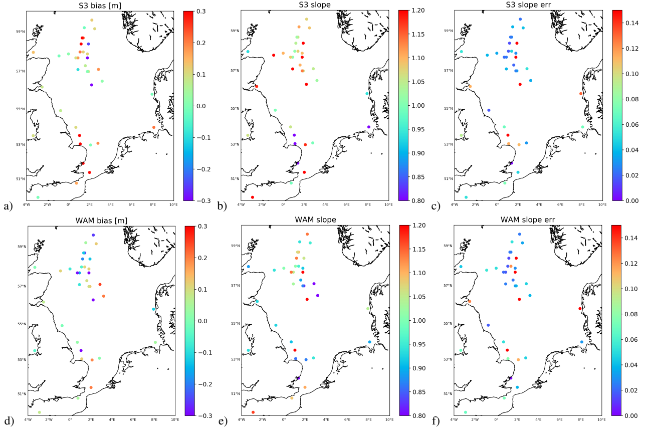
Figure 6. Colour coded biases (a,d) and calibration factors (b,e) derived by triple collocation for the SENTINEL-3a altimeter (top) and WAM model wave heights (bottom). The right column (c,f) gives the uncertainties of the slope estimations derived using the approach in Section 2.2 as standard deviation.
