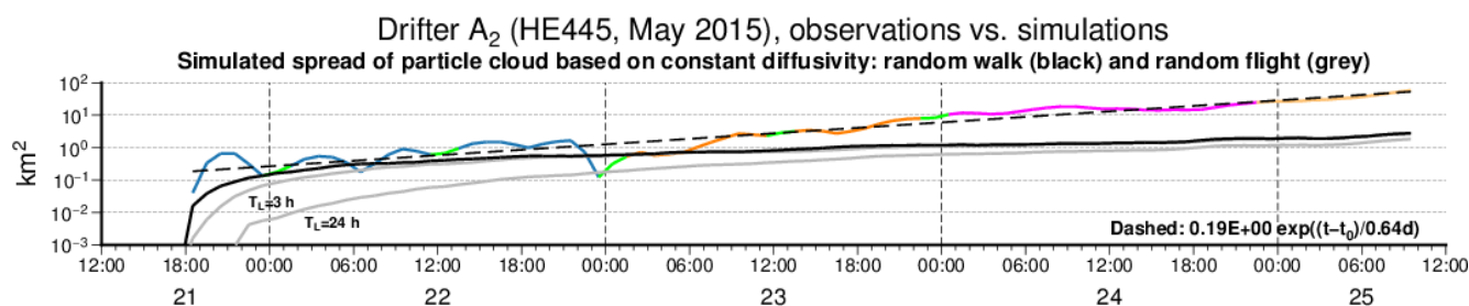
Figure 14. Time evolution of squared separation between observed and simulated trajectories of drifter A_2 . Segmentation using different colours is consistent with that in Fig. 3. The dashed line indicates the fitted exponential growth model annotated in the graph. The solid black line represents relative dispersion D^2 obtained from 100 trajectories initialized at the same location and simulated with random walk model Eq. (10). Grey lines show results when using random flight model Eq. (12) with T_L = 3\text{ h} and T_L = 24\text{ h} , respectively.
