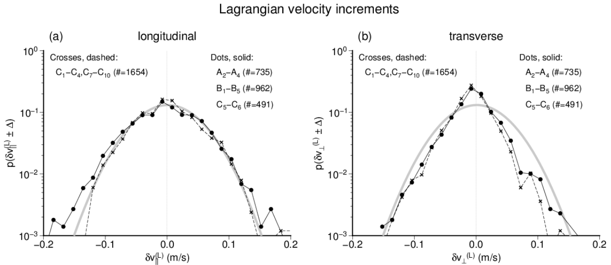
Figure 12. Distributions of (a) longitudinal and (b) transversal components of Lagrangian separation velocities, calculated from binned velocities (bin width 2\Delta=0.016 m/s) based on 20 min time resolution. Solid lines (dots) refer to those drifters that were particularly close to wind farms, dashed lines (crosses) to those that presumably did not experience direct wind farm effects. A normal distribution fitted to the longitudinal data (indicated in grey) was just copied from panel (a) to panel (b) as a reference that facilitates a comparison of distributions of the two velocity components.
