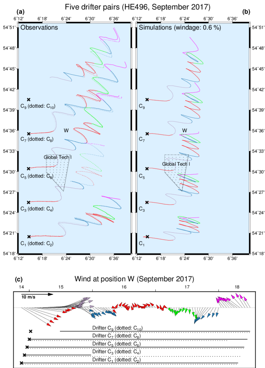
Figure 6. (a) Trajectories of five drifter pairs. (b) Corresponding simulations. (c) Wind conditions during the observational period. Horizontal lines indicate drifter travel times. Different colours are used for a consistent segmentation of the observational period.
