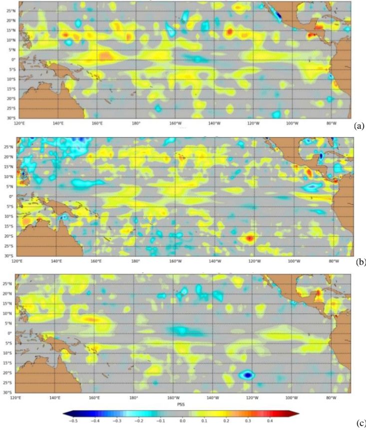
Figure 3: Example of model salinity bias ( x ) near the surface (Eq. 1a) calculated from in-situ data between 0 and 10 m depth only (a), of SSS bias ( \xi ) (Eq. 24b) calculated from in-situ data between 0 and 10 m depth and SMOS SSS (b) and salinity bias ( x ) (Eq. 24a + Eq. 1b) from in-situ data between 0 and 10 m and SMOS SSS (c) in the Tropical Pacific (week 20-27 January 2016).
