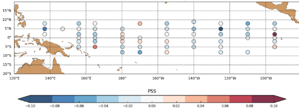
Figure 16. Difference in model salinity RMSE (pss) at 1 m depth calculated against the 1 m depth TAO mooring salinity values (SMOSexp - REF) calculated over the period 1 st Jan 2014 to 16 th March 2016 (negative/positive difference implies a reduction/increase in RMSE by the SMOS assimilation). Moorings are only included if they have more than 1 week of measurements during the period.
