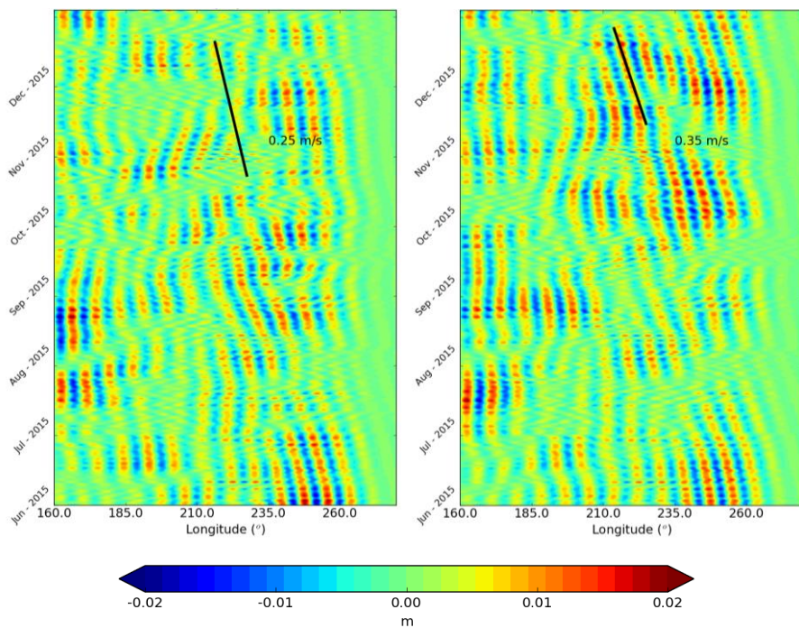
Figure 14: Hovmöller of 28640 day (33 days) band-passed SSH anomalies at 4°N referenced to the temporal annual mean of June-December 2015 for REF experiment (left) and for SMOExp experiment (right). The propagation speeds of 0.25 and 0.35 m/s (solid lines) are representative of the propagation speed for the 28640 day bands.
