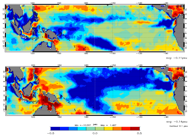
Figure 14: SSS anomalies (psu) in 2014 (top) and 2015 (bottom): mean salinity difference [model (control run) – the World Ocean Atlas (WOA) 2013].
