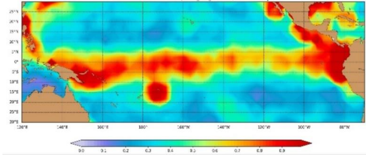
Figure 4: Example of the final product of Desroziers ratio r_{\xi}^5 r_{\xi}^4 r_{\xi}^3 r_{\xi}^2 r_{\xi}^1 on a (3^\circ \times 3^\circ) grid (see Eq. 4) estimated and applied to the a-priori error (bottom) , (week 20-27 January 2016)
