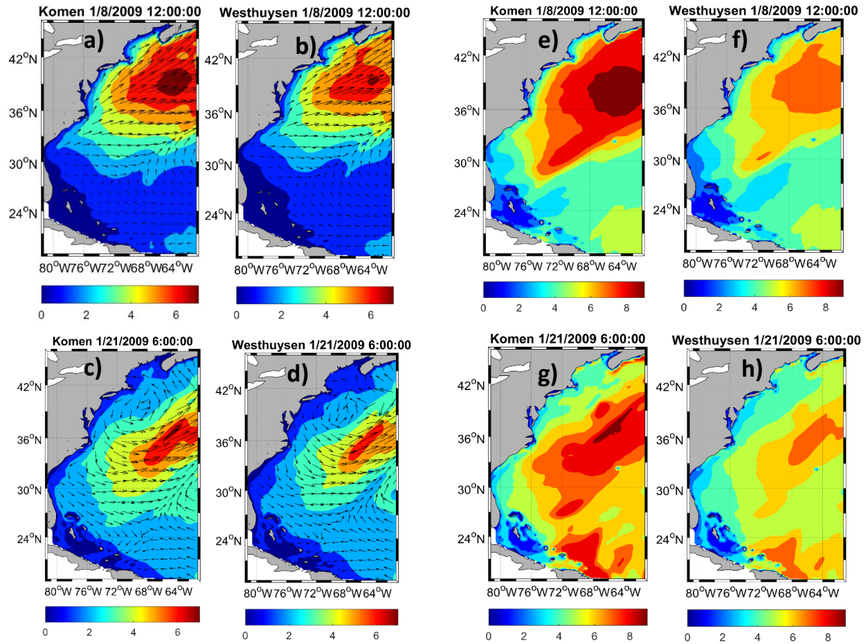
Figure9: Simulated wave height ( H_{m0} ) and direction over the modeling area using Komen and Westhuysen whitcapping formula for times t1 (a and b) and t2 (c and d) and simulation results for mean wave periods ( T_{m02} ) for times t1 (e and f) and t2 (g and h).
