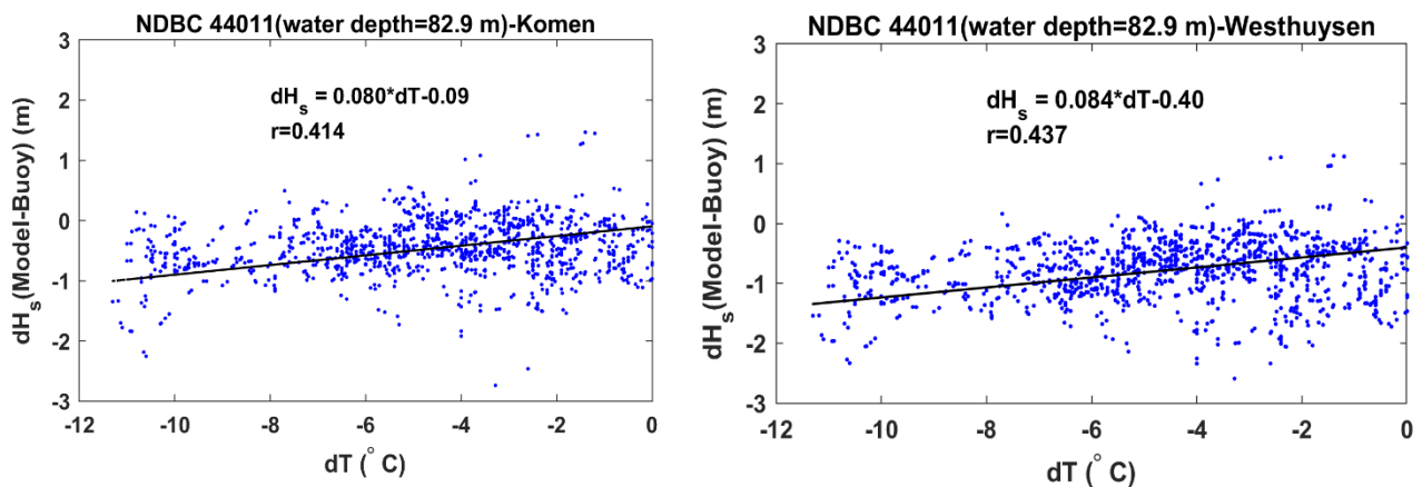
Figure17: Correlation between the air-sea temperature difference and deviations of the simulated wave height from the measurements at NDBC44011 for two whitcapping formulations
