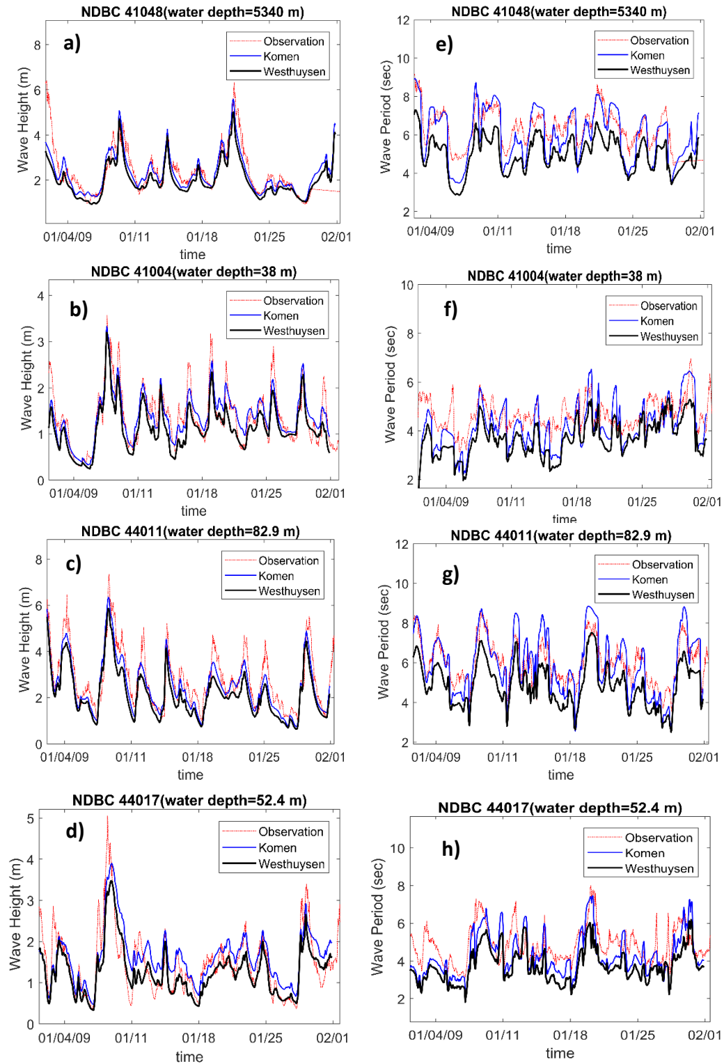
Figure 6: a-d) Time series of simulated wave heights and e-h) simulated mean wave periods, using Komen (blue lines) and Westhuysen (black lines) whitcapping formulas compared to measurements at the four NDBC buoys (dashed red lines).
