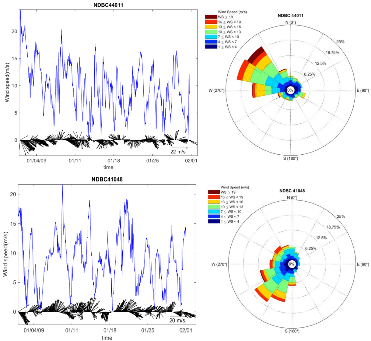
Figure2: Time series of measured wind speed (lines) and vectors (arrows) and the associated wind roses at NDBC buoys 44011 (upper) and 41048 (lower).
