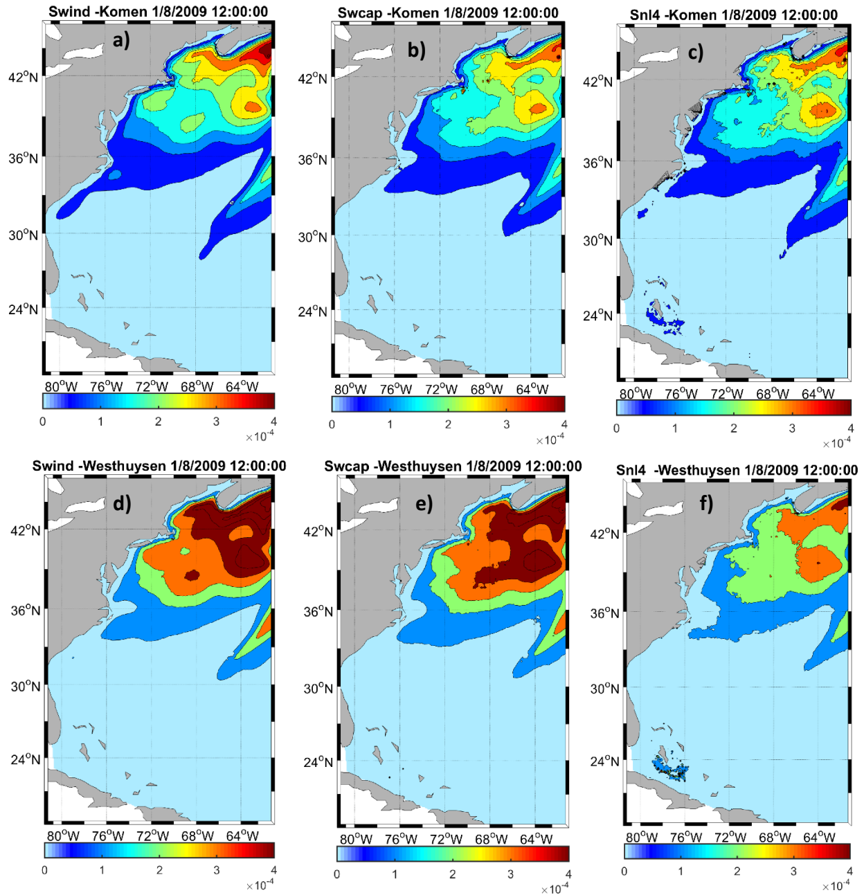
Figure11: Spatial variations of source terms (wind input, whitecapping dissipation, and quadruplet in m^2/s ) integrated in the spectral domain over the modeling area at time t1, for a-c) Komen and d-f) Westhuysen.
