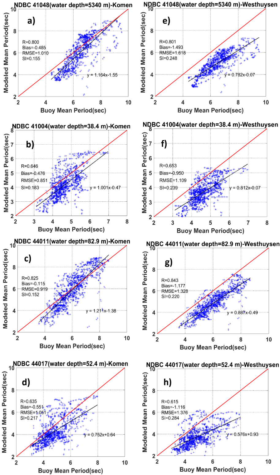
Figure8: Scatter plots and model performance metrics for simulated mean wave period using a-d) Komen whitecapping, and e-h) Westhuysen whitecapping at the NDBC buoys. The red and black lines are 1: 1 line and regression line respectively.
