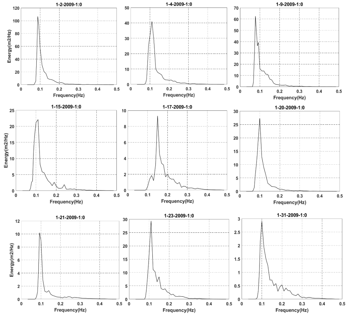
820 Figure3: Examples of single-peaked frequency spectra measured at NDBC 44011 in January 2009. The title for each panel 825 shows the date and time of measurement with the format month-day-year: hour: minute
