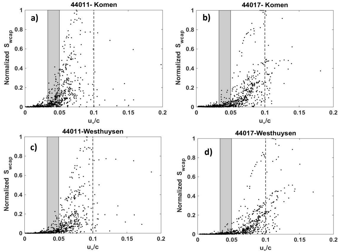
Figure13: Variations of the normalized whitecapping dissipation ( S_{wcap} ) from Komen and Westhuysen simulation scenarios with the inverse wave age \frac{u_s}{c} at a) and c) NDBC 44011, and b) and d) NDBC 44017. Gray boxes indicate the fully-developed zone ( 0.033 < \frac{u_s}{c} < 0.05 ). The dashed line separates zones for linear and quadratic growth based on Yan(198y) as indicated by \frac{u_s}{c} = 0.1 .
