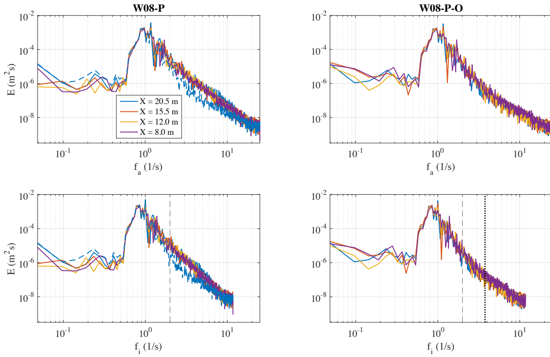
3 4 Figure 11: Wave energy spectra E(f_a) and E(f_i) of the water surface elevation z(t) at different fetches for the reference wind speed of 8 5 m/s and irregular paddle waves. (left) Clean water experiment W08-P. (right) Water with oil experiment W08-P-O (the spectrum at 6 the fetch X = 20.5 m is replicated with a dashed blue line on the left panel). On bottom panels the dashed grey vertical line shows the 7 maximum frequency (2 Hz) produced by the paddle, and the dotted black vertical line on the bottom-right panel shows the fish oil 8 resonance frequency f_{res} = \omega_{res}/(2\pi) = 3.77 Hz.
