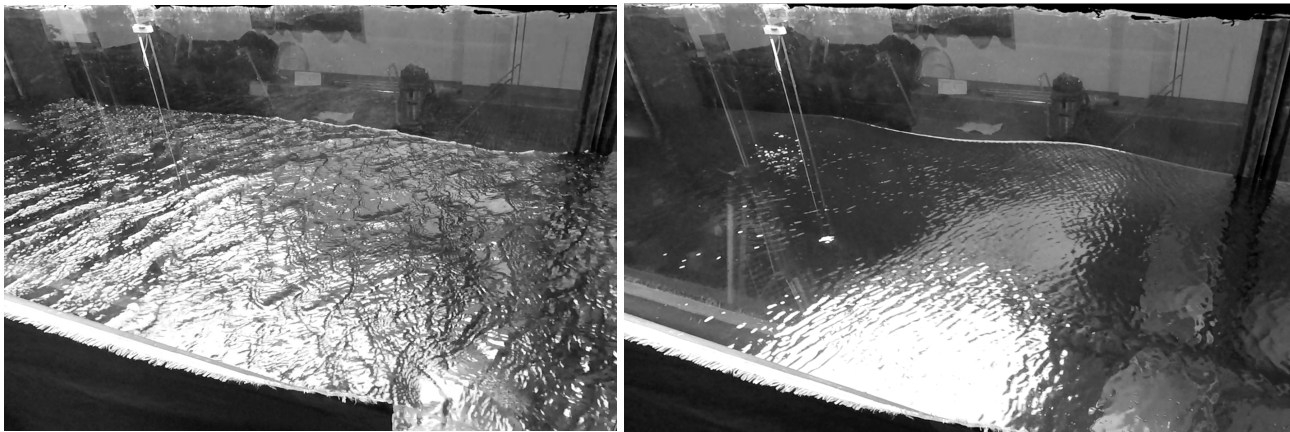
11 12 Figure 9: Two photographs of the water surface condition at fetch of about 20 m taken without (left panel, experiment W08-P) and 13 with oil instillation (right panel, experiment W08-P-O) onto wind-waves (wind blowing from left to right of the pictures at the 14 reference wind speed U_r = 8 m/s) and irregular paddle-waves. See also the videos available as supplementary material SM2.
