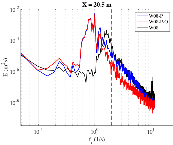
8 9 Figure 10: Variance density spectrum E(f_i) of the water surface elevation z(t) at fetch X = 20.5 m (wave probe G4) in presence of co- 10 existing wind and paddle waves in clean water (W08-P), wind and paddle waves in water with oil (W08-P-O), and wind waves only in 11 clean water (W08). The dashed grey vertical line shows the maximum frequency (2 Hz) produced by the paddle.
