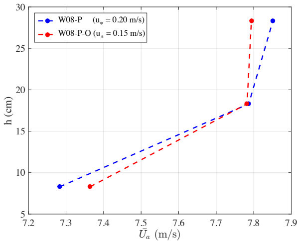
6 7 Figure 14: Vertical profile of the measured mean horizontal wind speed \bar{U}_a measured 8 over the water surface at fetch X = 11.5 m for co-existing wind- and paddle-generated waves in clean water condition (blue) and for 9 oil-covered surface after the oil instillation (red). In the legend, the value of the friction velocity is shown within brackets. Only the 10 value recorded at the three lowest Pitot tubes are shown.
