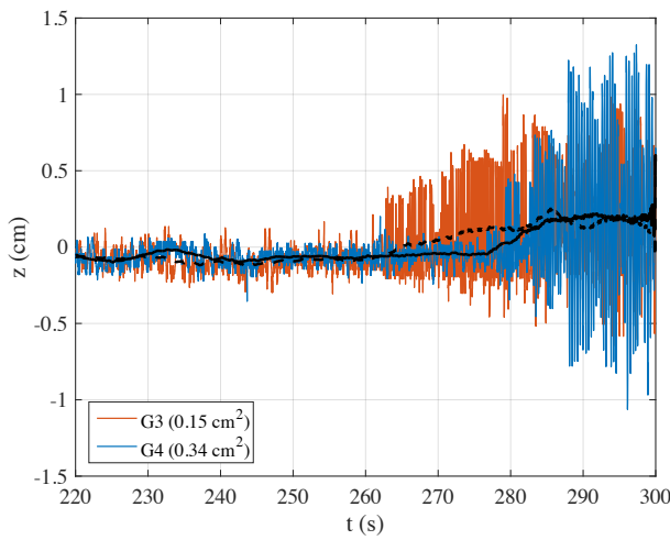
10 Figure 8: Sea surface elevation at probes G3 ( X = 15.5 m) and G4 ( X = 20.5 m) for an initially slick-covered surface without oil 11 instillation (experiment W06-O-NI). The dashed and solid black lines show the smoothed elevations (moving average of size 5 s) at 12 G3 and G4, respectively. In the legend, the variance of z(t) within the range of 290 \text{ s} \leq t \leq 300 \text{ s} is reported.
