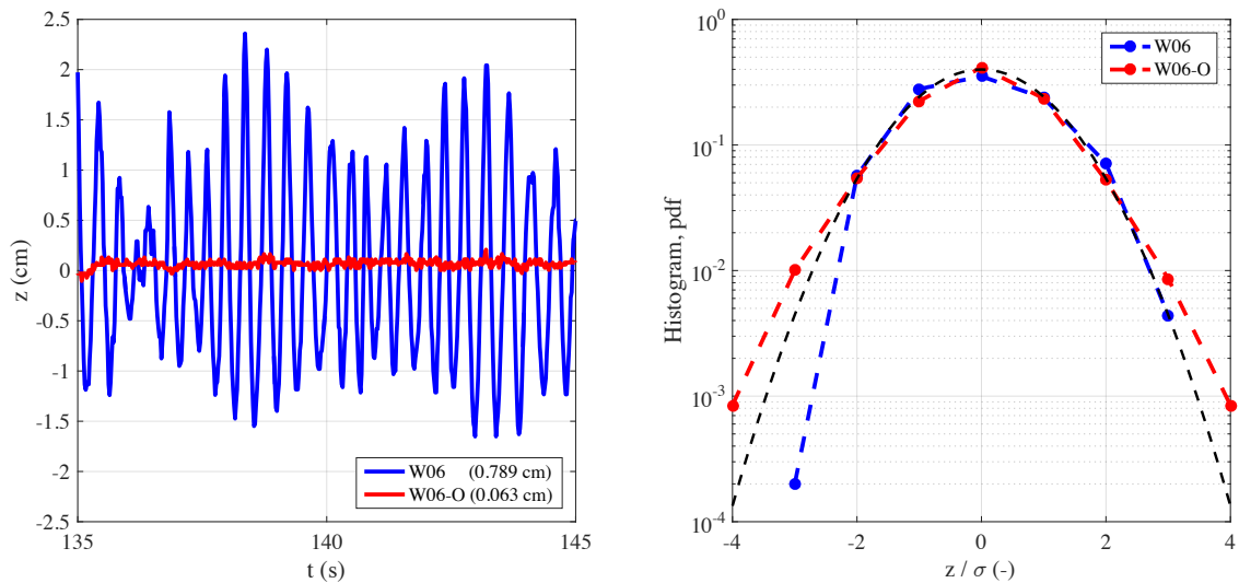
2 Figure 4: Sea surface elevation for clean (blue) and slick-covered (red) surface. (left) Extract Excerpt of the single-point record z(t) at 3 X = 20.5 m (probe G4) for the two conditions with clean water (experiment W06) and after the oil instillation (W06-O). In the legend, 4 the value of the standard deviation \sigma of z(t) is shown within brackets. (right) Histogram of the normalized elevations, high-pass 5 filtered above 1 Hz ( see discussion below ). The black dashed line shows the Gaussian probability density function (pdf).
