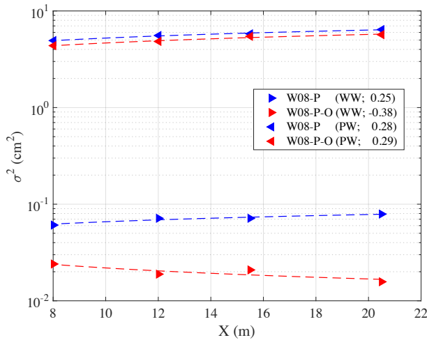
11 12 Figure 13: Spatial evolution of the water surface elevation variance \sigma^2 of co-existing wind (WW) and paddle (PW) waves in clean 13 water (W08-P) and with oil slick (W08-P-O). The solid and dashed lines show the power law-type function fitting the experimental 14 data. In the legend the coefficient \beta of the fitted power law is shown.
