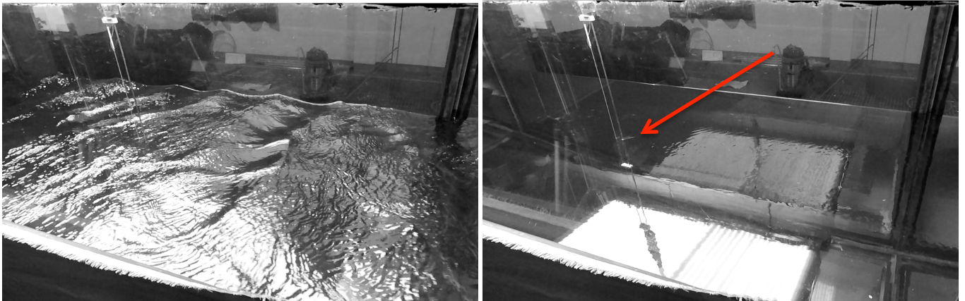
7 | 8 | Figure 2: Two photographs showing the water surface condition at fetch of about 20 m taken without (left panel) and with oil 9 | instillation (right panel). On both cases the water surface was forced with a reference wind speed U_r = 6 m/s (blowing from left to 10 | right on the pictures). The wave probe G4 is visible on the left-hand side of both pictures. The red arrow in the right panel points to 11 | the oscillating flow (vortex shedding) past the probe. See also the video available as supplementary material SM1.
