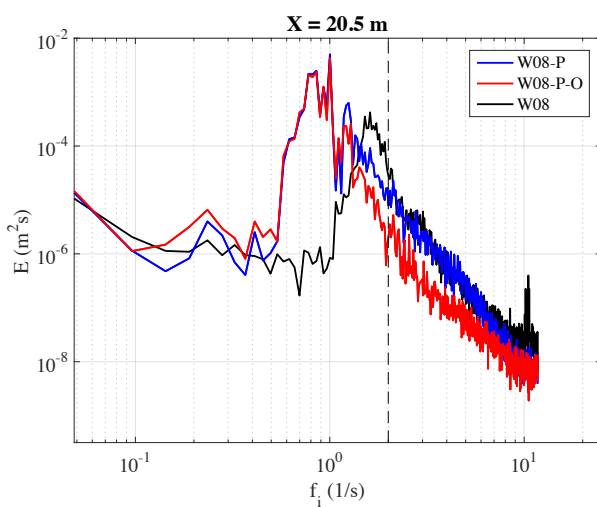
19 20 Figure 10: Variance density spectrum E(f_i) of the water surface elevation z(t) at fetch X = 20.5 m (wave probe G4) in presence of co- 21 existing wind and paddle waves in clean water (W08-P), wind and paddle waves in water with oil (W08-P-O), and wind waves only in 22 clean water (W08). The dashed gray vertical line shows the maximum frequency (2 Hz) produced by the paddle.
