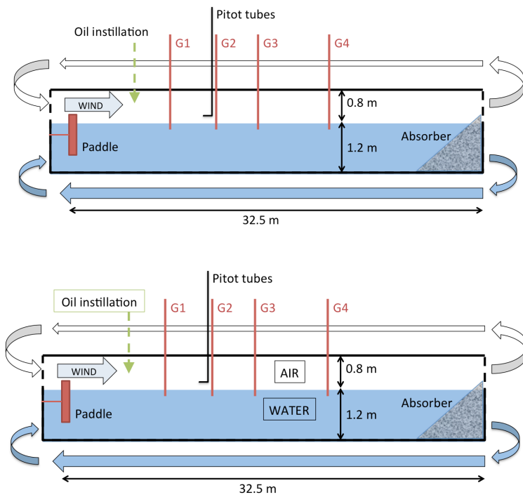
12 13 14 Figure 1: Schematic longitudinal diagram of the wave flume arrangement at the First Institute of Oceanography (FIO) flume 15 (Qingdao, P.R. China). For the sake of clarity, horizontal and vertical scales are distorted. The arrows indicate the direction of the 16 flow.
