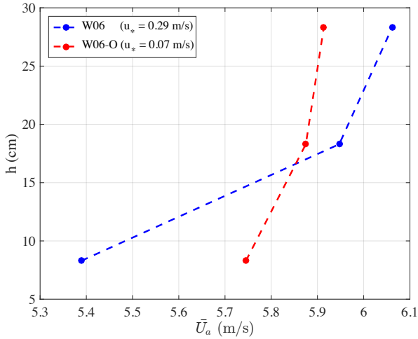
6 Figure 3: Vertical profile of the mean horizontal wind speed the wind velocity component \bar{U}_a measured over the water surface at 7 fetch X = 11.5 \text{ m} . Reference wind speed U_r = 6 \text{ m/s} . Clean water conditions (blue) and oil-covered surface (red). In the legend, the 8 value of the airflow friction velocity u_* is shown within brackets. Only the value recorded at the three lowest Pitot tubes are shown.
