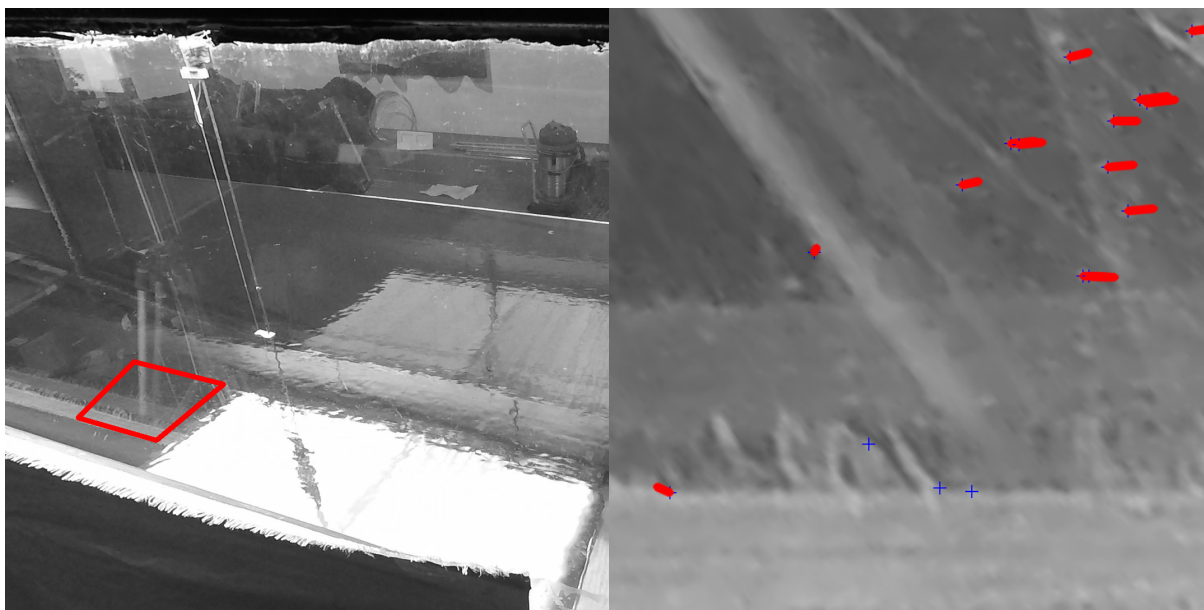
2 Figure 15: Estimate of surface current speed by optical flow during experiment W06-O. (left) Bounded by a red polygon, the surface 3 area used for the determination of the flow. (right) Example of detected particles with their corresponding movement vector . The 4 wind was blowing from the left side to the right side of the images (wind blowing from left to right of the pictures).
