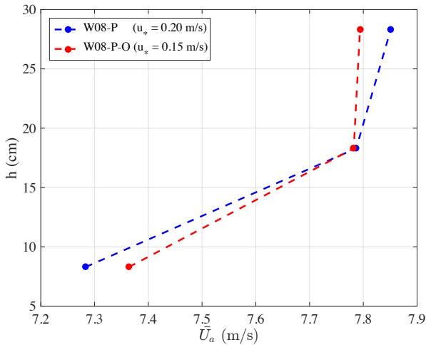
6 Figure 14: Vertical profile of the measured mean horizontal wind speed \bar{U}_a measured 7 over the water surface at fetch X = 11.5 m for co-existing wind- and paddle-generated waves in clean water condition (blue) and 8 oil-covered surface after the oil instillation (red). In the legend, the value of the friction velocity is shown within brackets. Only the 9 value recorded at the three lowest Pitot tubes are shown.
