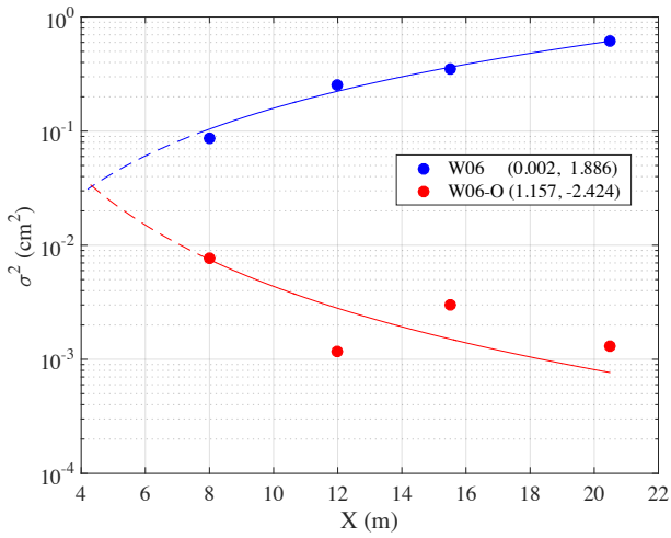
Figure 7: Spatial evolution of the water surface elevation variance \sigma^2 in clean water (W06) and with fish oil slick (W06-O). The solid lines are the power law-type function \sigma^2 = \alpha X^\beta fitting the observations (in the legend, the coefficient \alpha and \beta , respectively, are tabulated), while the dashed lines show the laws extended outside the observed data interval.
