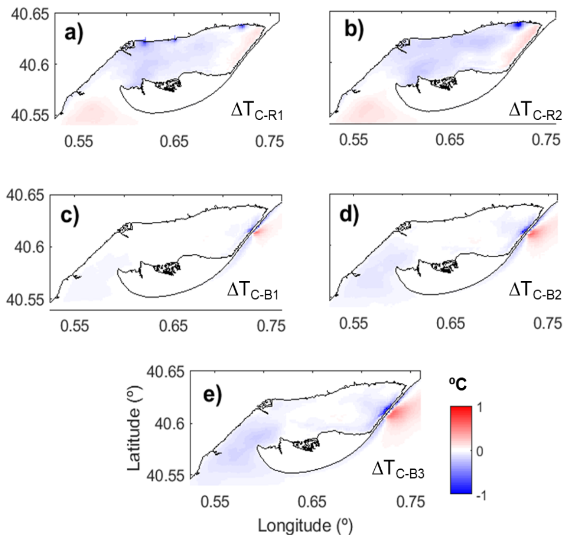
Figure 6. Differences for the SST between each test case and Control Simulation (C). Blue color indicates lower SST for the corresponding test compared with C (red colors indicates lower SST for the Control Simulation).
