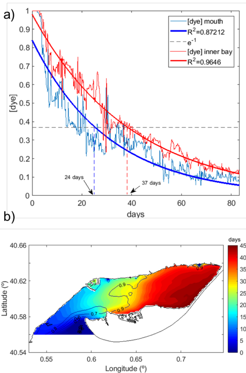
Figure 4. a) Shows the time-evolution of the dye concentration at two points -at the bay mouth and inside the bay- and the corresponding exponential fitting (with the squared correlation shown in the legend) used to obtain the LFT for the C case. b) shows the local e-flushing time for the C case (color). The black contour shows the squared correlation obtained at each of the grid points.
