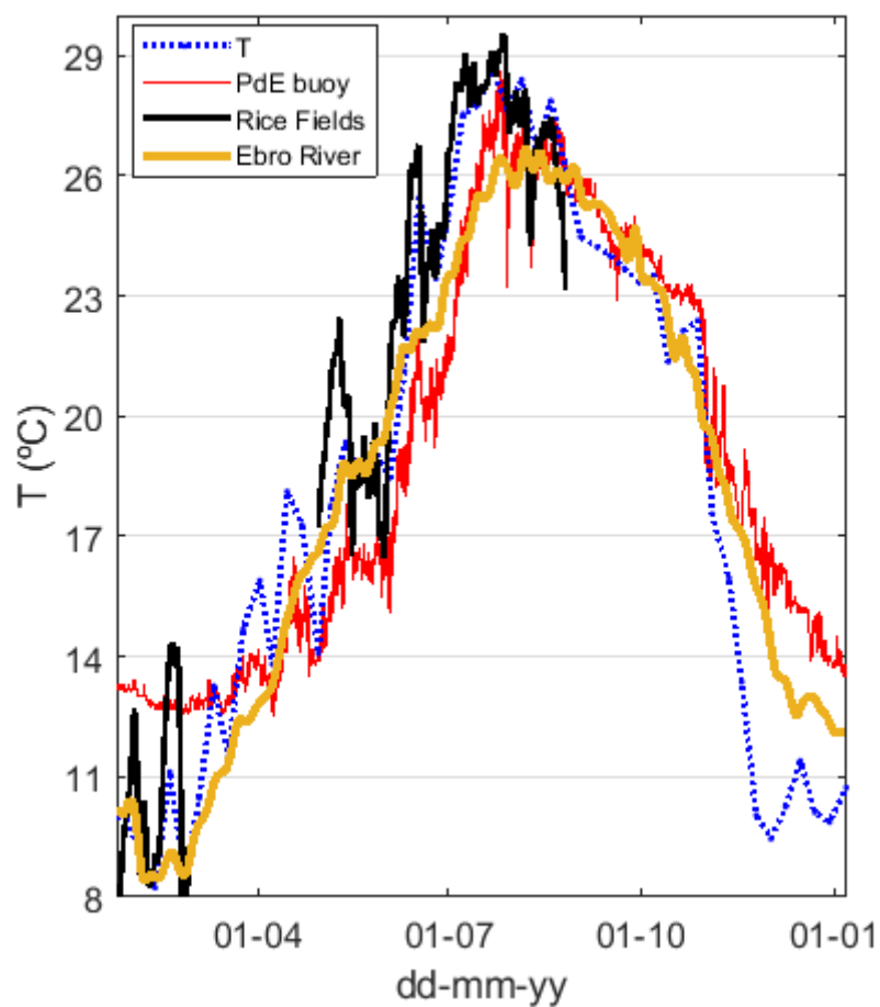
Figure 2. Water temperatures in Alfacs Bay at point T (year 2014), drainage-channels (Rice fields, from climatological observations -2002-2010- in a nearby coastal lagoon by the staff of the Delta Ebro Natural Park), Tarragona buoy (Tb) for open sea water conditions ( Puertos del Estado , PdE) and climatological data from Ebro River ( Confederación Hidrográfica del Ebro ).
