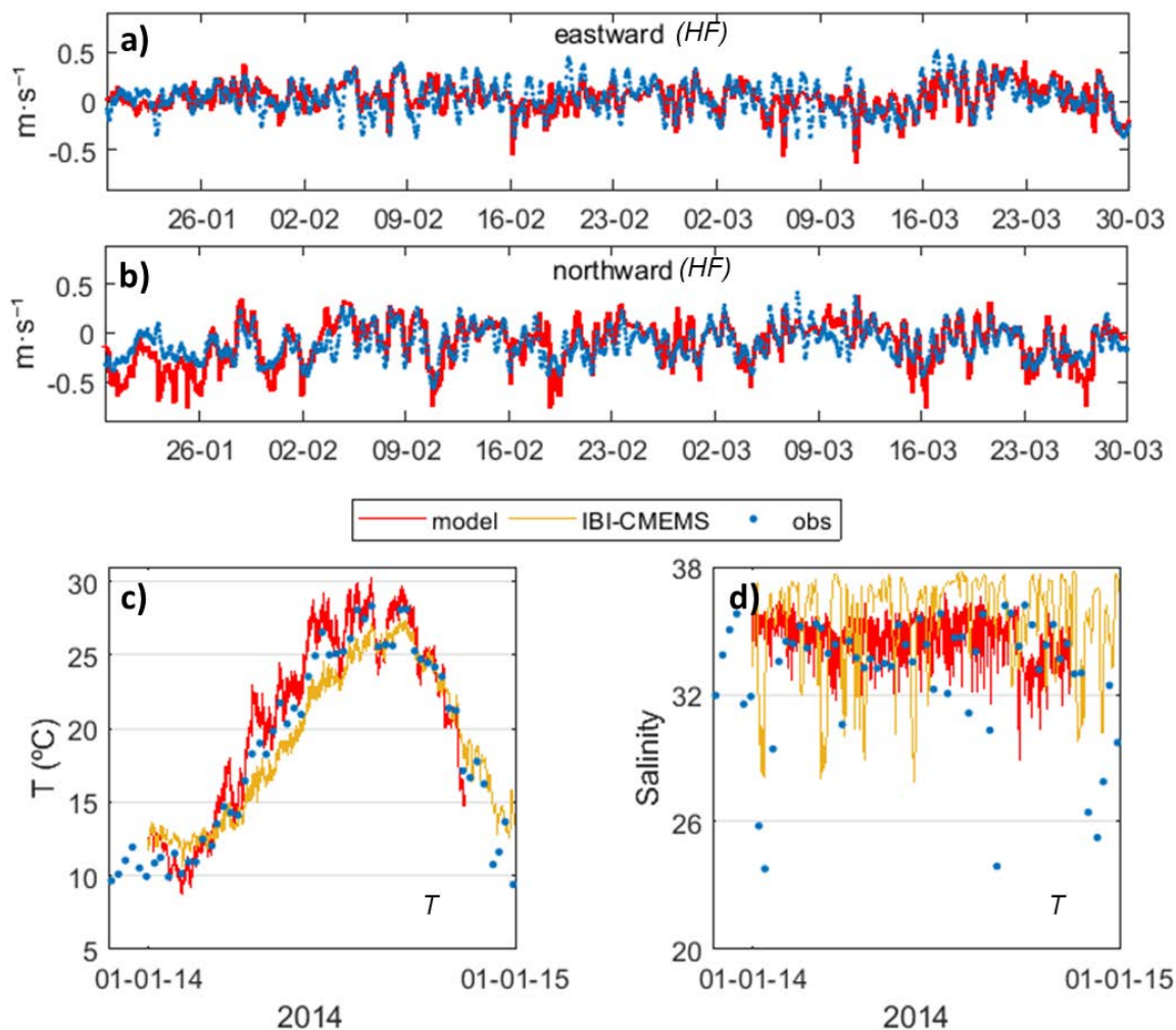
Figure 3. Eastward (a) and northward (b) water surface currents for D-A model and HF-Radar at HF (Fig.1) are shown. SST (c) and SSS (d) validation of the local model D-B (red), CMEMS-IBI (yellow) and observations (blue) at T (Fig.1).
