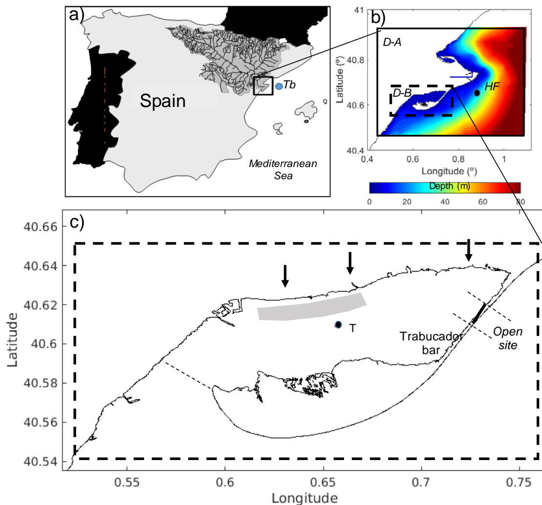
Figure 1: Location of Delta Ebro and Alfacs Bay and Pde Tarragona buoy (blue point, Tb) (a). b) shows the nesting scheme, with the coastal (D-A) and bay (D-B) domains and bathymetry. Data from High frequency Radar used to validate the system is indicated as “HF”. In c) the location of the weekly CTDs is indicated (T). The opening area of the Trabucador bar modified in the numerical experiments is also shown. The dashed line in the bay mouth indicates the separation between the inner bay and open sea for the salinity box model. The grey rectangle indicates the mussel farm area. The freshwater drainage channels locations are indicated with arrows.
