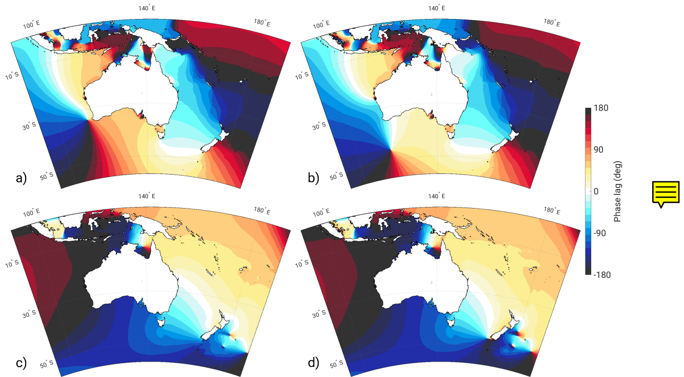
Figure 4. The constituent phase lags with respect to the Greenwich Meridian (deg) for the control (left) and 7 m SLR (right) simulations for M_2 (top) and K_1 (bottom)
