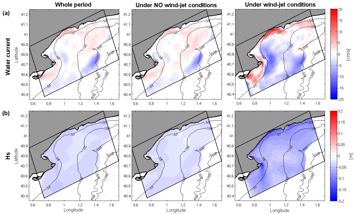
Figure 7. (a) Water-Surface water current and (b) Hs mean of of the hourly instantaneous differences between the uncSluncR run and the cRS run considering the whole period (left), the whole period except the wind-jet events (centre) and during the four wind-jet events (right). Positive values correspond to cRS value > uncSluncR value.
