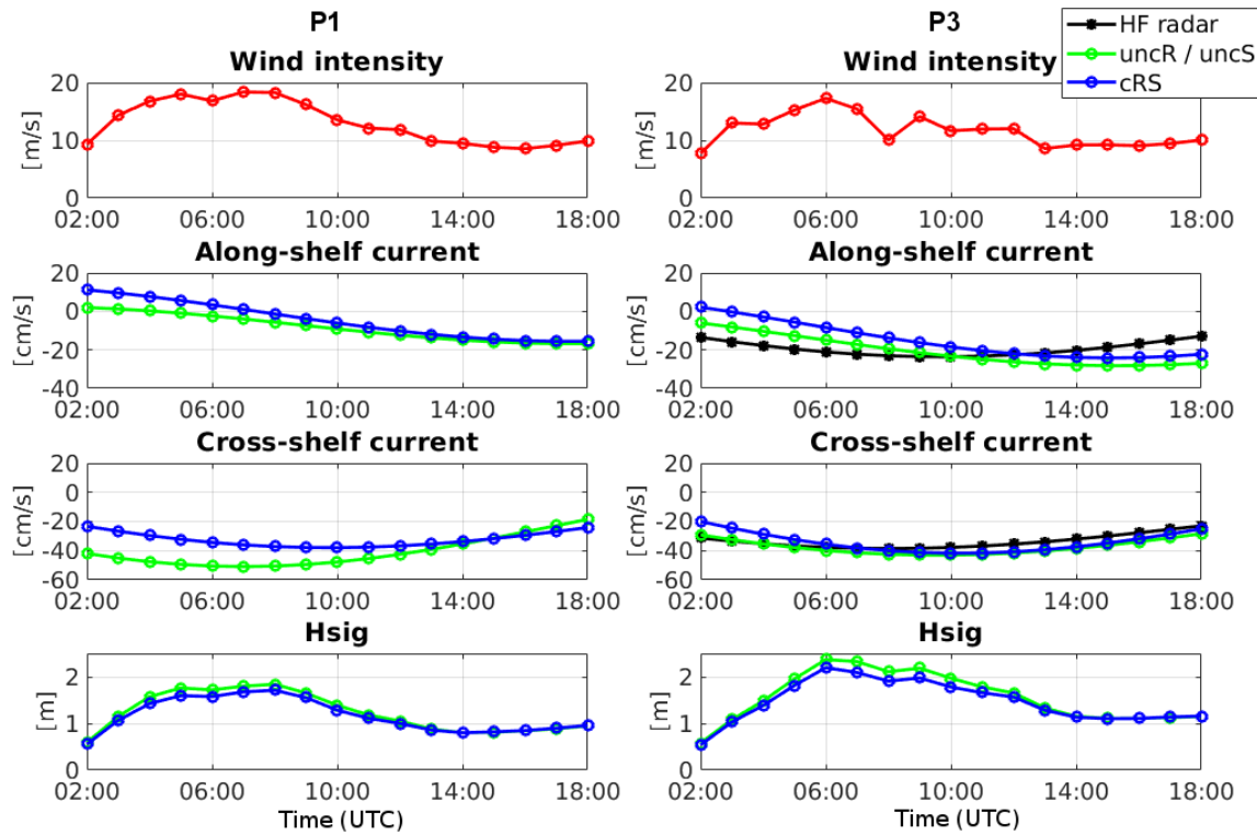
Figure 5. Wind intensity, along- and cross-shelf subinertial surface currents and Hsig time series at P1 and P3 during the wind-jet event E3 (25 April 2014). Negative values mean offshore and southwestwards. In red, the modeled wind intensity, in black the HF radar data, in green the uncR and uncS runs results and in blue the cRS run results.
