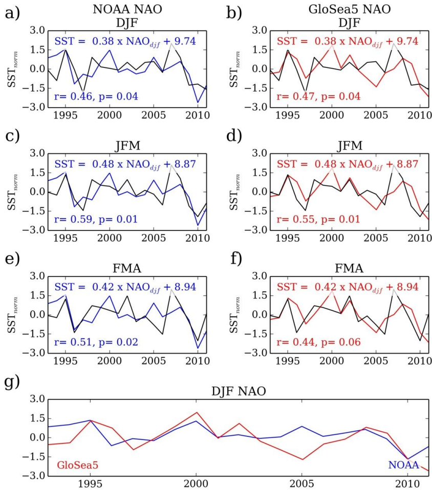
Figure 10 Exemplar regional seasonal forecast of English Channel SST (selected for the strength of the correlations): The seasonal 5 forecasts is based on the linear relationship between the reanalysis SST, and the observed NAO (blue, left column: a, c, e) which is then applied to the GloSea5 Forecast NAO (red, second column, b, d, f). Each forecast (coloured line) is based on the DJF NAO, with each row showing the consecutive month (first column: DJF forecast; a, b; second row: JFM forecast; c, d; third row: FMA forecast; e, f). For each panel, the black line represents the NWS reanalysis SST, which is the same for both the observed and GloSea5 NAO plots for that row. The coloured line represents the DJF NAO based forecast – while the amplitude of this varies 10 with lag (due to the different equation), the pattern is based on the same DJF NAO, and so the pattern remains the same for each column of a given row. Both modelled and forecast line have been normalised (removing the mean and dividing by the standard deviation) – this does not affect the strength or significance of the correlation. The equation for the forecast is given (before normalisation), with the strength of the correlations in each panel. The lowest panel (g) shows the time-series of the observed (blue) and GloSea5 forecast DJF NAO (red).
