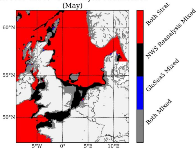
Figure 2 a Upper panel) 20-year mean seasonal cycle of stratified extent for CO5 NWS reanalysis (black) and GloSea5 (blue). b Lower Panel) 20-year mean stratification map (for May, where (SST - NBT) = 0.5 \text{ } ^\circ\text{C} ). Grey and red denote regions where both models agree that there is a mixed and stratified water column respectively. Black and Blue denote regions where the CO5 NWS reanalysis and GloSea5 disagree – black being where NWS considers the water column to be mixed, while GloSea5 considers it to be mixed, and blue being the opposite.
