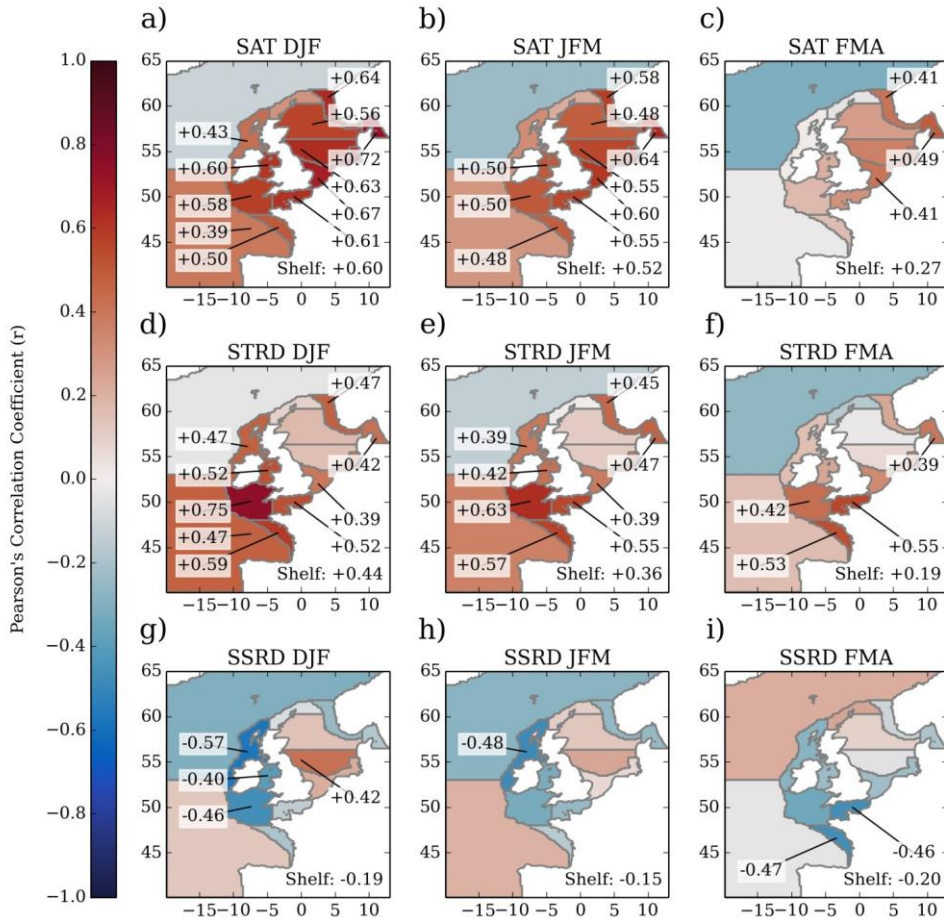
Figure 6 Correlation maps between winter (DJF) NAO and atmospheric surface fields associated with shelf temperature (Surface Air Temperature (SAT; a-c), Downwards component of the Thermal Radiation at the surface (STRD; d-f) and Downwards component of the Short-wave (Solar) Radiation (SSRD; g-i), upper to lower rows respectively). The left hand panels denote zero-lag (a, d, g), correlating the winter (DJF) NAO with the winter (DJF) surface forcing. The following columns denote 1 and 2 month lags, correlating the winter (DJF) NAO against the JFM (Jan-Mar; b, e, h), FMA (Feb-Apr; c, f, i) surface forcing respectively. The correlation values are given for the shelf, and for regions where the correlation is significant at the 95 % confidence level.
