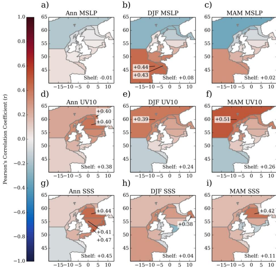
Figure 12 Correlations between winter (DJF) storm track latitude, and Annual mean, winter and spring (left to right) mean sea level pressure (MSLP; a-c), wind magnitude (UV10; d-f), and surface salinity (SSS; g-i).
