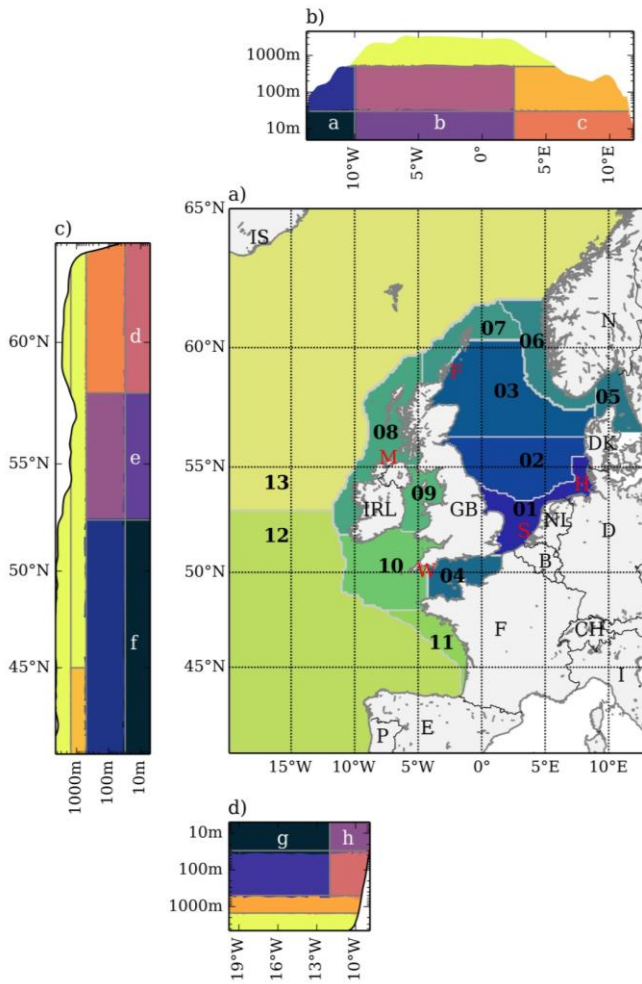
5 Figure 1 a) CO5 NWS reanalysis domain with coloured analysis regions-, numbered as: 01 Southern North Sea; 02 Central North Sea; 03 Northern North Sea; 04 English Channel; 05 Skagerrak/Kattegat; 06 Norwegian Trench; 07 Shetland Shelf; 08 Irish Shelf; 09 Irish Sea; 10 Celtic Sea; 11 Armorican Shelf; 12 NE Atlantic (S); 13 NE Atlantic (N). Red lettering shows observation locations: F, Fair Isle; M, Malin Head; H, Helgoland Roads; S, Southern North Sea ferry box data; W, Western Channel Observatory. b-d) Region mask used for the oceanic lateral boundary condition: b) The Northern Boundary is divided at 10° W and 2.5° E, and at 30 m and 500 m (below 500 m the boundary is not separated by longitude); c) The Western Boundary is separated at 30 m and 500 m, and at 52.5° N and 58° N. Mediterranean Intermediate Water is identified between 500 m and 1500 m south of 45° N, and this is separated. d) The Southern Boundary is divided at 30 m, 500 m and 1500 m. Above 500 m the boundary is separated at 12° W. The white letters in the outer panels (b-d) refer to the surface lateral boundary regions used in this analysis: a, NBC (Wst); b, NBC (CtI); c, NBC (Est); d, WBC (Nth); e, WBC (CtI) (used in Figure 11a, b); f, WBC (Sth); g, SBC (Wst); h, SBC (Est) (used in Figure 11d, e). 10 15
