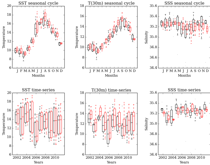
Modelled (red) and observed (black) T and S from the WCO
