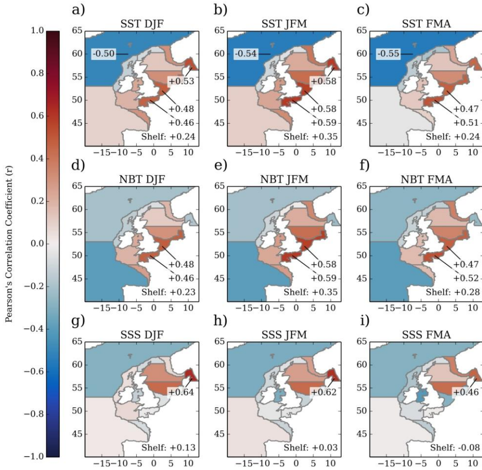
Figure 8 As Figure 6, but for the shelf response itself: SST (a-c), NBT (d-f) and SSS (g-i).
