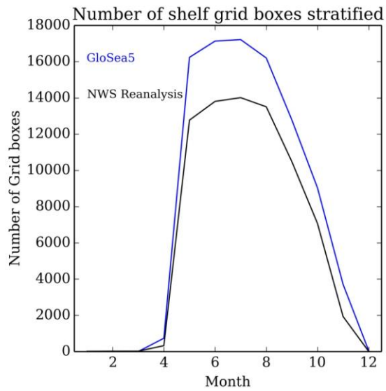
GloSea5 and NWS Reanalysis stratification (May)
