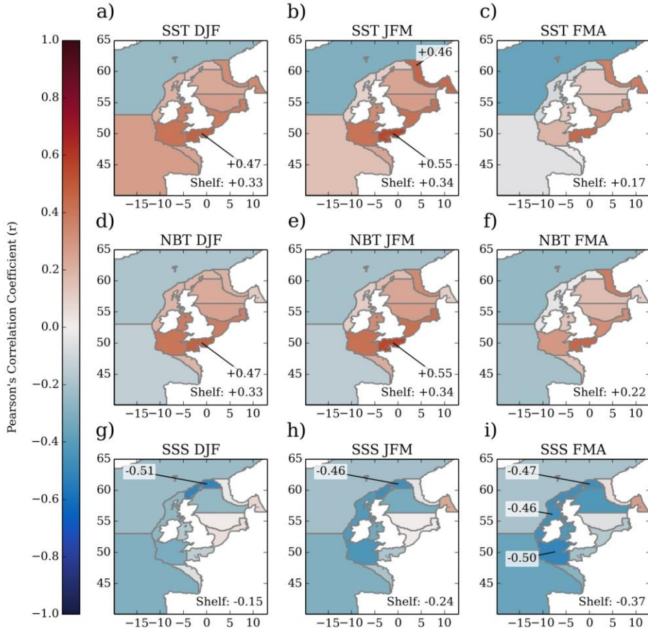
Figure 9 As with Figure 7, but using the GloSea5 forecast DJF NAO: SST (a-c), NBT (d-f) and SSS (g-i).
