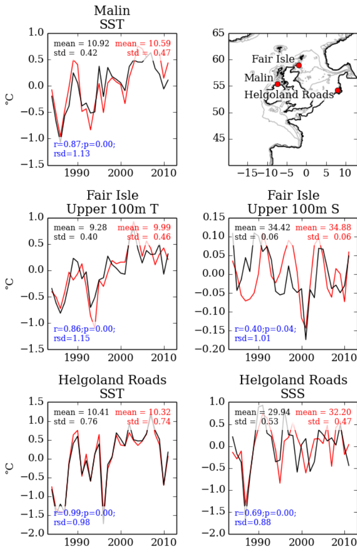
5 Figure 5 Reanalysis evaluation with ICES temperature and salinity data. Data is presented as anomalies (the time-series mean is removed) to highlight the variability (reanalysis red; observations black), however the mean and standard deviation (and Pearson's correlation coefficient ( r , with its significance ( p )), relative standard deviation ( rsd ), and root mean square) are given. Temperature (left panels) and salinity (right panels) from three ICES time series: Malin Head (upper left); Fair Isle (middle row) and Helgoland Roads (lower row). Upper right panel shows the location of these time-series (the Malin Head dataset does not include salinity).
