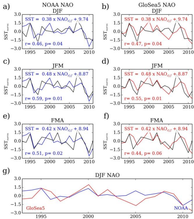
Figure 10 Exemplar regional seasonal forecast of English Channel SST (selected for the strength of the correlations): The seasonal forecasts is based on the linear relationship between the reanalysis SST, and the observed NAO (blue, left column: a, c, e) which is then applied to the GloSea5 Forecast NAO (red, second column, b, d, f). Each forecast (coloured line) is based on the DJF NAO, with each row showing the consecutive month (first column: DJF forecast; a, b; second row: JFM forecast; c, d; third row: FMA forecast; e, f). For each panel, the black line represents the NWS reanalysis SST, which is the same for both the observed and GloSea5 NAO plots for that row. The coloured line represents the DJF NAO based forecast – while the amplitude of this varies with lag (due to the different equation), the pattern is based on the same DJF NAO, and so the pattern remains the same for each column of a given row. Both modelled and forecast line have been normalised (removing the mean and dividing by the standard deviation) – this does not affect the strength or significance of the correlation. The equation for the forecast is given (before normalisation), with the strength of the correlations in each panel. The lowest panel (g) shows the time-series of the observed (blue) and GloSea5 forecast DJF NAO (red).
