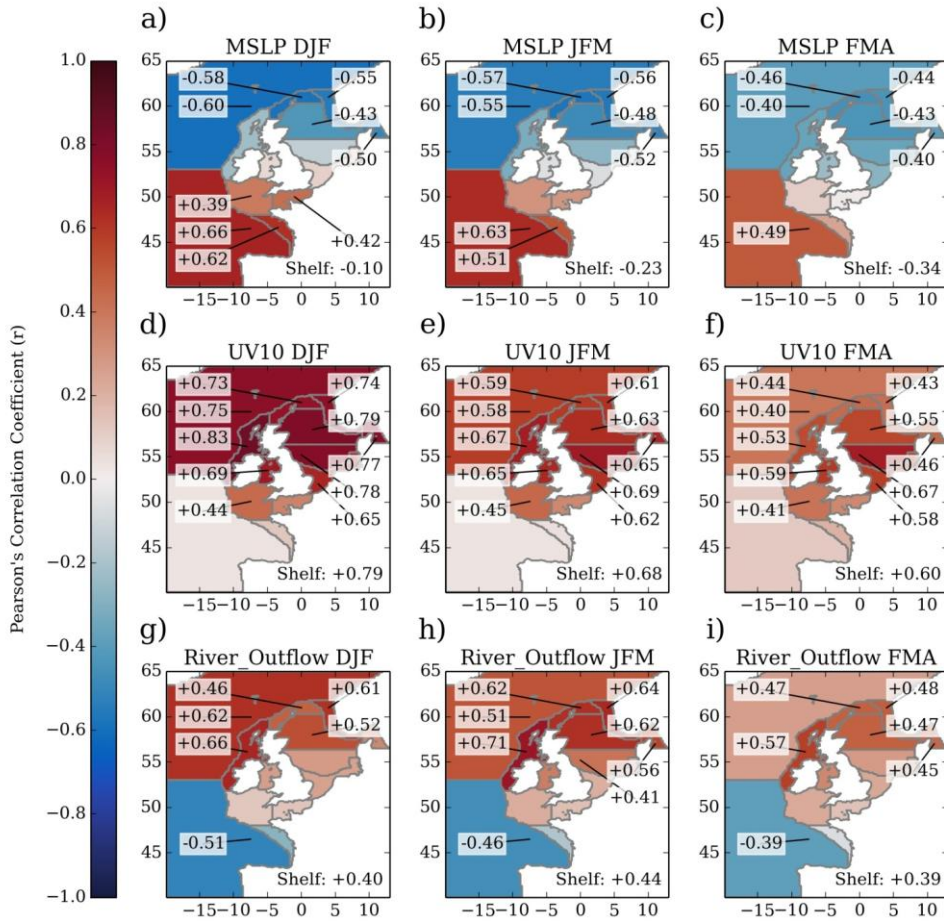
Figure 7 As Figure 6, but for atmospheric surface fields associated with SSS variability: Mean Sea Level Pressure (MSLP; a-c), wind magnitude (UV10; d-f) and river outflow (g-i).
