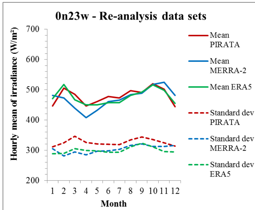
Monthly means (line) and standard deviations (dotted line) of hourly DSIS, in W\ m^{-2} , from PIRATA measurements (red) and data sets (MERRA-2: blue, ERA5: green) at (0°N, 23°W). A difference between red line (measurements) and coloured line (data set) for a given month denotes a systematic error for this month: underestimation if the coloured line is below the red line, overestimation otherwise. For a given month, a coloured dotted line above the red one means that the data set produces too much variability for this month; in the opposite case, the data set does not contain enough variability.
