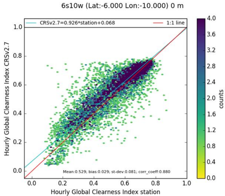
Figure 2: 2D histogram of PIRATA measurements (horizontal axis) and data sets (vertical axis) at (6°S, 10°W) for E and KT . HC3v5: (a) and (b); SARA-2: (c) and (d); CRS: (e) and (f). Ideally, the dots should lie along the red line (1:1 line). The blue line is the affine function fitted over the points and should ideally overlay the red line.
