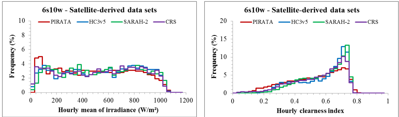
10 Figure 3: Frequency distributions of PIRATA measurements (red) and data sets (HC3v5: blue, SARA-2: green, CRS: purple) at (6^\circ\text{S}, 10^\circ\text{W}) for E (left) and KT (right). If the coloured line is above, respectively below, the red one for a given sub-range of values, it means that the data set produces these values too frequently, respectively too rarely with respect to the PIRATA measurements.
