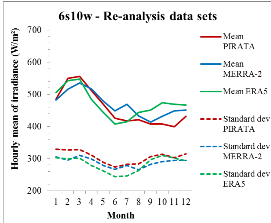
Figure 8: Monthly means (line) and standard deviations (dotted line) of hourly DSIS, in W m^{-2} , from PIRATA measurements (red) and data sets (MERRA-2: blue, ERA5: green) at (6°S, 10°W). A difference between red line (measurements) and coloured line (data set) for a given month denotes a systematic error for this month: underestimation if the coloured line is below the red line, overestimation otherwise. For a given month, a coloured dotted line above the red one means that the data set produces too much variability for this month; in the opposite case, the data set does not contain enough variability.
