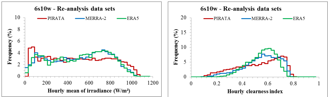
Figure 7: Frequency distributions of PIRATA measurements (red) and data sets (MERRA-2: blue, ERA5: green) at (6°S, 10°W) for E (left) and KT (right). If the coloured line is above, respectively below, the red one for a given sub-range of values, it means that the data set produces these values too frequently, respectively too rarely with respect to the PIRATA measurements.
