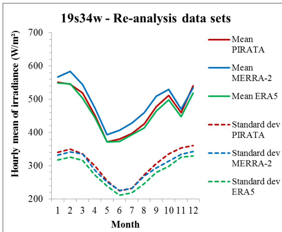
Monthly means (line) and standard deviations (dotted line) of hourly DSIS, in W\ m^{-2} , from PIRATA measurements (red) and data sets (MERRA-2: blue, ERA5: green) at (19°S, 34°W). A difference between red line (measurements) and coloured line (data set) for a given month denotes a systematic error for this month: underestimation if the coloured line is below the red line, overestimation otherwise. For a given month, a coloured dotted line above the red one means that the data set produces too much variability for this month; in the opposite case, the data set does not contain enough variability.
