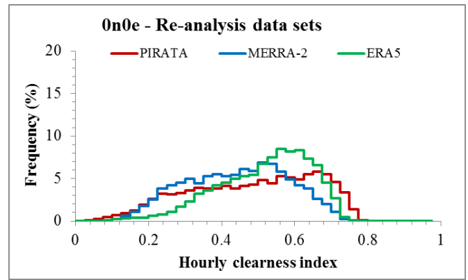
Frequency distributions of PIRATA measurements (red) and data sets (MERRA-2: blue, ERA5: green) at (0°N, 0°E) for E (left) and KT (right). If the coloured line is above, respectively below, the red one for a given sub-range of values, it means that the data set produces these values too frequently, respectively too rarely with respect to the PIRATA measurements.
