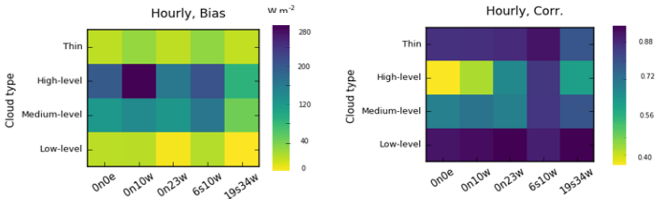
Figure 10: Bias (left, in \text{W m}^{-2} ) and correlation coefficient (right) as a function of the cloud type at each PIRATA buoy for ERA5.
