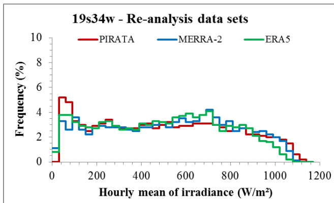
Frequency distributions of PIRATA measurements (red) and data sets (MERRA-2: blue, ERA5: green) at (19°S, 34°W) for E (left) and KT (right). If the coloured line is above, respectively below, the red one for a given sub-range of values, it means that the data set produces these values too frequently, respectively too rarely with respect to the PIRATA measurements.
