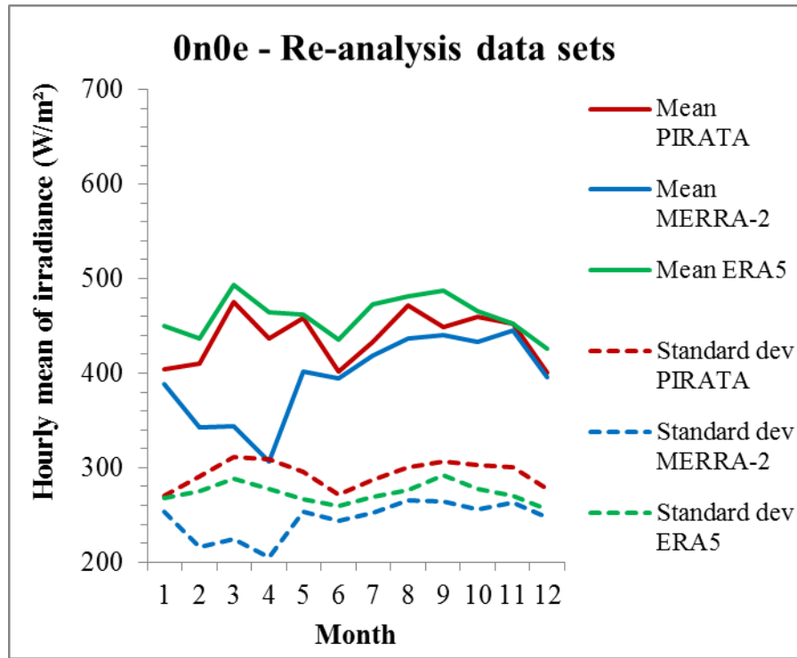
Monthly means (line) and standard deviations (dotted line) of hourly DSIS, in W\ m^{-2} , from PIRATA measurements (red) and data sets (MERRA-2: blue, ERA5: green) at (0°N, 0°E). A difference between red line (measurements) and coloured line (data set) for a given month denotes a systematic error for this month: underestimation if the coloured line is below the red line, overestimation otherwise. For a given month, a coloured dotted line above the red one means that the data set produces too much variability for this month; in the opposite case, the data set does not contain enough variability.
