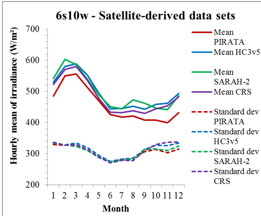
Figure 4: Monthly means (line) and standard deviations (dotted line) of hourly DSIS, in W m^{-2} , from PIRATA measurements (red) and data sets (HC3v5: blue; SARA2: green; CRS: purple) at (6°S, 10°W). A difference between red line (measurements) and coloured line (data set) for a given month denotes a systematic error for this month: underestimation if the coloured line is below the red line, overestimation otherwise. For a given month, a coloured dotted line above the red one means that the data set produces too much variability for this month; in the opposite case, the data set does not contain enough variability.
