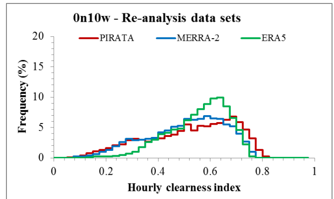
Frequency distributions of PIRATA measurements (red) and data sets (MERRA-2: blue, ERA5: green) at (0°N, 10°W) for E (left) and KT (right). If the coloured line is above, respectively below, the red one for a given sub-range of values, it means that the data set produces these values too frequently, respectively too rarely with respect to the PIRATA measurements.
