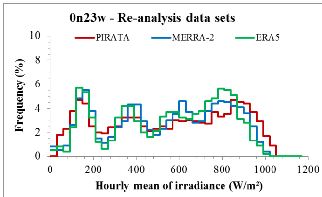
Frequency distributions of PIRATA measurements (red) and data sets (MERRA-2: blue, ERA5: green) at (0°N, 23°W) for E (left) and KT (right). If the coloured line is above, respectively below, the red one for a given sub-range of values, it means that the data set produces these values too frequently, respectively too rarely with respect to the PIRATA measurements.
