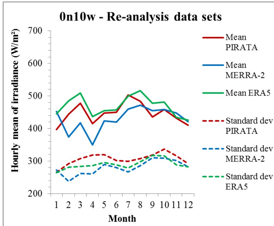
Monthly means (line) and standard deviations (dotted line) of hourly DSIS, in W\ m^{-2} , from PIRATA measurements (red) and data sets (MERRA-2: blue, ERA5: green) at (0°N, 10°W). A difference between red line (measurements) and coloured line (data set) for a given month denotes a systematic error for this month: underestimation if the coloured line is below the red line, overestimation otherwise. For a given month, a coloured dotted line above the red one means that the data set produces too much variability for this month; in the opposite case, the data set does not contain enough variability.
