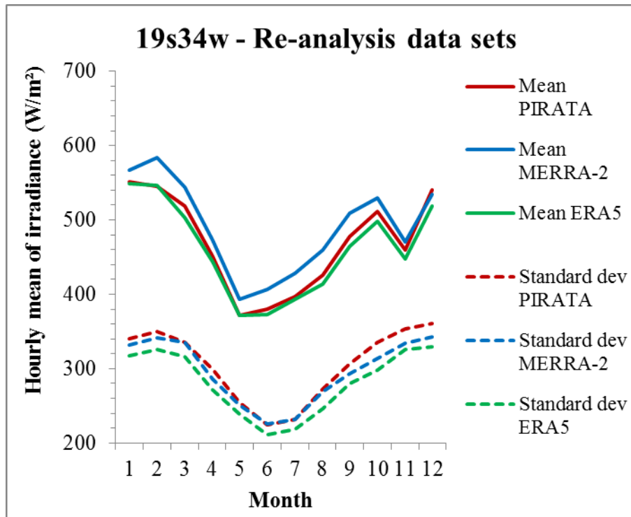
Monthly means (line) and standard deviations (dotted line) of hourly DSIS, in W m^{-2} , from PIRATA measurements (red) and data sets (MERRA-2: blue, ERA5: green) at 19s34w. A difference between red line (measurements) and coloured line (data set) for a given month denotes a systematic error for this month: underestimation if the coloured line is below the red line, overestimation otherwise. For a given month, a coloured dotted line above the red one means that the data set produces too much variability for this month; in the opposite case, the data set does not contain enough variability.
