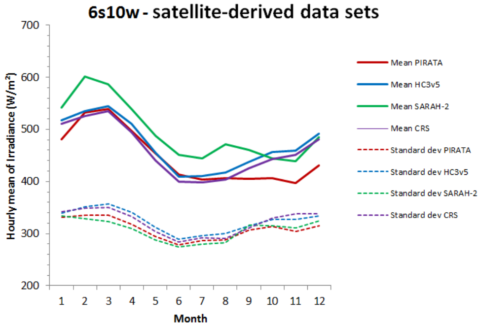
5 Figure 4: Monthly means (line) and standard deviations (dotted line) of hourly DSIS, in W m^{-2} , from PIRATA measurements (red) and data sets (HC3v5: blue ; SARA2: green; CRS: purple) at 6s10w. A difference between red line (measurements) and coloured line (data set) for a given month denotes a systematic error for this month: underestimation if the coloured line is below the red line, overestimation otherwise. For a given month, a coloured dotted line above the red one means that the data set produces too much variability for this month; in the opposite case, the data set does not contain enough variability.
