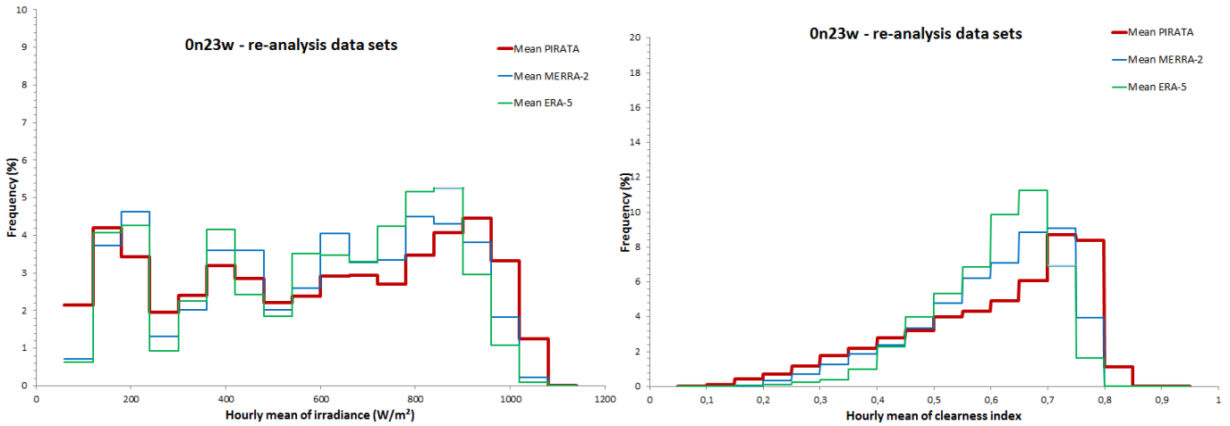
Frequency distributions of PIRATA measurements (red) and data sets (MERRA-2: blue, ERA5: green) for the station 0n23w for E (left) and KT (right). If the coloured line is above, respectively below, the red one for a given sub-range of values, it means that the data set produces these values too frequently, respectively too rarely with respect to the PIRATA measurements.
