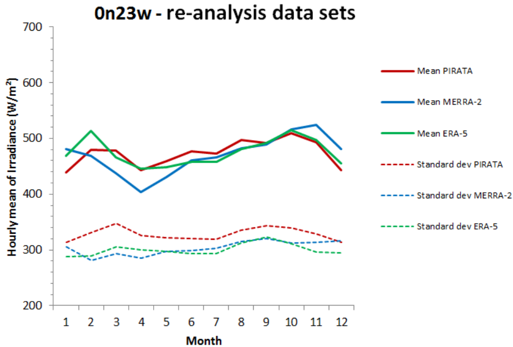
Monthly means (line) and standard deviations (dotted line) of hourly DSIS, in W\ m^{-2} , from PIRATA measurements (red) and data sets (MERRA-2: blue, ERA5: green) at 0n23w. A difference between red line (measurements) and coloured line (data set) for a given month denotes a systematic error for this month: underestimation if the coloured line is below the red line, overestimation otherwise. For a given month, a coloured dotted line above the red one means that the data set produces too much variability for this month; in the opposite case, the data set does not contain enough variability.
