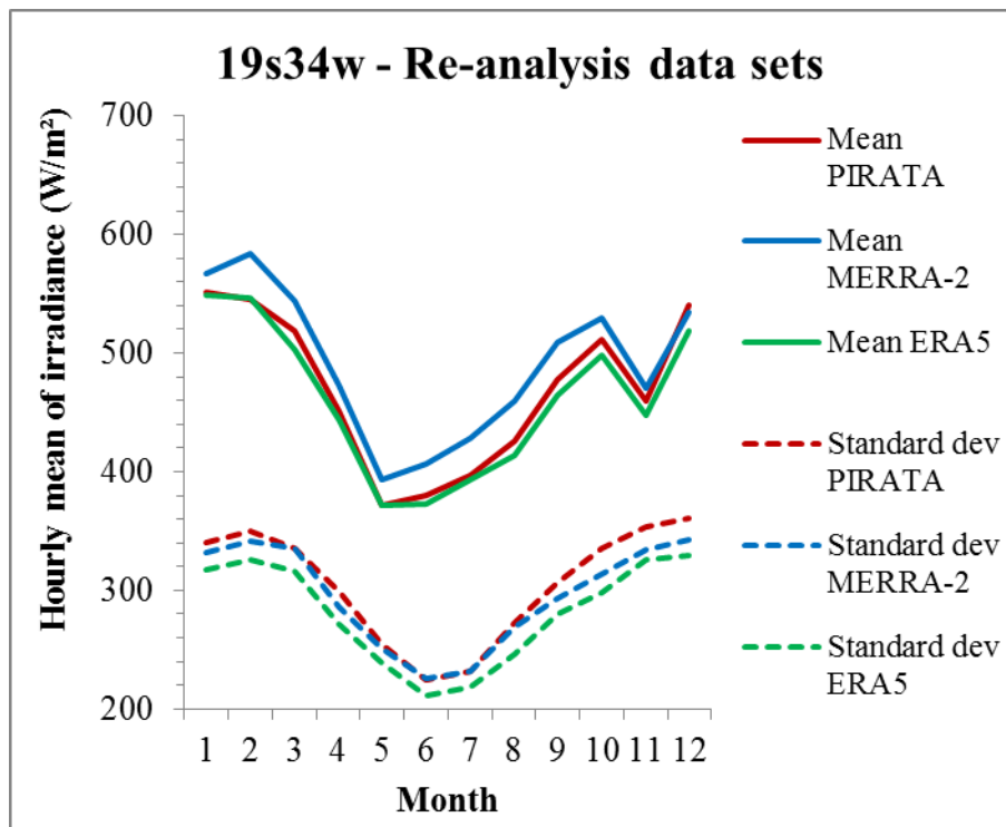
Monthly means (line) and standard deviations (dotted line) of hourly DSIS, in W\ m^{-2} , from PIRATA measurements (red) and data sets (MERRA-2: blue, ERA5: green) at 19s34w. A difference between red line (measurements) and coloured line (data set) for a given month denotes a systematic error for this month: underestimation if the coloured line is below the red line, overestimation otherwise. For a given month, a coloured dotted line above the red one means that the data set produces too much variability for this month; in the opposite case, the data set does not contain enough variability.
