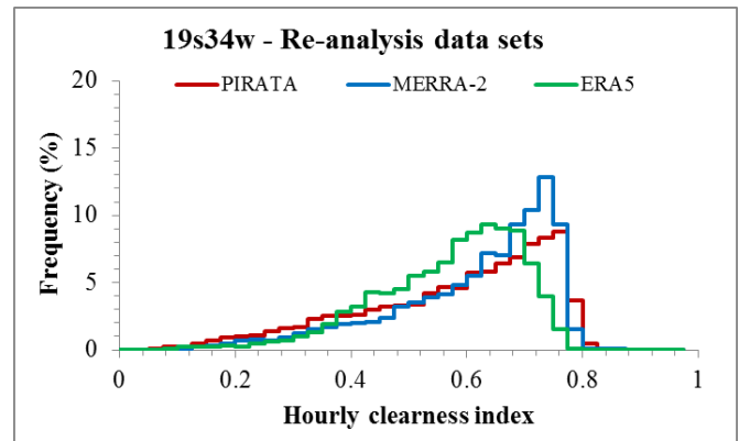
Frequency distributions of PIRATA measurements (red) and data sets (MERRA-2: blue, ERA5: green) at 19s34w for E (left) and KT (right). If the coloured line is above, respectively below, the red one for a given sub-range of values, it means that the data set produces these values too frequently, respectively too rarely with respect to the PIRATA measurements.
