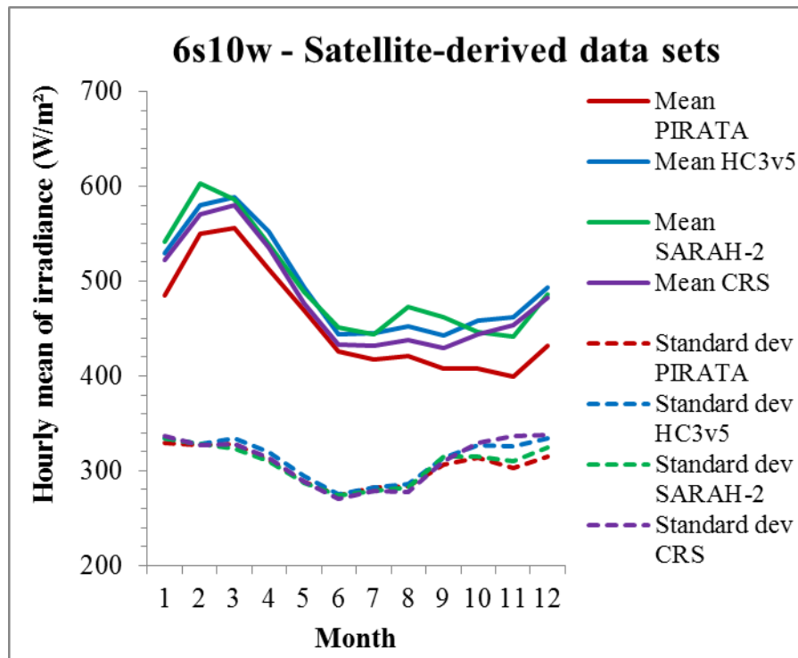
5 Figure 4: Monthly means (line) and standard deviations (dotted line) of hourly DSIS, in W m^{-2} , from PIRATA measurements (red) and data sets (HC3v5: blue; SARAH-2: green; CRS: purple) at 6s10w. A difference between red line (measurements) and coloured line (data set) for a given month denotes a systematic error for this month: underestimation if the coloured line is below the red line, overestimation otherwise. For a given month, a coloured dotted line above the red one means that the data set produces too much variability for this month; in the opposite case, the data set does not contain enough variability.
