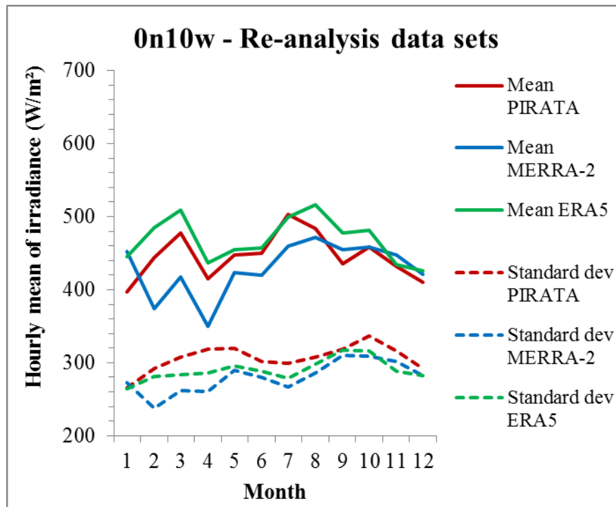
Monthly means (line) and standard deviations (dotted line) of hourly DSIS, in W m^{-2} , from PIRATA measurements (red) and data sets (MERRA-2: blue, ERA5: green) at 0n10w. A difference between red line (measurements) and coloured line (data set) for a given month denotes a systematic error for this month: underestimation if the coloured line is below the red line, overestimation otherwise. For a given month, a coloured dotted line above the red one means that the data set produces too much variability for this month; in the opposite case, the data set does not contain enough variability.
