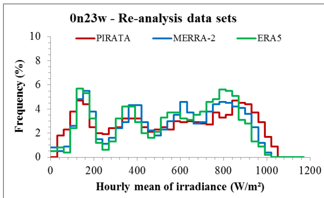
Frequency distributions of PIRATA measurements (red) and data sets (MERRA-2: blue, ERA5: green) at 0n23w for E (left) and KT (right). If the coloured line is above, respectively below, the red one for a given sub-range of values, it means that the data set produces these values too frequently, respectively too rarely with respect to the PIRATA measurements.
