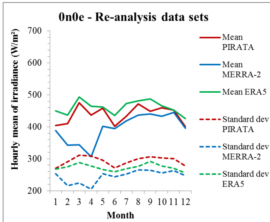
Monthly means (line) and standard deviations (dotted line) of hourly DSIS, in W\ m^{-2} , from PIRATA measurements (red) and data sets (MERRA-2: blue, ERA5: green) at 0n0e. A difference between red line (measurements) and coloured line (data set) for a given month denotes a systematic error for this month: underestimation if the coloured line is below the red line, overestimation otherwise. For a given month, a coloured dotted line above the red one means that the data set produces too much variability for this month; in the opposite case, the data set does not contain enough variability.
