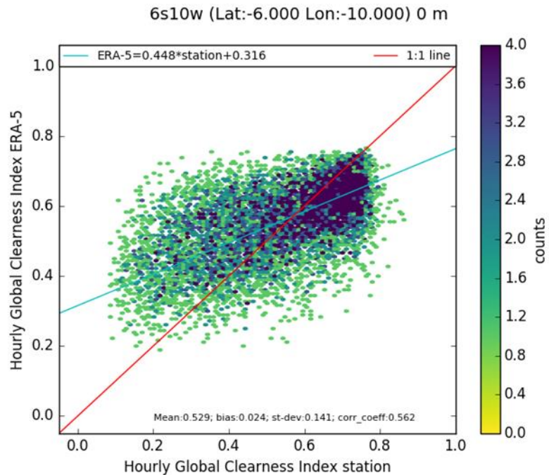
Figure 5: 2D histogram of PIRATA measurements (horizontal axis) and data sets (vertical axis) at 6s10w for E and KT . MERRA-2: (a) and (b); ERA5: (c) and (d). Ideally, the dots should lie along the red line (1:1 line). The blue line is the affine function fitted over the points and should ideally overlay the red line.
