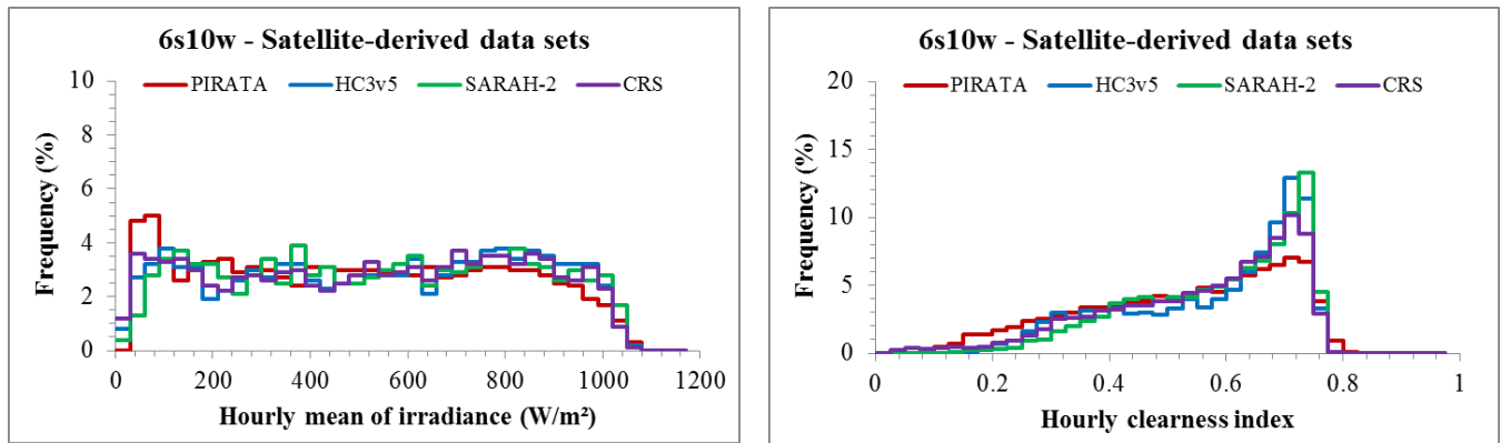
10 Figure 3: Frequency distributions of PIRATA measurements (red) and data sets (HC3v5: blue, SARAH-2: green, CRS: purple) at 6s10w for E (left) and KT (right). If the coloured line is above, respectively below, the red one for a given sub-range of values, it means that the data set produces these values too frequently, respectively too rarely with respect to the PIRATA measurements.
