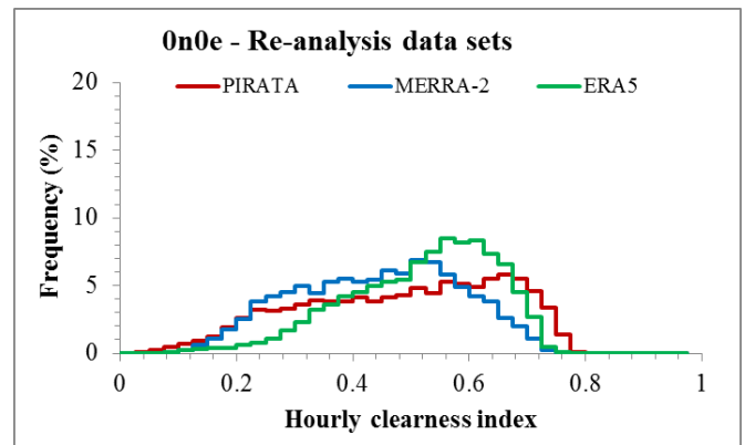
Frequency distributions of PIRATA measurements (red) and data sets (MERRA-2: blue, ERA5: green) at 0n0e for E (left) and KT (right). If the coloured line is above, respectively below, the red one for a given sub-range of values, it means that the data set produces these values too frequently, respectively too rarely with respect to the PIRATA measurements.
