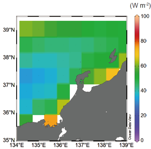
Figure 4: Temporal and spatial variations in sea surface heat flux. (a) Annual variations in sea surface heat flux ( W m^{-2} ) between 2000–2013 in the area of 134–139° E and 35–39°30' N. Vertical bars denote one standard deviation. (b) Spatial variation of sea surface heat flux ( W m^{-2} ) during spring (March–May) from 2000–2013. Blank areas were excluded because they were ascribed as landmass in JRA55.
