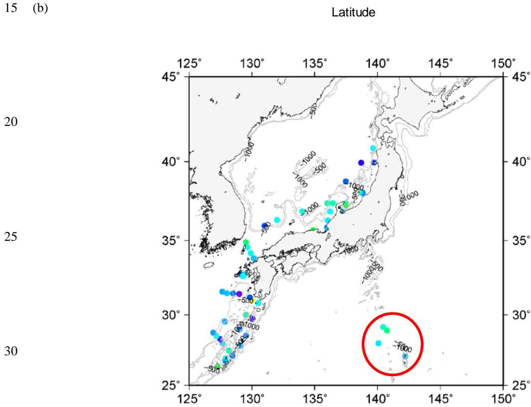
Figure 9: Latitudinal and horizontal distributions of the ^{134}\text{Cs}/^{137}\text{Cs} activity ratios measured at the coastal sites of the SOJ and ECS in 2015-2016. The values were radioactive decay corrected to 11 th March 2011. The data measured in the Ogasawara area (red circles in (a)) were also added. (a) Latitudinal distribution, (b) horizontal distribution.
