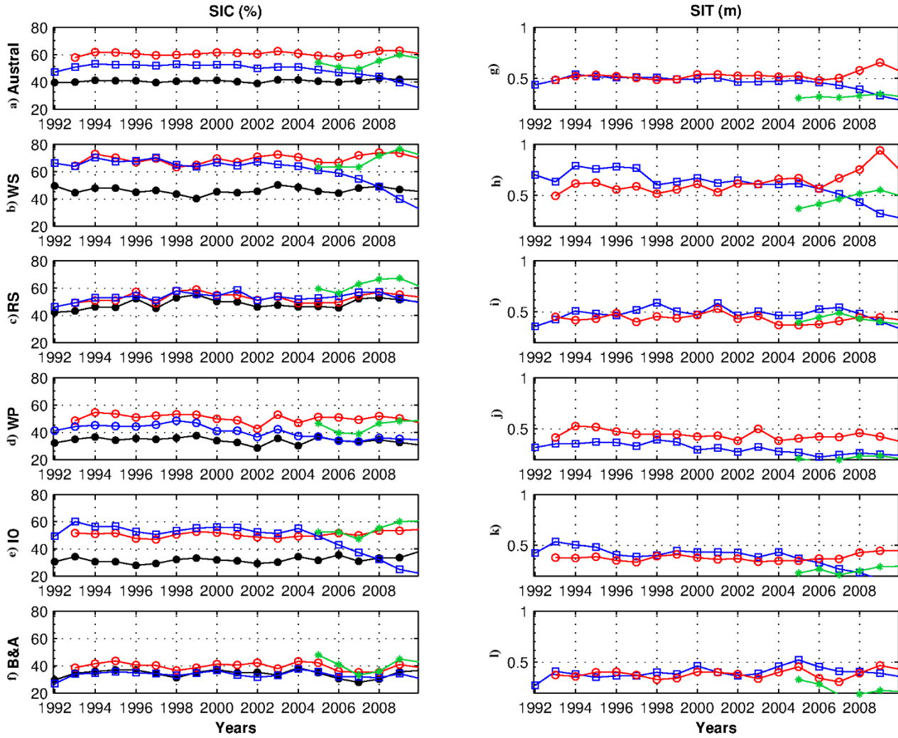
Figure 2: Annual mean Sea Ice Concentration (left) and Thickness (right) of each sector of the Southern Ocean. The red(O), green(*) and blue (□) lines are the annual mean time series from UR025.4, SoSE and ECCO2, respectively, and the circles, stars and squares are the respective annual values. The black(●) line with the filled black circles represents the mean sea ice concentration from the Goddard Satellite observations. The sectors are labeled WS (Weddell Sea), RS (Ross Sea), WP(Western Pacific), IO(Indian Ocean) and B&A (Bellingshausen and Amundsen Seas).
