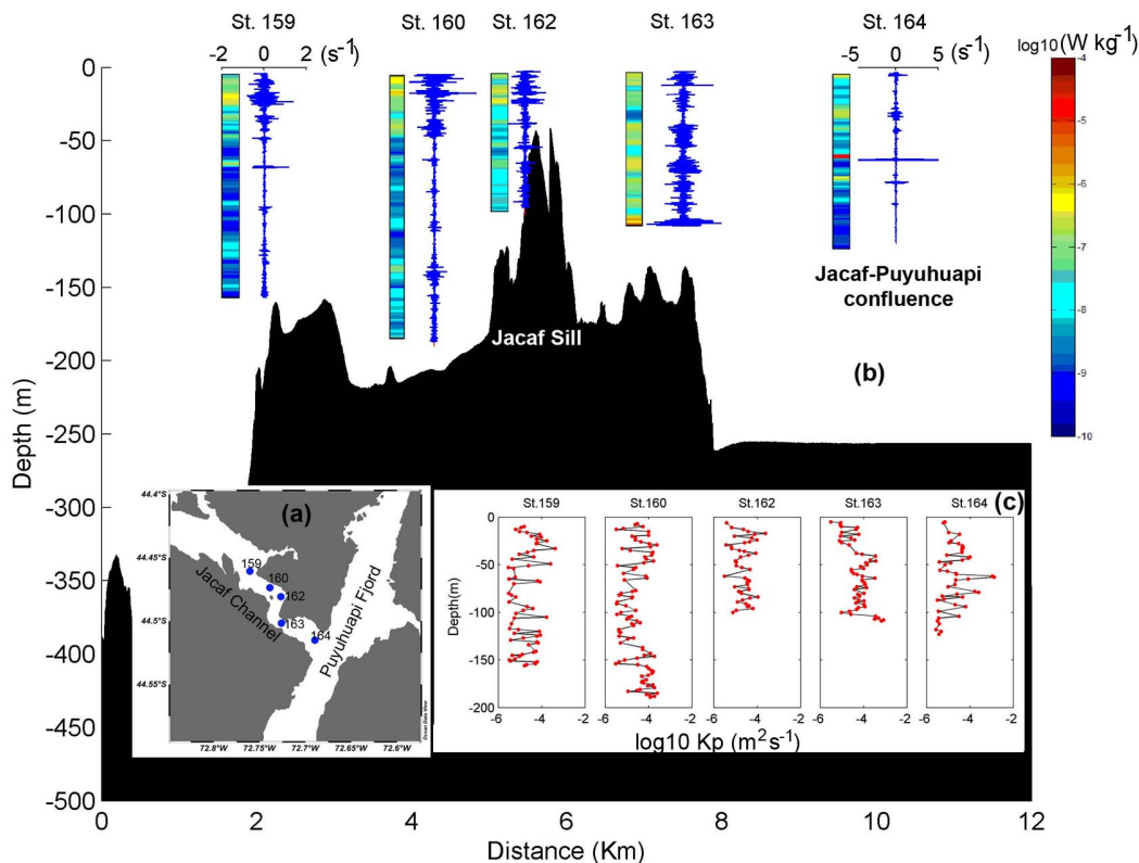
Fig. 11. (a) Microstructure profile locations along Jacaf Channel and sill using VMP-250 in November 2013. (b) The color bar showed the dissipation rate of turbulent kinetic energy ( \epsilon ) and the blue lines depi
