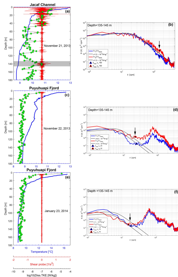
Fig. 10. Profiles of water temperature (blue line), vertical shear (red line) and dissipation rate of turbulent kinetic energy (black line with green dots) obtained with the VMP-250 microprofiler at the depth
