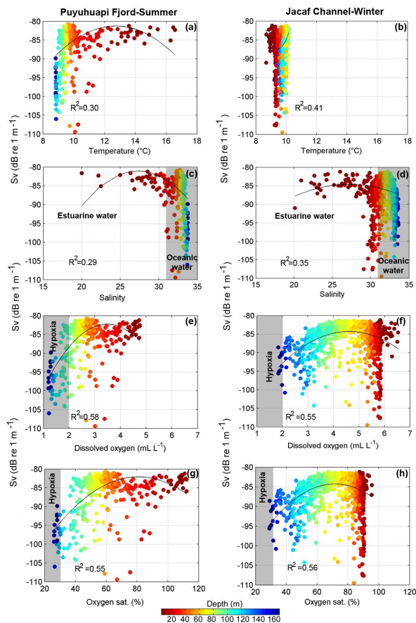
Fig. 9. Relationships between the relative abundance of zooplankton (expressed in Sv values) using 38 kHz frequency echo-sounder measurements (y-axis) and temperature in (a) Puyuhuapi Fjord and (b) Jacaf Ch
