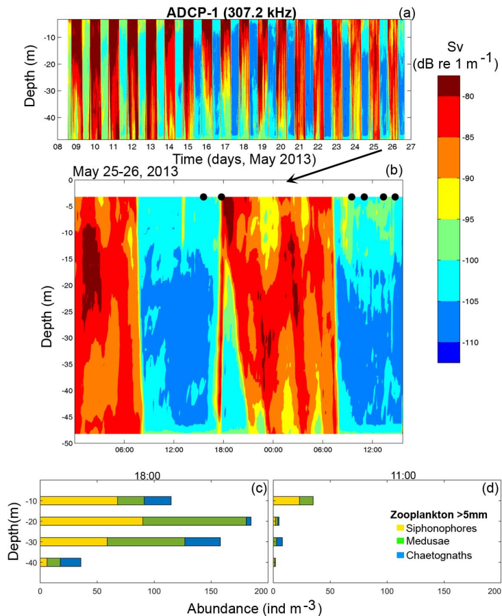
Fig. 3. (a) Volume backscattering strength (Sv v ) calculated from the ADCP-1 backscatter signal in Puyuhuapi Fjord, deployed at 50 m depth from the 8th to the 26th of May, 2013. (b) Zoom of the Sv data and the
