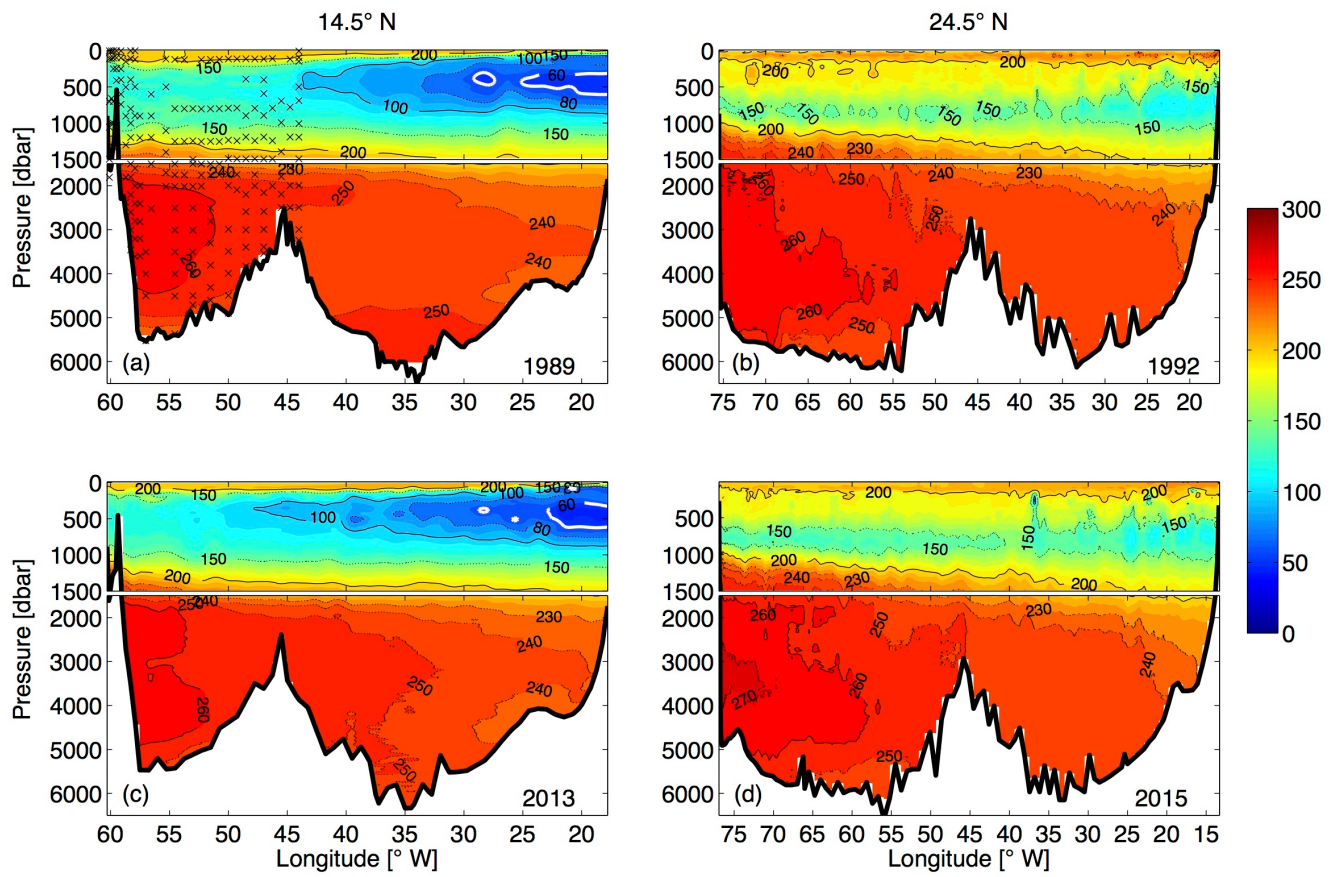
Figure 5. Vertical sections of oxygen ( \mu\text{mol kg}^{-1} ) at 14.5° N in (a) 1989 and (c) 2013; and at 24.5° N in (b) 1992 and (d) 2015. The “crosses” in (a) marks the position of bottle oxygen data, which are used to reconstruct the oxygen section in the western basin (see text for details). The white contour in (a) and (c) marks the 60 \mu\text{mol kg}^{-1} oxygen. The upper 1500 m in each subplot are stretched.
