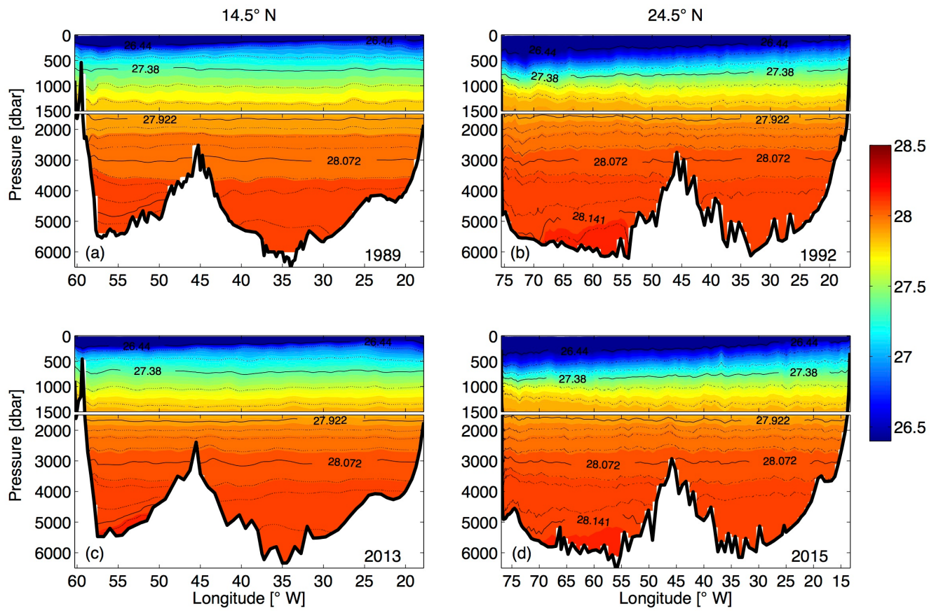
Figure 6. Vertical sections of neutral density ( \text{kg m}^{-3} ) at 14.5^\circ \text{N} in (a) 1989 and (c) 2013; and at 24.5^\circ \text{N} in (b) 1992 and (d) 2015. The upper 1500 m in each subplot are stretched.
