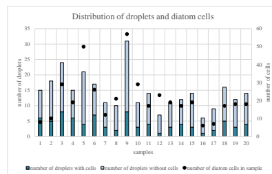
Figure 5. Number of droplets containing Nannofrustulum diatom cells, without cells and number of cells in each sample aerosolized by bubbles of D = 1.2 mm.
