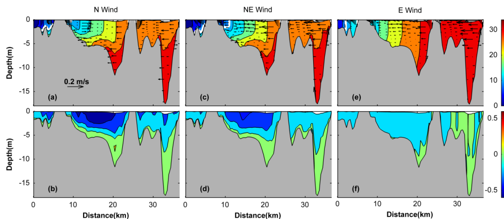
Figure 15. Comparison of 50-hour averaged salinity and current at the cross-section in the middle of the estuary (T4). The upper panel is for salinity and current, while the lower panel is for log10 of the eddy diffusivity.
