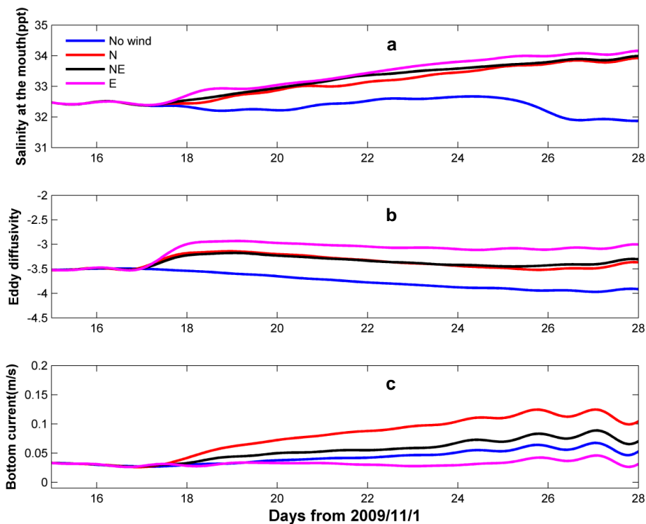
Figure 16. a) Low-pass filtered vertically-averaged salinity at the estuary mouth; b) Low-pass filtered log 10 of mean eddy diffusivity along the longitudinal transect T1; c) Low-pass filtered mean bottom current along the T1.
