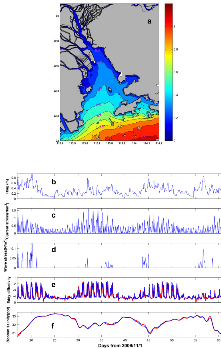
Figure 11. a) Spatial distribution of significant wave height (units: m) on Day 47; b) Time series of significant wave height at the selected station; c) Current induced bottom stress; d) Wave-induced bottom stress; e) Vertically-averaged of the logarithm (log 10 ) of eddy diffusivity without (blue solid line) and with waves (red solid line). f) Bottom salinity without (blue solid line) and with waves (red solid line).
