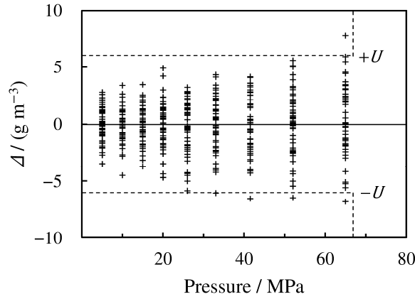
Figure 8. Residuals \Delta (measured minus the predicted values) yielded by the fit of \Delta\Delta\rho_0^{\text{SW}}(p - p_0) . U – Uncertainty in the density–salinity relation for high pressures.
