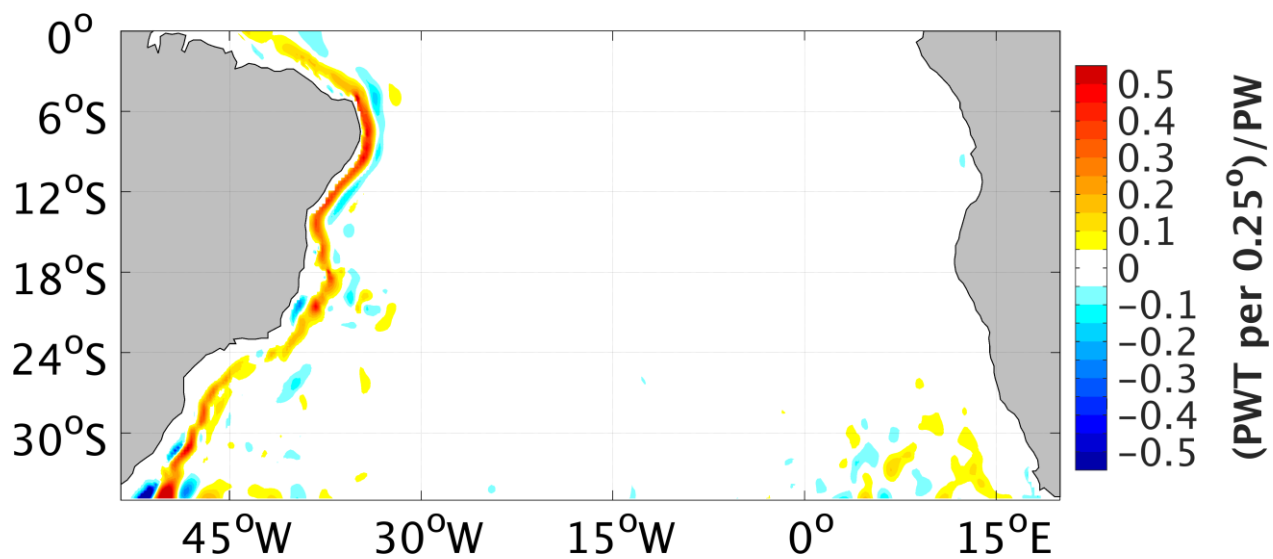
655 Figure 9. The linear regression coefficient between the inter-product p-OTTs and their MHTs for each latitude. Units are in PWT per 0.25° per 1 PW across each latitude.
