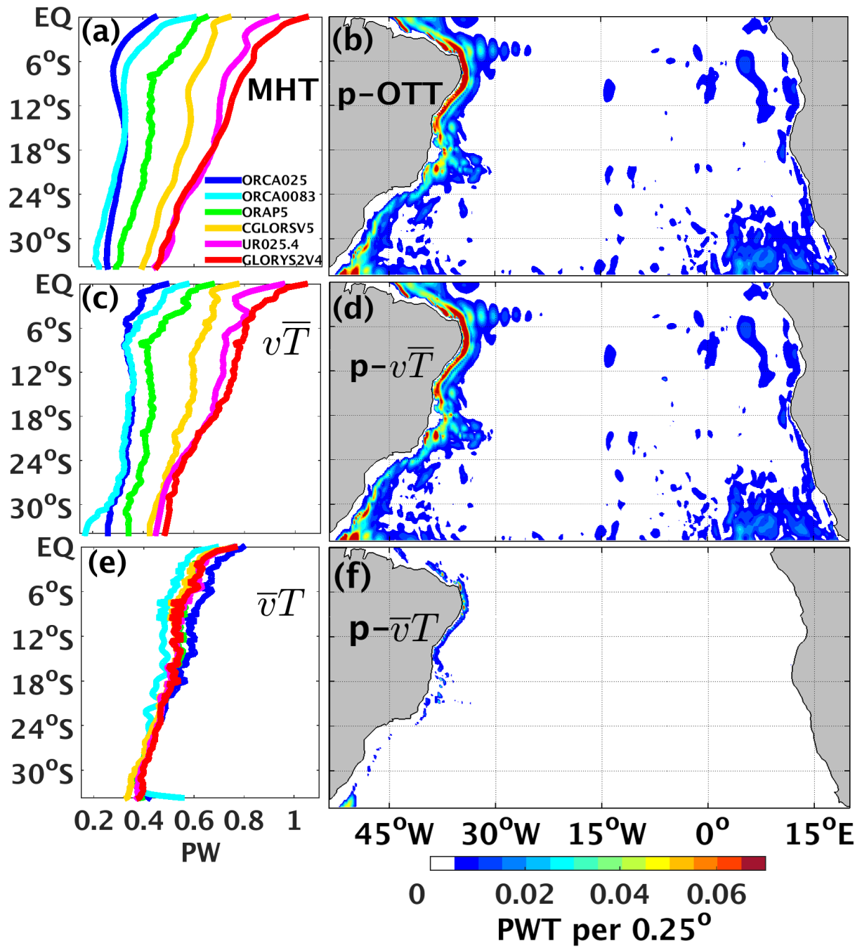
635 Figure 7. (Left) The original MHTs (a), the MHTs based on the v\bar{T} component (c), and the MHTs based on the \bar{v}T component (e) in PW. (Right) The ENS-ALL spread of the p-OTTs (b), p- v\bar{T} (d) and p- \bar{v}T (f) in PW per 0.25°. Overbar represents the mean of the ENS-ALL.
