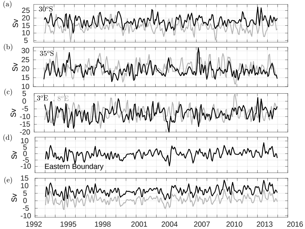
Figure 5. Time series of transports in the upper 800 m. (a) meridional transport of the Benguela Current at 30^{\circ}\text{S} (black - across line AB; gray across line A'B, see Figure 2). (b) meridional transport of the Benguela Current at 35^{\circ}\text{S} (across line CD in black; across line C'D in gray). (c) zonal transport at 3^{\circ}\text{E} (across line AC; across A'C'). (d) Cross-shelf transport at the eastern boundary near the African coast across 1000 m isobath (across line BD). (e) Transport imbalance for ABCD (black) and A'BC'D (gray).
