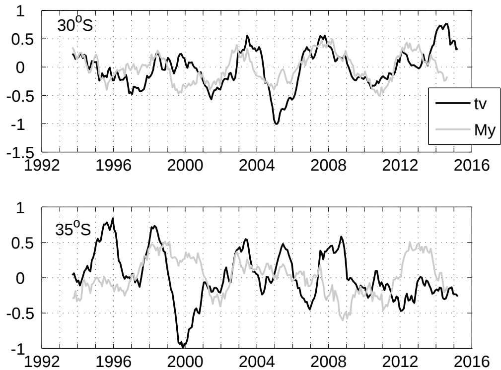
Figure 10. Zonally integrated normalized anomalies M_y (gray) and meridional transport (tv, black) at 30°S and 35°S. Both the time series are smoothed using a 18-month running mean filter.
