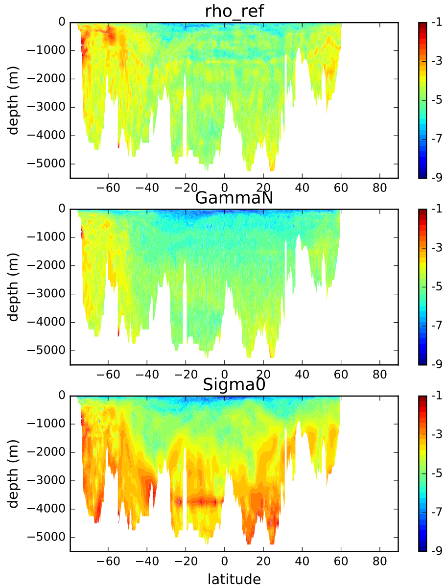
Figure 5. Decimal logarithm of the sine between the neutral vector and the gradient of \rho_{ref} (top), \gamma^n (middle) and \sigma_0 (bottom) as a function of latitude and depth at 30^\circ\text{W} (in the Atlantic).
