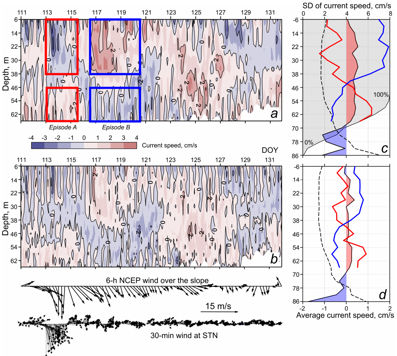
450 Figure 4. The temporal evolution of 2-h mean (a) zonal and (b) meridional velocities (cm/s) recorded between 21 April, 00:00h and 11 May, 21:00h with (c,d) their mean (solid black lines) and standard deviations (dashed black lines). Red and blue shading corresponds to positive and negative velocities, respectively. The red and blue lines correspond to mean velocities measured during episode A and B, respectively. The grey shading in (c) shows the percentage of “good” current records. Blank areas in (a) and (b) mask the records with less than 50% of good data in daily records. The lower panel demonstrates (top) the 6-h NCEP wind over 455 continental slope at 82.5°N, 10.0°W and (bottom) 30-min wind measured at Station Nord.
