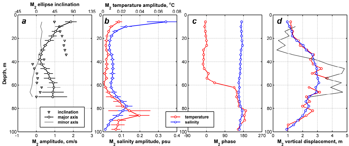
490 Figure 9. (a) Vertical distribution of the lunar semidiurnal ( M_2 ) tidal ellipse parameters at the mooring position. Horizontal bars indicate the 95% confidence interval for major axis amplitude. (b) The tidal ( M_2 ) amplitude of temperature (red) and salinity (blue) and the corresponding 95% confidence intervals. (c) The M_2 phases of temperature and salinity. (d) The vertical displacement (m) of water parcel estimated as a ratio of M_2 tidal amplitude of temperature/salinity (red/blue) to the vertical gradients of temperature/salinity estimated from the mean vertical profiles in Figure 5a and 5b. Dotted black line shows the vertical displacements estimated from lunar semidiurnal component of vertical velocity.
