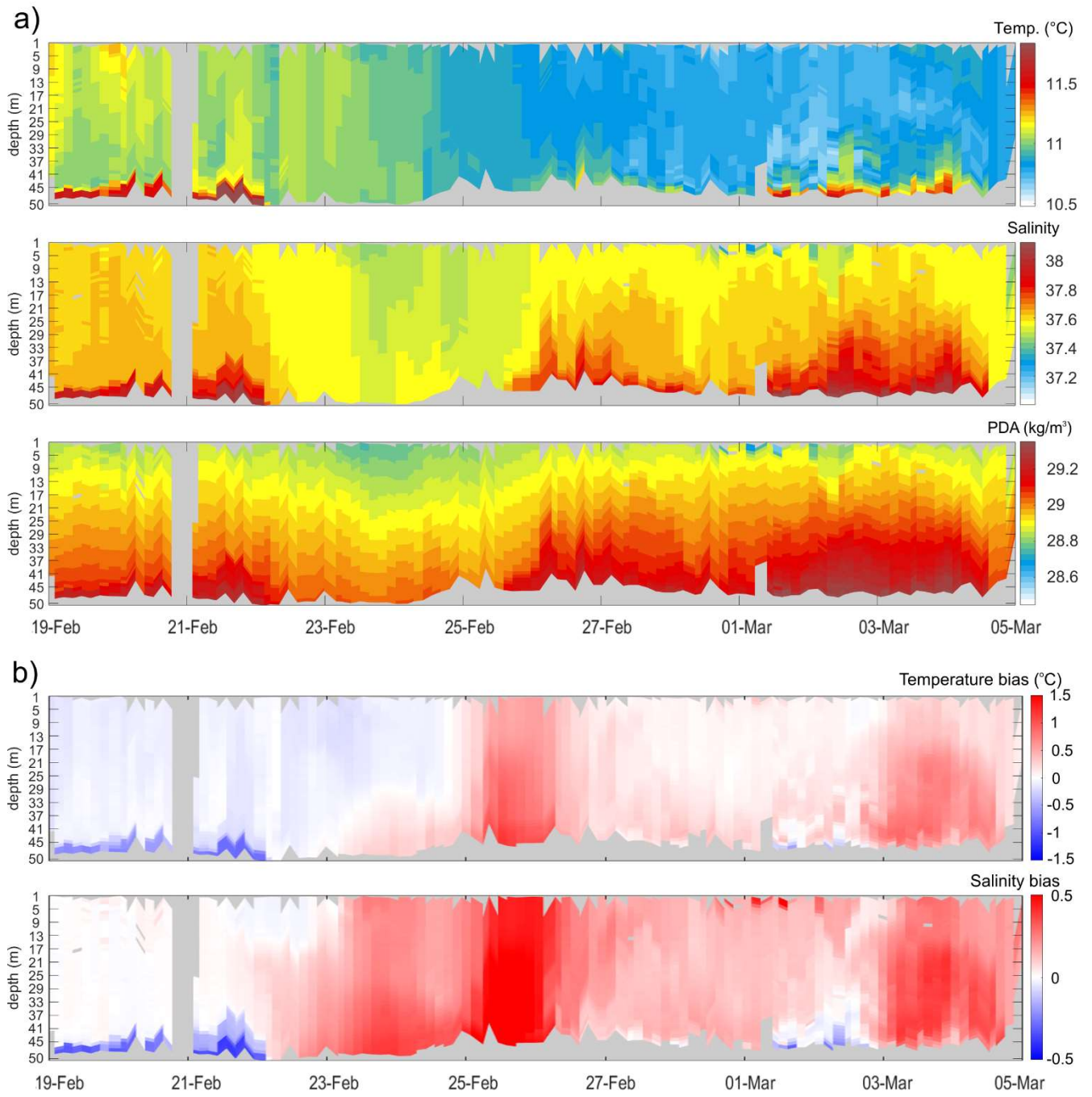
Figure 6. (a) Temperature, salinity and PDA values measured between 19 February and 5 March 2015 by Arvor-C profiling float in the Kvarner Bay, together with (b) model-to-observation difference (bias). Profiling float trajectory is plotted in Fig. 1.
