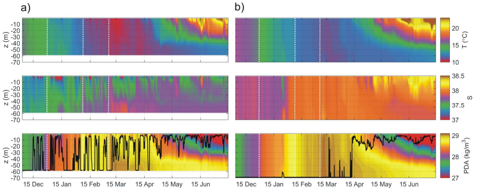
Figure 10. Hovmöller plot of modeled temperature, salinity and PDA values at grid points (a) G1 and (b) G2. Vertical dashed lines indicate three severe bora episodes discussed in Section 3, while thick black line in PDA plot shows mixed layer depth.
