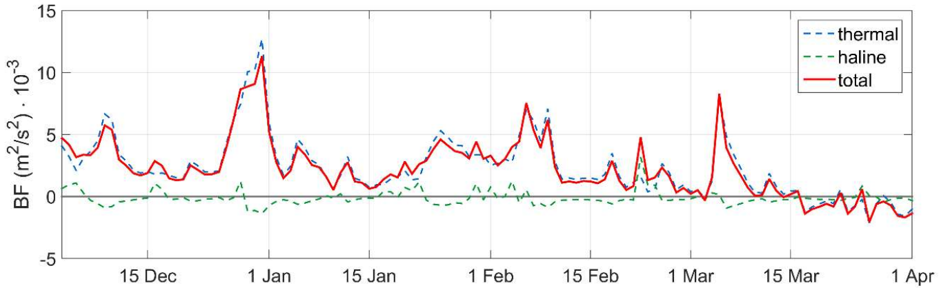
Figure 11. Daily values of surface buoyancy fluxes (BF) and its components averaged over the nested model domain.
