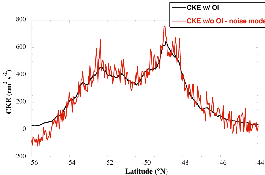
Fig. 2. CKE averaged from 1993-2016 along a part of a satellite pass in the Southern Ocean for SSH anomalies that have been optimally interpolated (black line) and from the raw SSH anomalies with no filtering
