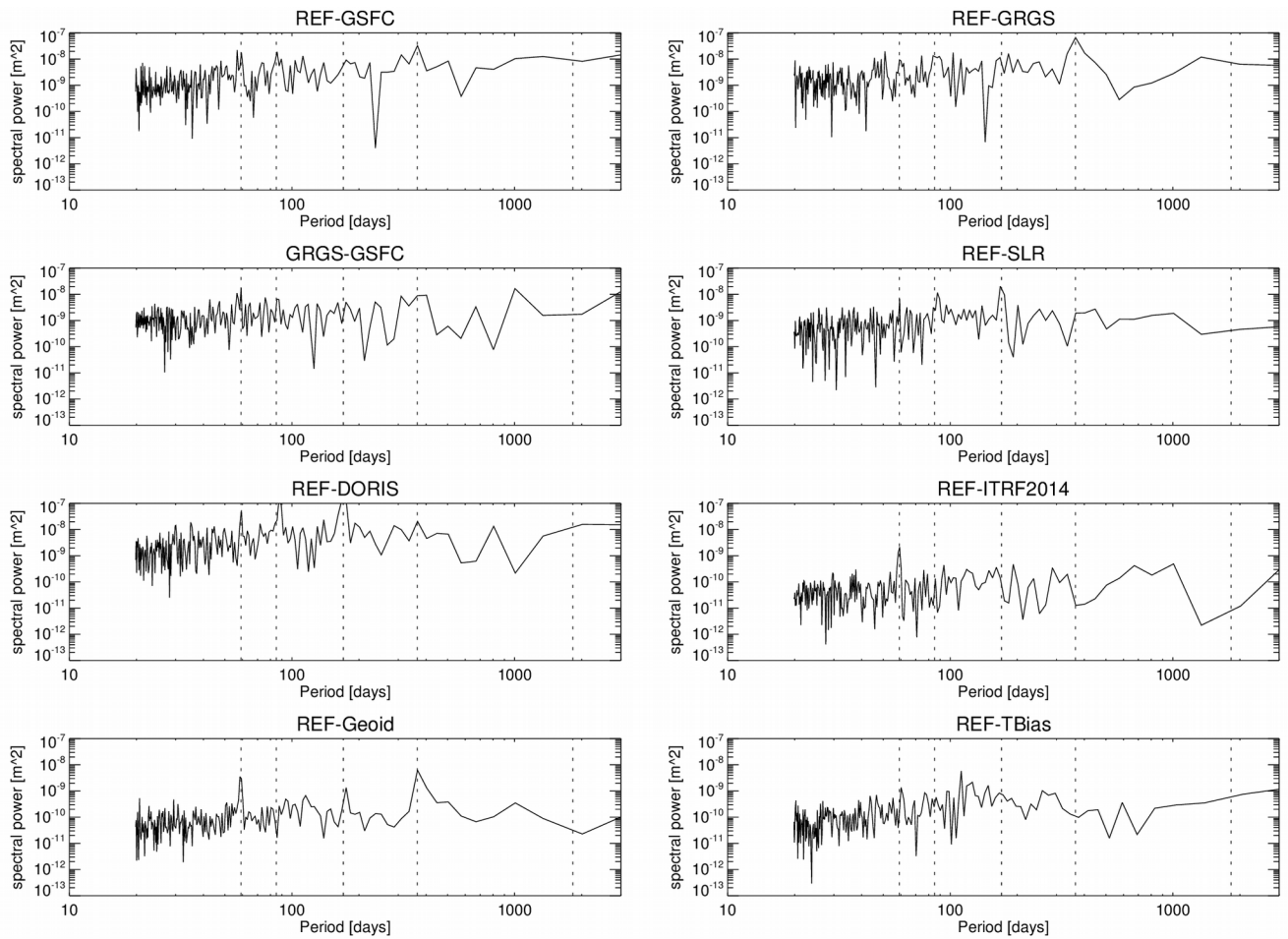
Figure S2: Power spectra of the global mean radial orbit differences over the oceans for REF minus GSFC , REF minus GRGS , GRGS minus GSFC , REF minus SLR , REF minus DORIS , REF minus ITRF14 , REF minus Geoid , and REF minus TBias . Vertical dashed lines mark periods of 59, 85, 170 days, 1 and 5 years.
