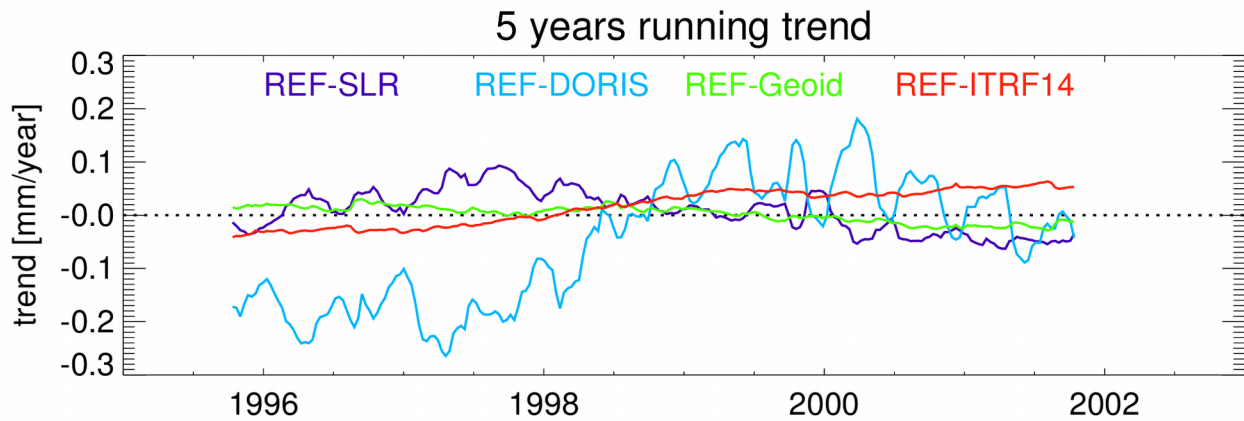
675 Figure 4: 5-year running trends for the global mean radial orbit differences over the oceans for REF minus GSFC (dark blue), REF minus GRGS (light blue), and GRGS minus GSFC (green) on the top; for REF minus SLR (dark blue), REF minus DORIS (light blue), REF minus Geoid (green), and REF minus ITRF14 (red) on the bottom. Trend values are given for the central time of the corresponding running window.
