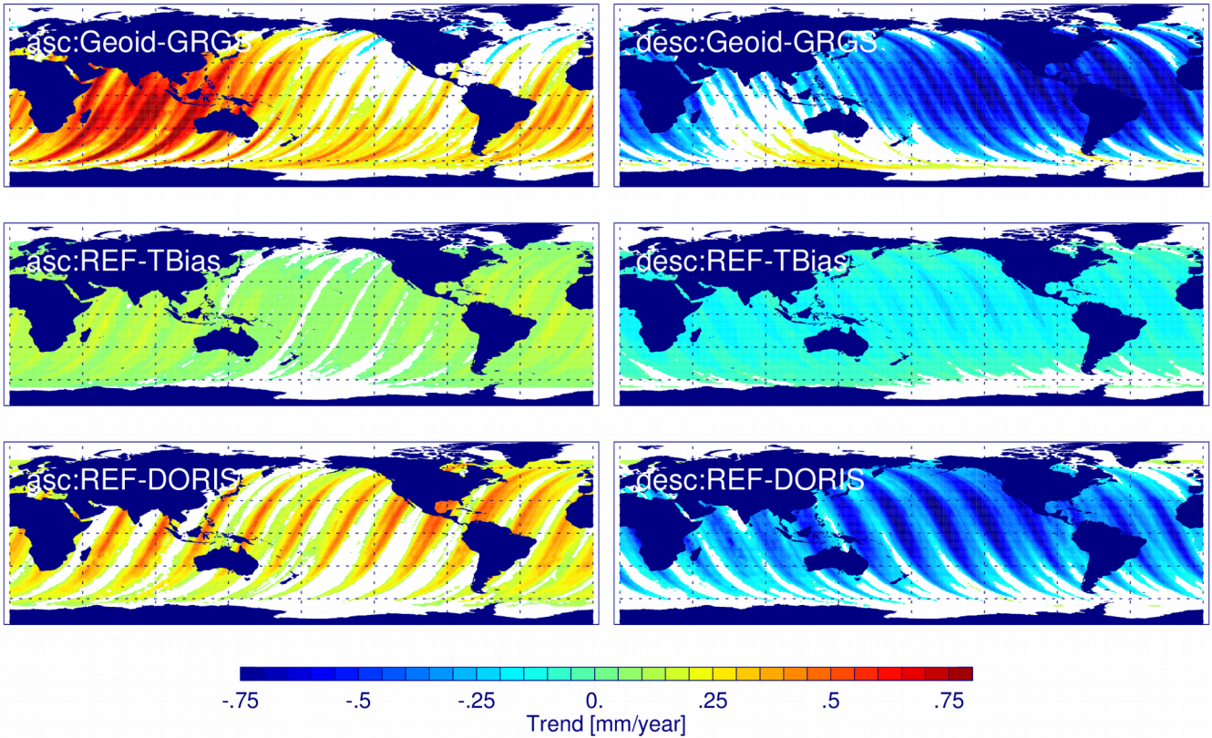
Figure 8: Decadal trend differences of radial orbit components for ascending (left) and descending (right) passes for Geoid minus GRGS REF minus TBias , and REF minus DORIS for the period April 1993 – June 2004. Regions with formal errors larger than the fitted value are masked out (white). The global mean trend difference over the ocean is given in Table 6.
