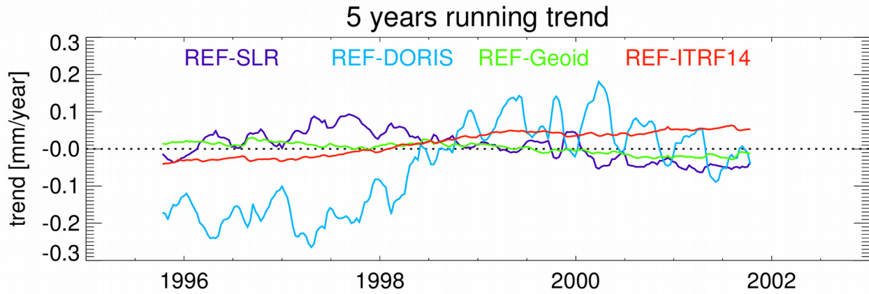
695 Figure 4: 5-year running trends for the global mean radial orbit differences over the oceans for REF minus GSFC (dark blue), REF minus GRGS (light blue), and GRGS minus GSFC (green) on the top; for REF minus SLR (dark blue), REF minus DORIS (light blue), REF minus Geoid (green), and REF minus ITRF14 (red) on the bottom. Trend values are given for the central time of the corresponding running window.
