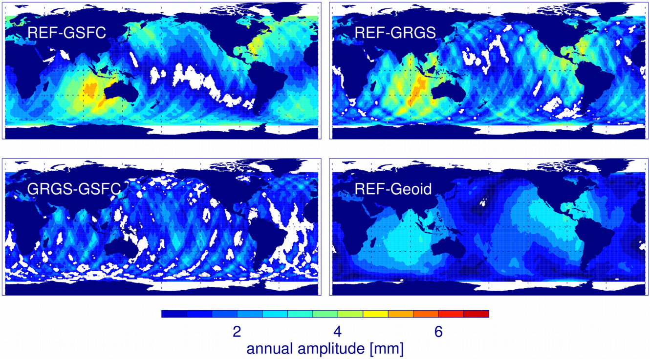
705 Figure 5: Annual amplitude of the radial orbit differences for REF minus GSFC , REF minus GRGS , GRGS minus GSFC , and REF 710 minus Geoid . The regions with formal errors larger than the fitted value are masked out (white). The maximum amplitude 715 difference is given in Table 5.
