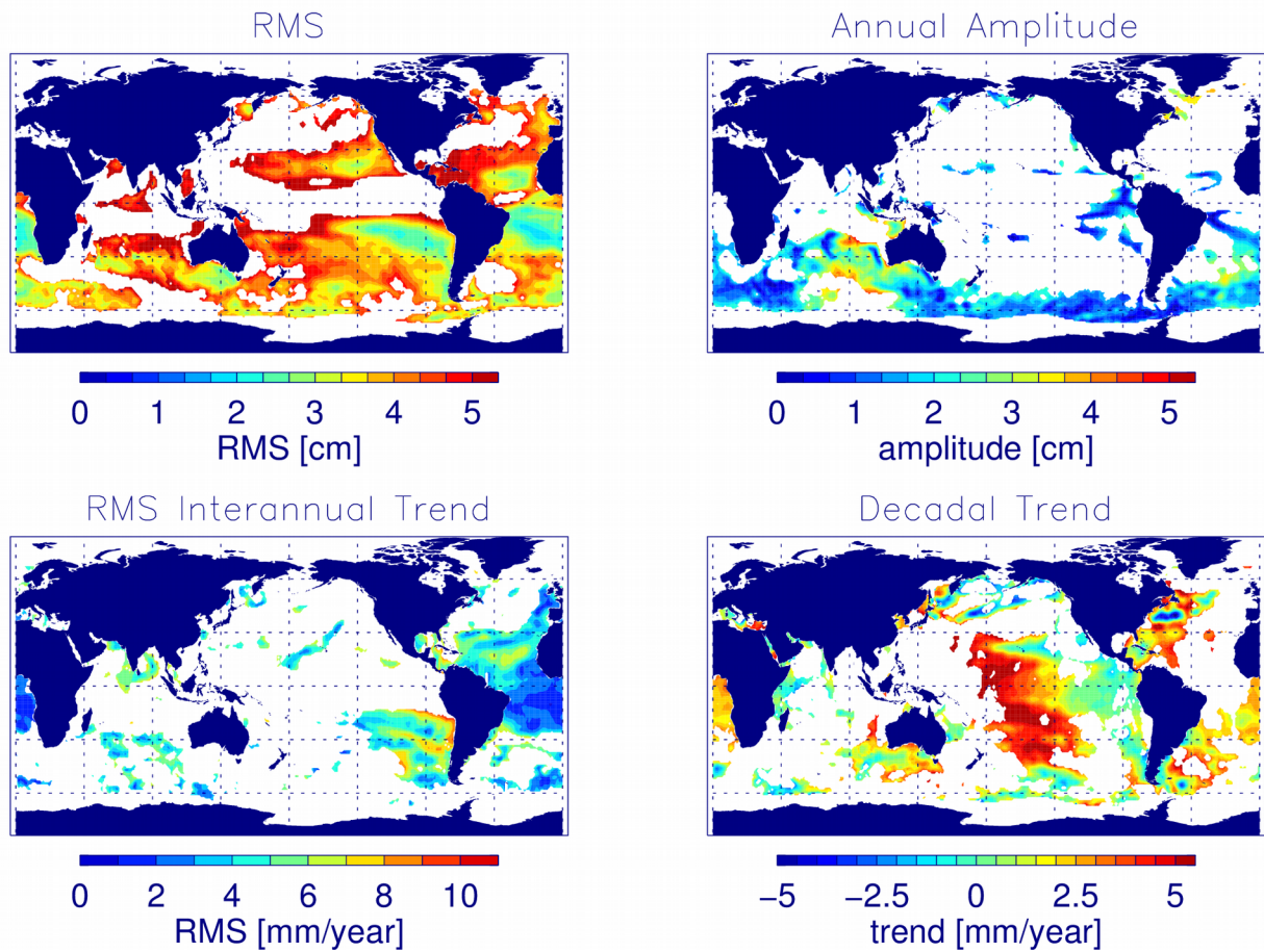
755 Figure 9: RMS of sea level, annual amplitude, RMS of interannual (5 years) running trend, and decadal trends from TOPEX altimeter data for the period February 1993– October 2005. Colour coded are sea level values for which the local orbit errors (estimated from GFZ minus GRGS ) reach more than 10 % of the local sea level values. All other regions are masked out (white).
