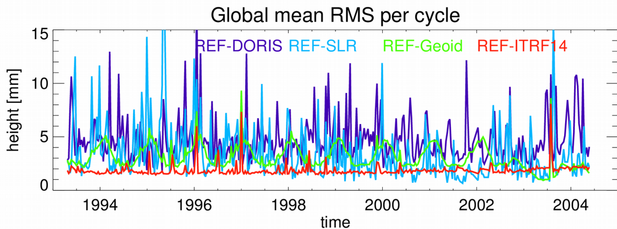
685 Figure 3: Time series of the global mean RMS per cycle of gridded radial orbit differences for REF minus GSFC (dark blue), and REF minus GRGS (red) on the top; for REF minus DORIS (dark blue), REF minus SLR (light blue), REF minus Geoid (green), and REF minus ITRF14 (red) on the bottom.
