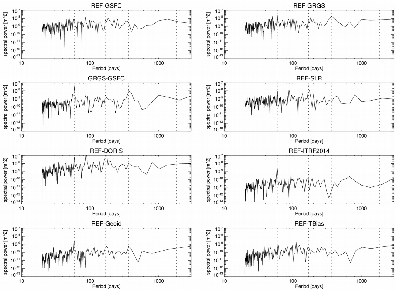
815 Figure S2: Power spectra of the global mean radial orbit differences for REF minus GSFC , REF minus GRGS , GRGS minus GSFC , REF minus SLR , REF minus DORIS , REF minus ITRF14 , REF minus Geoid , and REF minus TBias . Vertical dashed lines mark periods of 59, 85, 170 days, 1 and 5 years.
