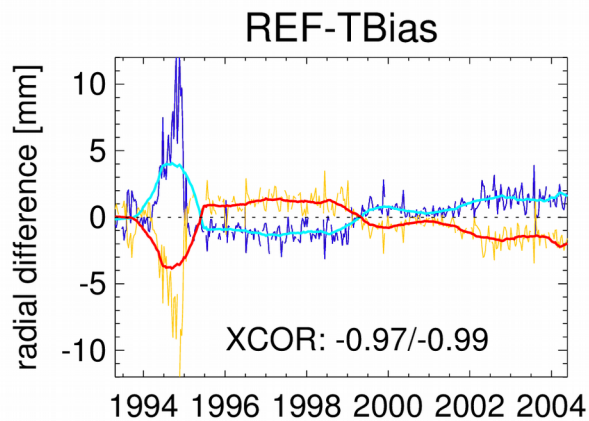
Figure S3: Global mean radial orbit differences per cycle for Geoid minus GRGS , REF minus DORIS , and REF minus Tbias separately for ascending (blue, cyan) and descending (yellow, red) tracks and 1-year box-car filtered. The cross-correlation coefficient between the ascending and descending passes for the original and the filtered series is given at the lower part of each graph.
