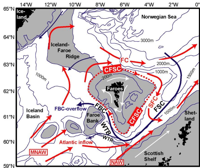
Figure 1. Bathymetry of the Faroe Channels, including schematic arrows of flow pathways. Gray areas are shallower than 500 m. Continuous arrows indicate well-established flows of: cold overflow water at depth (blue arrows), warm Atlantic inflow as North Atlantic Water (NAW) and as Modified North Atlantic Water (MNAW) in the upper layers off the shelves (red arrows), and shelf water (white arrows). Dashed red arrows indicate the hypothetical Circum-Faroe Slope Current (CFSC). FSC = Faroe-Shetland Channel, FBC = Faroe Bank Channel, WTB = Wyville Thomson Basin, WTR = Wyville Thomson Ridge, FC = Faroe Current, SFC = Southern Faroe Current.
