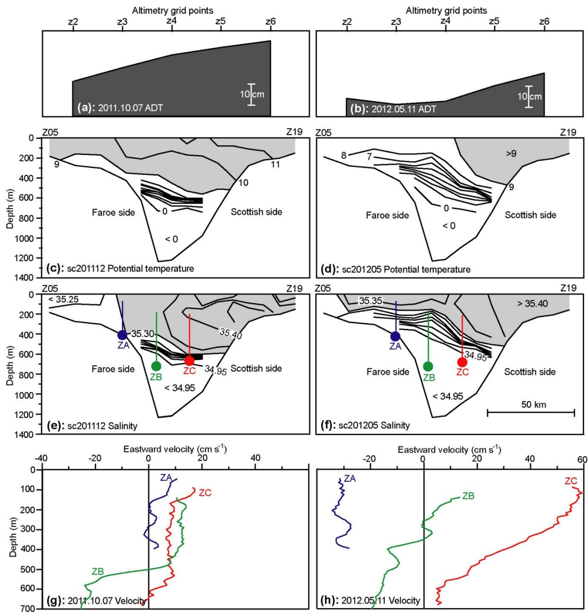
Figure 6. Conditions on the Z-section during two different cruises by MRV Scotia: Cruise sc201112 on 7–8 Oct. 2011 ( a , c , e , g ), and cruise sc201205 on 10–12 May 2012 ( b , d , f , h ). ( a , b ) Absolute Dynamic Topography (ADT). ( c , d ) Potential temperature distribution (in °C, contouring interval: 1 °C). Gray areas indicate water warmer than 9 °C. ( e , f ) Salinity distribution (contouring interval: 0.05). Gray areas indicate water more saline than 35.30. ( g , h ) Eastward component of ADCP velocity profiles (ADCP locations indicated on panels e and f ). Panels a , b , g , and h are for dates in the middle of each cruise but would not look significantly different for other days within the cruise periods.
