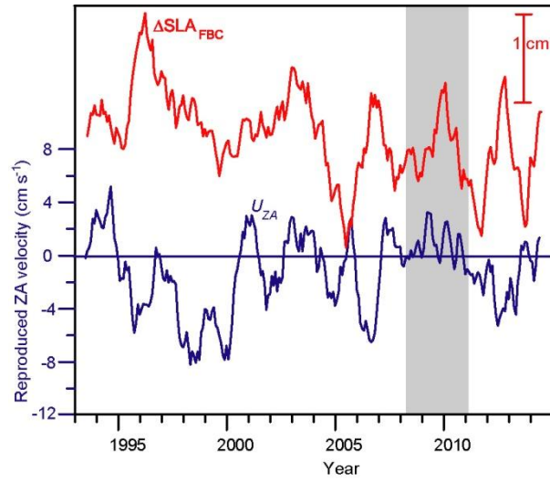
Figure 5. Annually (13 months) filtered values of: reproduced eastward velocity at 200 m at ZA ( U_{ZA} , blue) and difference in SLA-values between f1 and f2 ( f2-f1 : \Delta SLA_{FBC} , red). The gray area indicates the period of ferry-based ADCP measurements by Rossby and Flagg (2012).
