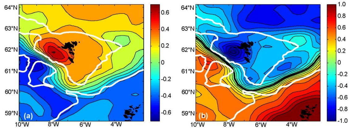
Figure 9. Relationships between Atlantic water transport through the Faroe Bank Channel and altimetry values in the region. (a) Correlation coefficient between \Delta SLA_{FBC} and SLA^* in all grid points of the region. (b) Negative value of the regression coefficient (slope) of SLA^* in all grid points regressed on \Delta SLA_{FBC} , where the zero value is indicated by a thick black line. The thick white lines indicate the 500 m bottom contour. Based on weekly averages.
