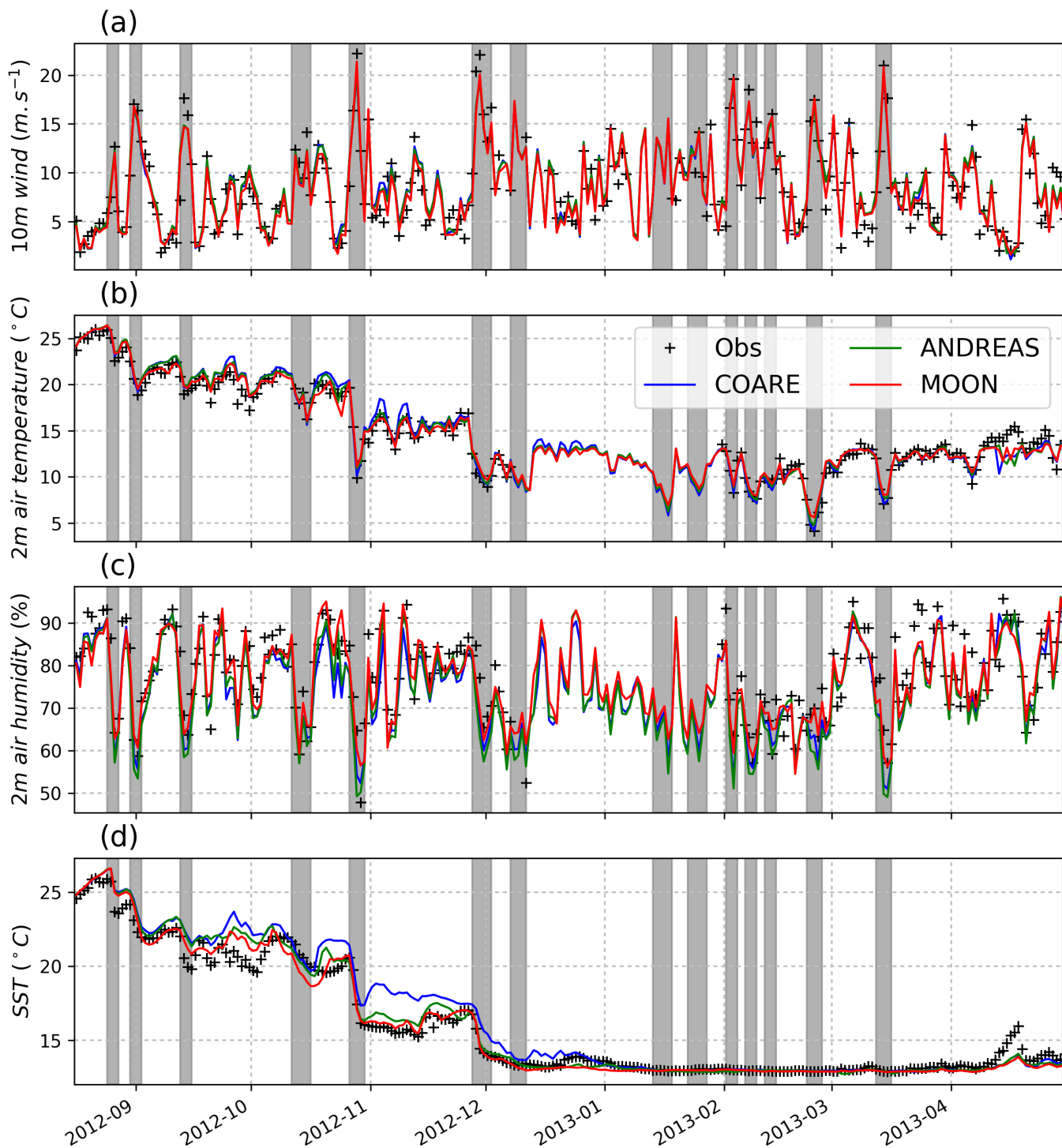
Figure 4. Time series of (a) the 10 m wind speed (b) the 2 m air temperature (c) the 2 m air humidity and (d) the sea surface temperature measured at the Lion meteorological buoy (in black) and computed by each simulation (COARE in blue, ANDREAS in green and MOON in red). The grey bars correspond to the strong wind periods (hourly wind speed > 15 \text{ m s}^{-1} )
