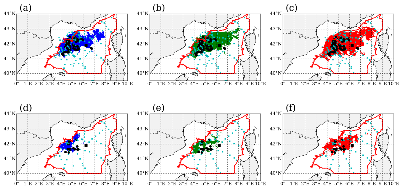
Figure 10. Coloured areas: extend of mixed patch zone computed for each simulation: (left) COARE, (middle) ANDREAS, (right) MOON. The mixed patch is defined as the area where the stratification index, (a-c) at 1000 m and (d-f) at 2000 m, reaches 0 during simulation. Black squares correspond to the position of the CTD and ARGO mixed profiles: (a-c) SI(1000) = 0 . and (d-f) SI(2000) = 0 . Cyan points show the position of the CTD and ARGO stratified profiles: (a-c) SI(1000) > 0 . and (d-f) SI(2000) > 0 . Red line: Convective area defined in section 3.
