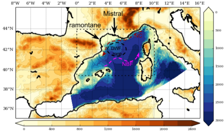
Figure 1. Full frame: spatial extension of the atmospheric model. Topography (metres, horizontal colour bar, positive above sea level) and bathymetry (metres, vertical colour bar, negative below sea level) of the ocean model. The black dotted rectangle indicates the area studied. The red and magenta dotted line represent oceanic surface circulation with the Northern Current (NC) and North Balearic Front (NBF), respectively. The black dotted circle indicates the Dense Water Formation (DWF) zone
