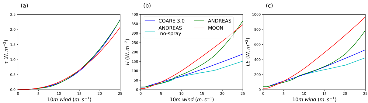
Figure 2. Turbulent fluxes of momentum (a), sensible heat (b) and latent heat (c) as functions of the surface wind speed for each bulk parameterization (COARE 3.0 in blue, ANDREAS no-spray in cyan, ANDREAS in green and MOON in red). The computation was performed with SURFEX offline, with the air surface temperature fixed at 10 °C, the sea surface temperature at 15 °C, the relative humidity at 70 %, and the surface atmospheric pressure at 1013 hPa.
