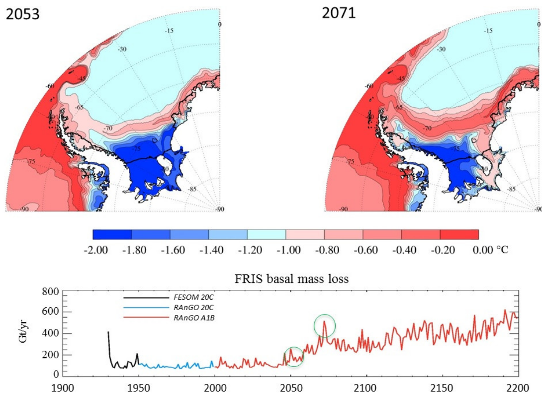
Figure 8. Top: Simulated bottom temperature for 2053 and 2071 in the RAnGO A1B experiment. The lower panel indicates the corresponding points in time on the time series of annual-mean basal mass loss.
