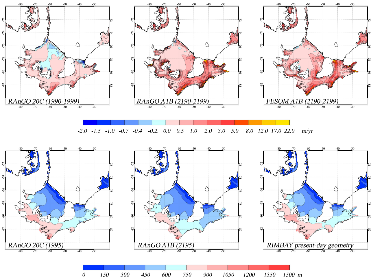
Figure 7. Top: 10-yr mean basal melt rates in the RAnGO 20C experiment for 1990-1999 (left), in RAnGO A1B for 2190-2199 (middle), and in FESOM A1B for 2190-2199 (right). Bottom: Corresponding ice-shelf drafts from the RAnGO 20C/A1B simulation for 1995 (left) and 2195 (middle), and in the RIMBAY present-day geometry. Coloured areas represent modelled cavity geometries. Black lines denote coast and grounding lines from RTopo-2.
