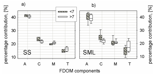
Figure 7. Dependence of percentage contribution of the main FDOM components as the box plots for (a) the sub-surface water, SS and (b) the sea surface microlayer, SML; for the coastal waters (salinity <7) and open sea (salinity >7).
