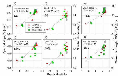
Figure 3. The relationship between salinity and: (a) the spectral slope coefficient, S_0 , measured in the 200–600nm, (b) the slope ratio S_R = S_{200-250} / S_{500-600} and (c) the relative changes in the molecular weight, MW ( E_2/E_3 ) for SS; and: (d), (e) and (f) for SML, respectively.
