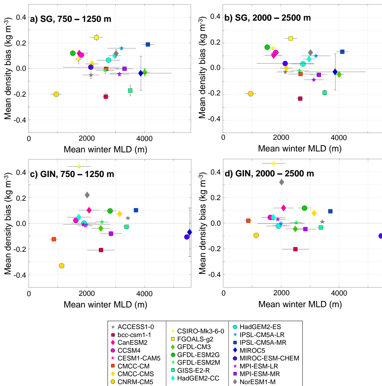
Figure 2. Across-model relationship between the 20-year mean density bias at the two depth levels representative of NADW (columns) and the 20-year mean winter MLD, in the subpolar gyre SG (top) and the GIN seas (bottom).
