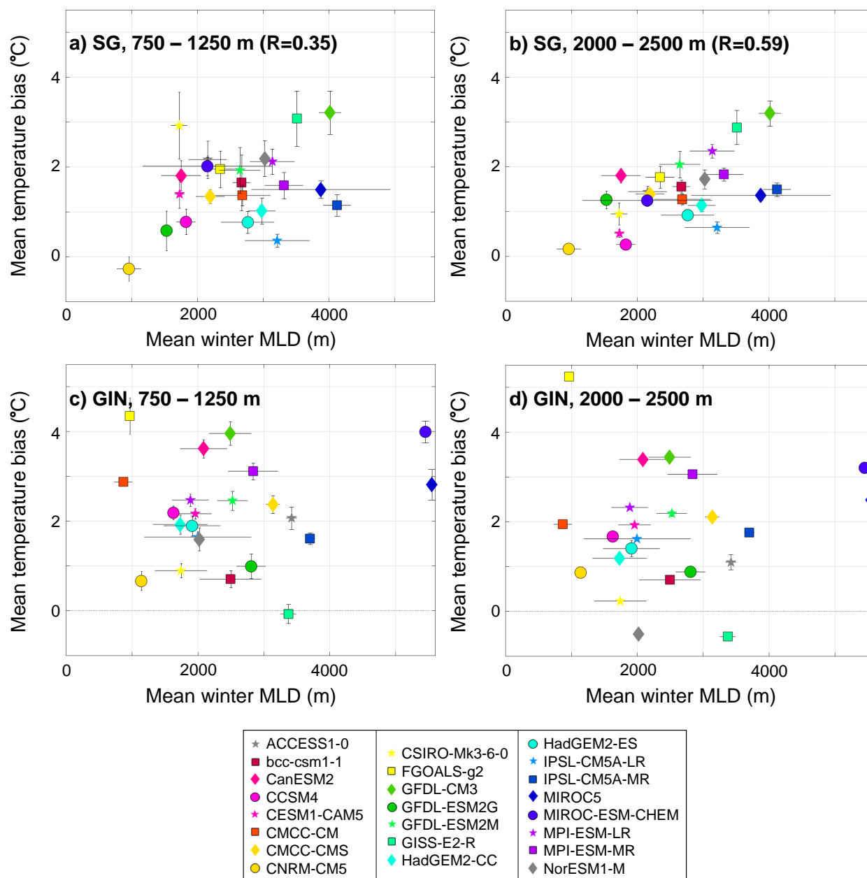
Figure 3. Across-model relationship between the 20-year mean temperature bias at the two depth levels representative of NADW (columns) and the 20-year mean winter MLD, in the subpolar gyre SG (top) and the GIN seas (bottom).
