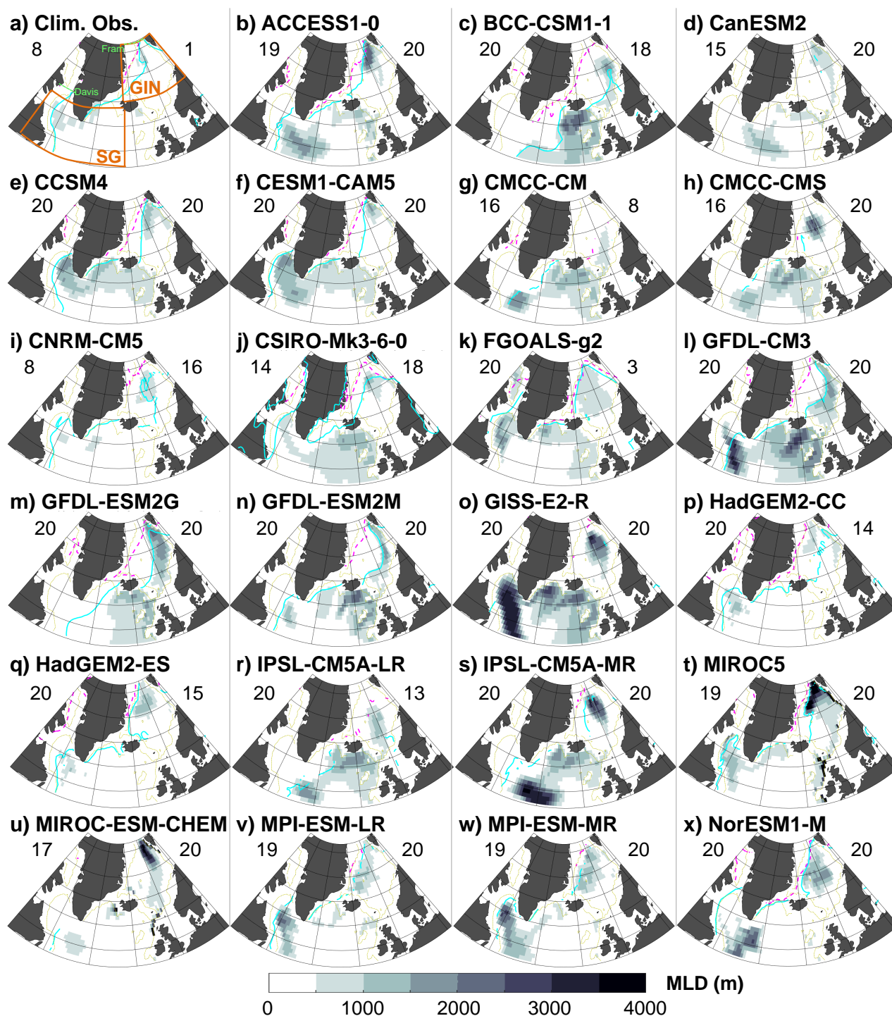
Figure 1. North Atlantic, a) climatological mixed layer depth of de Boyer Montégut et al. (2004); b to x) mean 1986-2005 winter MLD in the CMIP5 historical run. Orange boxes on a) show the subpolar gyre (SG) and Greenland-Iceland-Norwegian seas (GIN) regions as defined in this study; green dashed lines, Davis and Fram straits. Yellow dotted line on each panel indicates the 1000 m isobath; cyan and magenta lines, the mean March and September sea ice extent respectively. Left number is the number of years, out of 20, with deep convection in SG; right number, deep convection in GIN.
