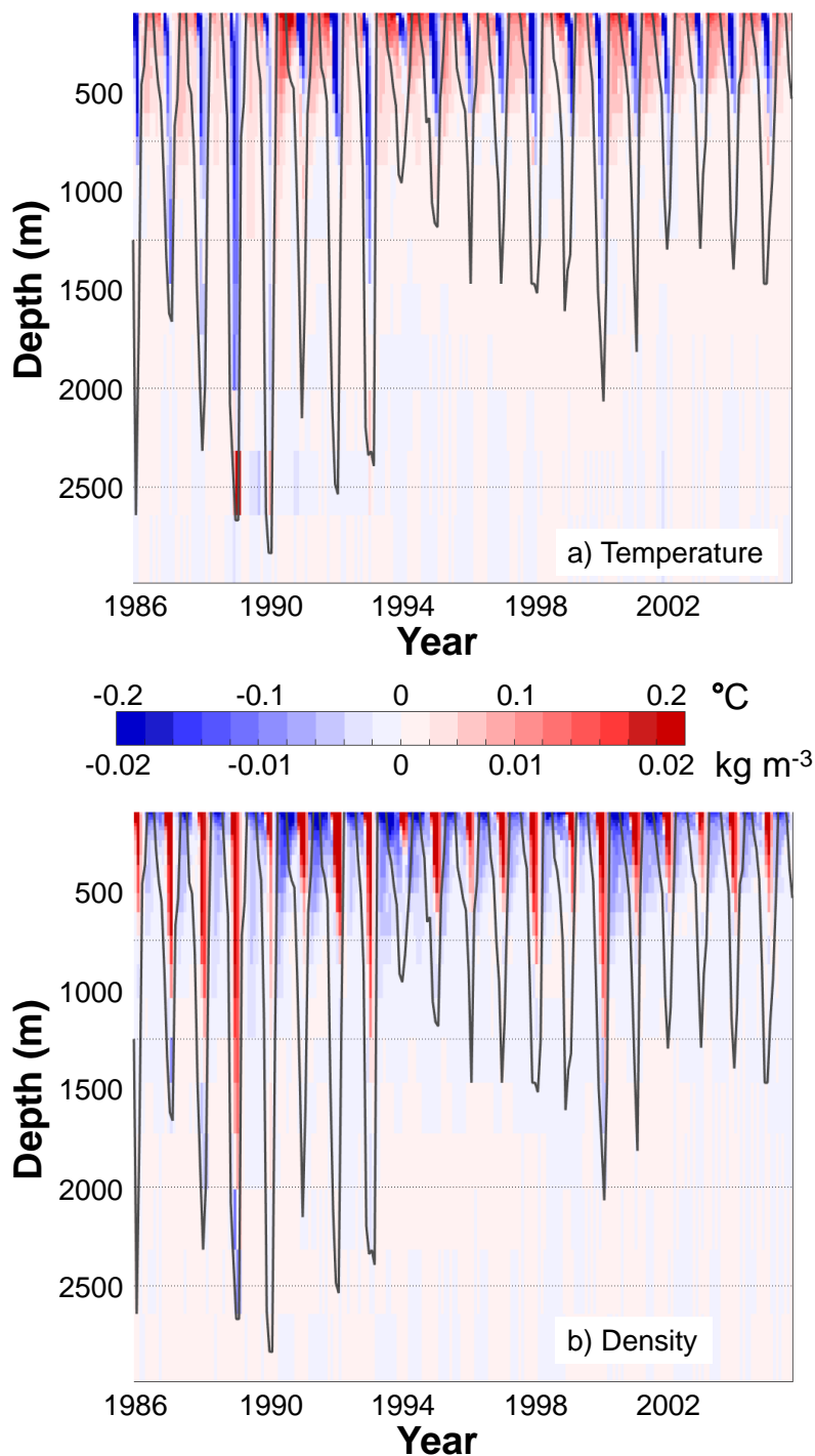
Figure 4. For only one model, CanESM2, Hovmöller diagram showing the difference from one month to the next of the temperature (top) and density (bottom) profiles with depth in the subpolar gyre. Dark grey line represents the SG mixed layer depth. Black dotted vertical lines highlight the depth levels representative of NADW: 750, 1250, 2000 and 2500 m.
