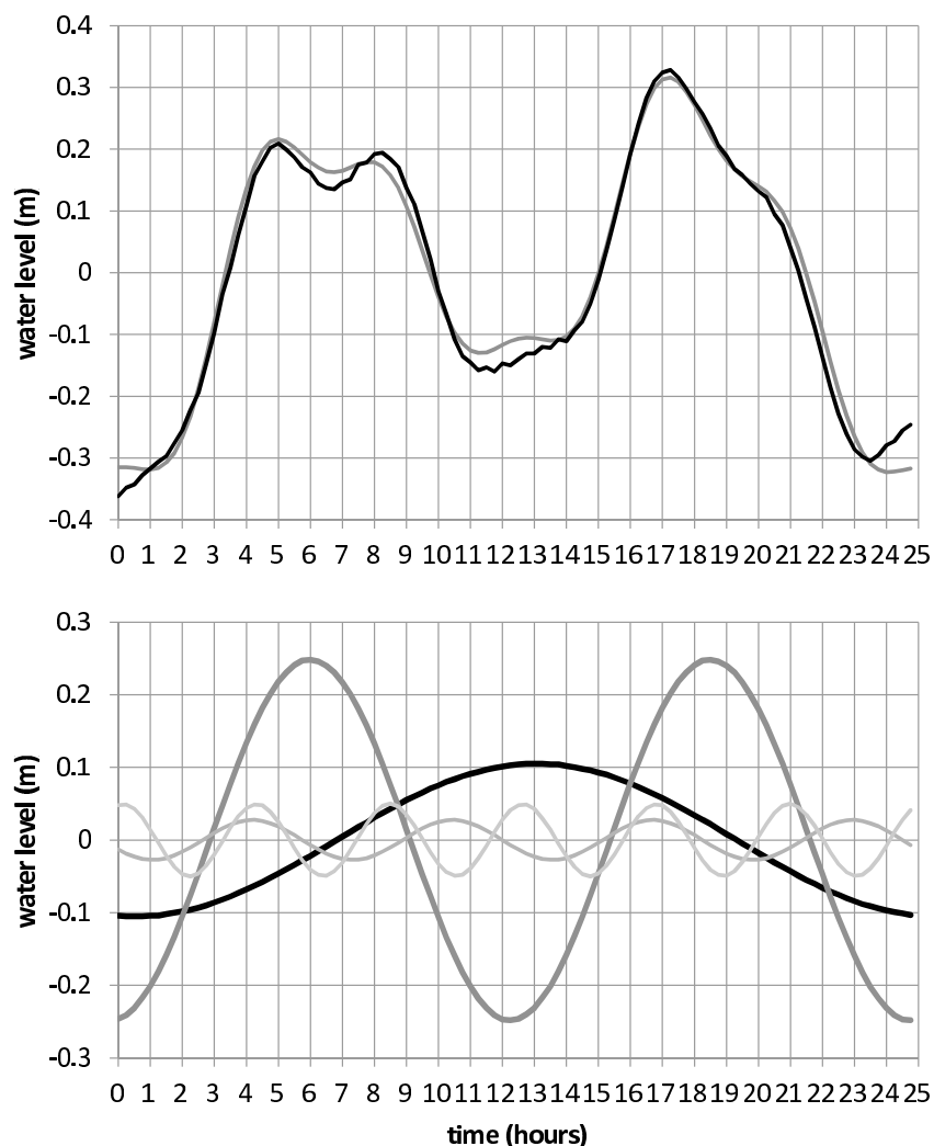
Figure 5. a) Observed and fitted tidal curves for 19th February. The double high water on the morning is reproduced by the fitted curve. b) D1, D2, D4, and D6 harmonics for 19th February (note that the higher the harmonic, the lighter the line colour). The high tide in D1 (black line) occurs in the middle of the day and causes the diurnal inequality seen in Fig. 3a. The D6 harmonic (lightest grey) has a larger amplitude than D4 and the minimum in D6 occurs closer to the high D2 than does the minimum in D4. It is the D6 harmonic that is primarily responsible for the double high water at Port Ellen.
