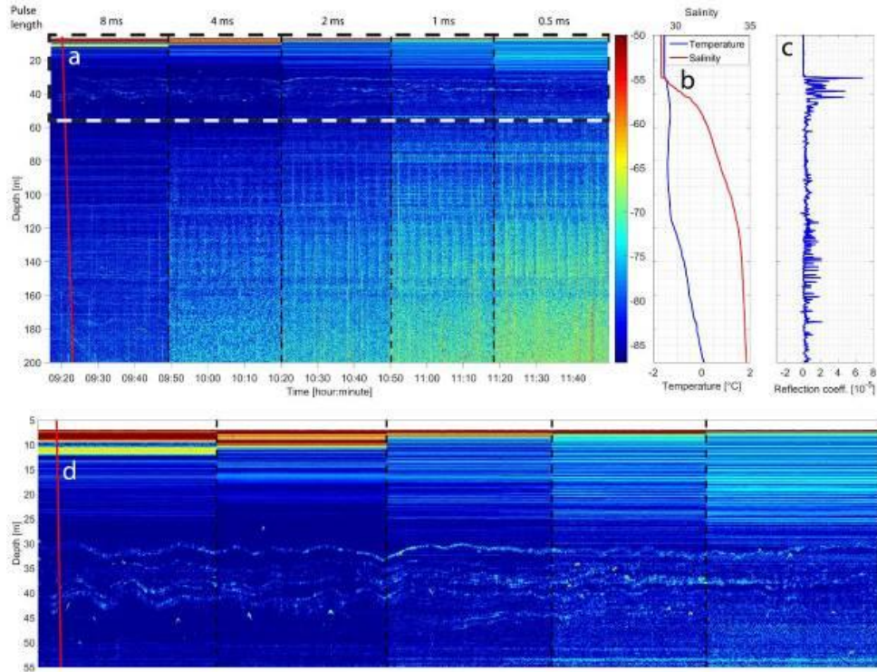
5 Figure 4. Comparison of EK80 data with different pulse lengths. (a) EK80 echogram. (b) CTD profiles showing temperature (blue) and salinity (red). (c) Reflection coefficients derived from CTD data. (d) Enlargement of dashed box in a. In a and d, the vertical red line is the CTD position and the vertical dashed black lines indicate changes in pulse length (decreasing from 8 ms to 0.5 ms).
