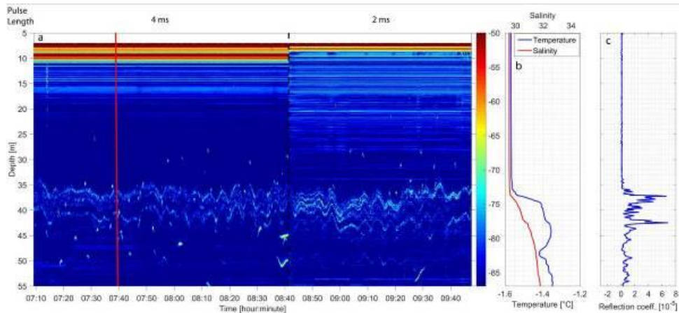
10 Figure 5. Tendancy of increased range resolution in EK80 data with smaller pulse length. (a) EK80 echogram with backscatter strength in dB on the color bar. (b) CTD profiles showing temperature (blue) and salinity (red). (c) Reflection coefficients derived from CTD data. Note that, as there is no ground truth CTD cast within the later section of the echogram, there might be splitting/merging of layers (as shown in Stranne et al., 2017) and other changes in the stratification behavior occurring near the change in pulse length.
