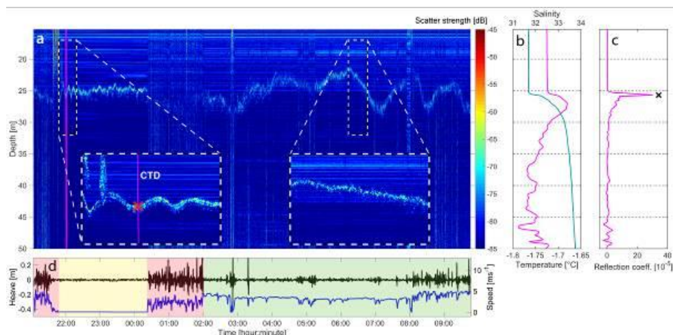
Figure 2. Continuous tracking of MLD in central Arctic Ocean over a 117 km cruise track. (a) EK80 echogram (2 ms pulse length) with magnified insets (dashed boxes) showing the MLD while drifting (left) and while steaming (right). (b) CTD profiles showing temperature (magenta) and salinity (cyan). (c) reflection coefficients derived from CTD data (magenta) and from scatter strength (black cross represents the observed scatter strength of -65 dB at this depth extracted from the left inset in a). (d) heave (black), speed over ground (blue), and time periods corresponding to ice breaking (red), steaming (green), and drifting (yellow). Vertical magenta lines in a show the position of the CTD. The red cross in a (left inset) marks the depth of the reflection coefficient spike in c. Note that the ability to detect MLD acoustically is severely reduced while breaking ice.
