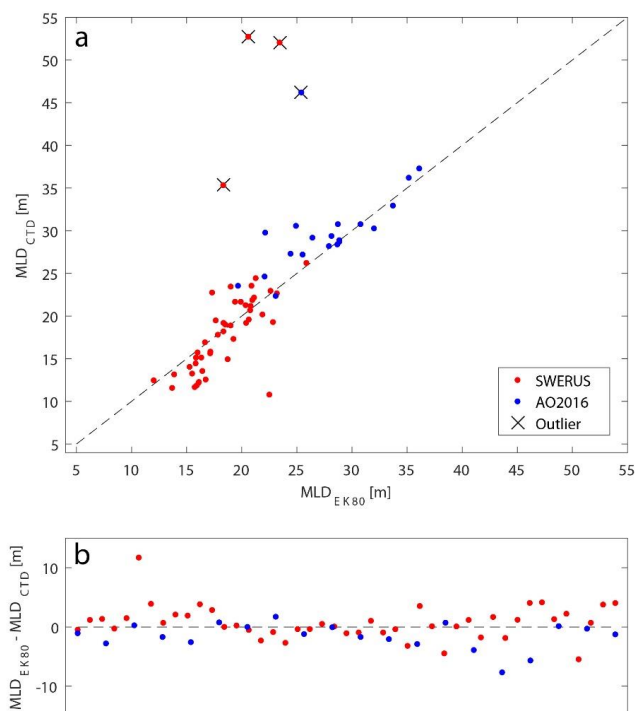
Figure 3. (a) MLD for the individual stations derived from CTD ( MLD_{CTD} ) versus MLD derived from EK80 data ( MLD_{EK80} ). (b) Difference between MLD_{EK80} and MLD_{CTD} . In total, four outliers (black crosses in (a)) where the \Delta T threshold method fails (as exemplified in Figure S2) are excluded from the statistics. Note that the original \Delta T threshold ( 0.2\text{ }^{\circ}\text{C} ) as presented in de Boyer Montégut et al. (2004) generally failed in the central Arctic Ocean (Figure S3) and that we instead used a modified \Delta T threshold of 0.05\text{ }^{\circ}\text{C} on CTD data from AO2016.
