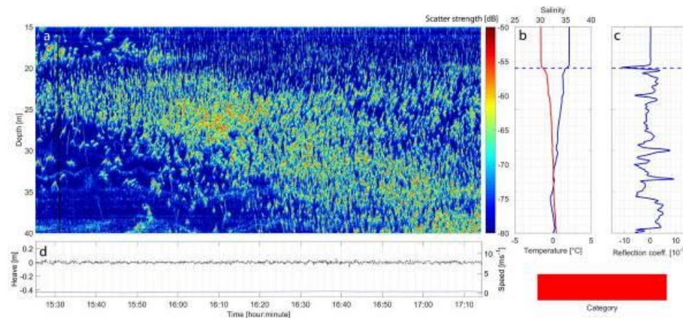
10 Figure 6. MLD obscured by biological scatter. (a) EK80 echogram with black vertical line indicating the position of the CTD rosette. (b) CTD profiles showing temperature (blue) and salinity (red). (c) Reflection coefficients derived from 15 CTD data. The horizontal dashed line in b and c show the MLD as defined by the \Delta T threshold method. Also shown at the lower right is the category (red) of this particular CTD station, indicating failure of the acoustic method to detect the MLD amidst strong biological scattering that spans across the MLD.
