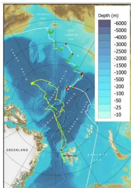
Figure 1. Map showing cruise tracks for the SWERUS-C3 cruise (white) and the Arctic Ocean 2016 cruise (yellow). CTD stations are shown as dots where green indicates the MLD was successfully observed acoustically, red indicates the MLD was not successfully observed acoustically, and blue indicates no mixed layer was present.
