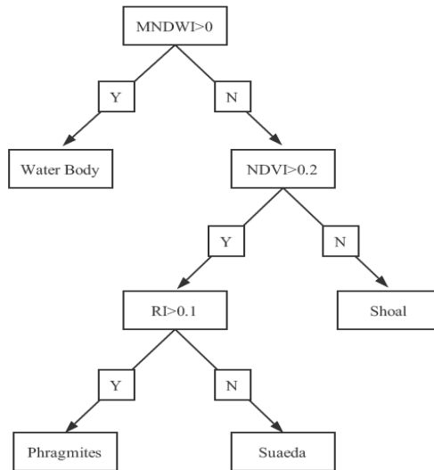
Figure 10. Vegetation classification based on decision tree
