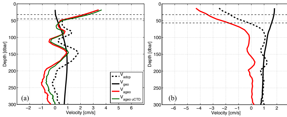
5 | Figure 3: Section-averaged cross-track velocity profiles at (a) 14.5° N and (b) 11° S. In (a), the solid red curve and the solid black 10 | curve is the ageostrophic and geostrophic velocity calculated from the CTD data, respectively. The dark green curve is the ageostrophic velocity based only on the uCTD data. In (b), the solid red curve and solid black curve is the ageostrophic and geostrophic velocity calculated from the combination of the CTD/uCTD data, respectively. The dashed black curve is the ADCP velocity. The upper horizontal dashed line denotes the basin-wide averaged MLD and the lower denotes the basin-wide averaged TTP depth.
