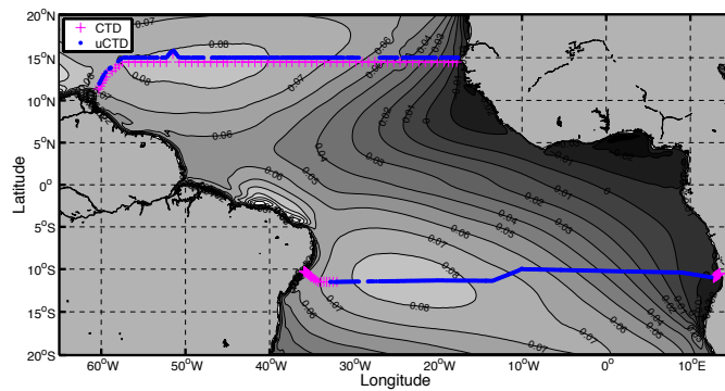
Figure 1: Positions of the CTD (magenta +) and uCTD (blue dots) measurement along 14.5° N and 11° S section. The 14.5° N section was completed during RV Meteor cruises M96 (April 28 to May 20, 2013, west of 20° W) and M97 (June 08 to June 09, 2013, east of 20° W), the 11° S section during M98 (July 06 to July 23, 2013). Note that the uCTD position for 14.5° N section is artificially shifted to the north by 0.5° for visual clarity. The grey shading with contours is the mean zonal wind stress calculated from NCEP/CFSr monthly wind stress between 1979 and 2011 in N m -2 .
